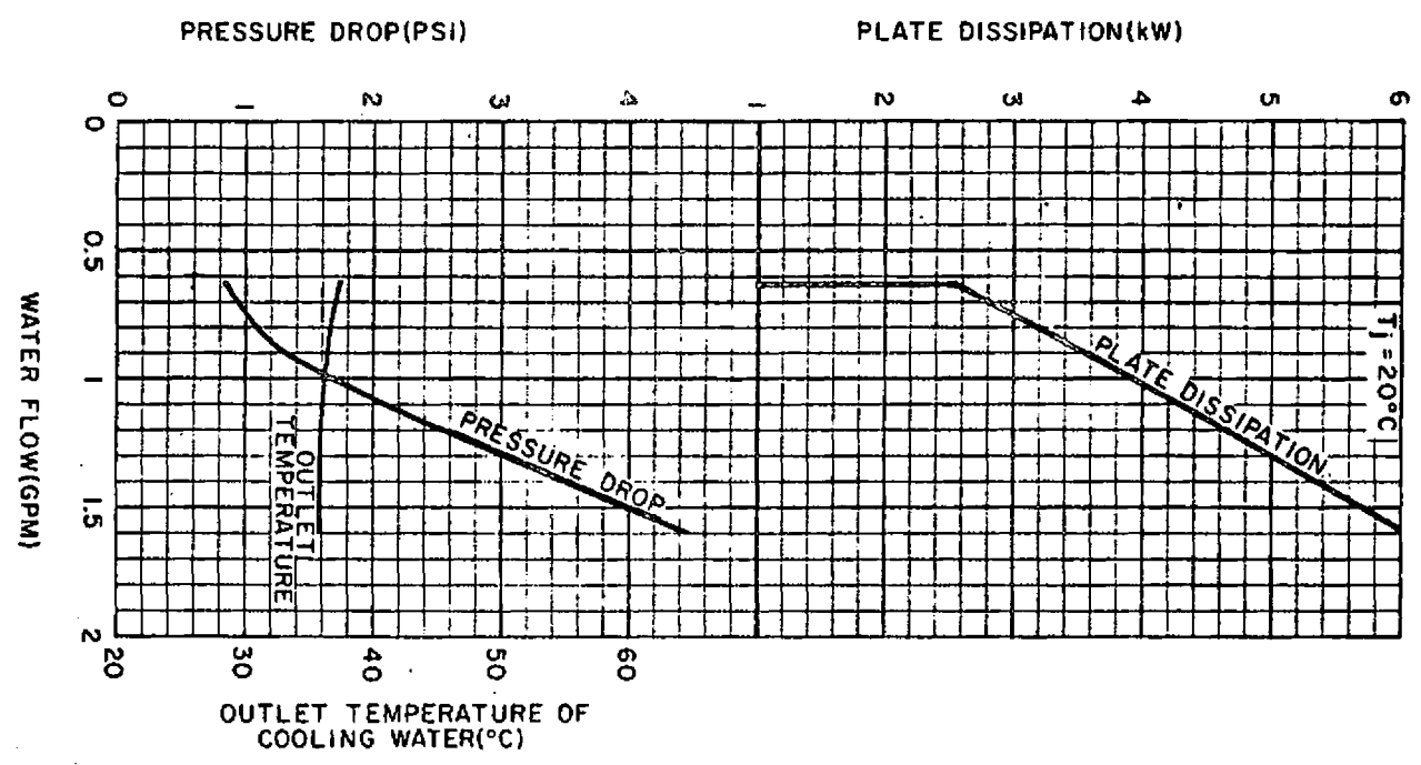
COOLING CHARACTERISTICS
