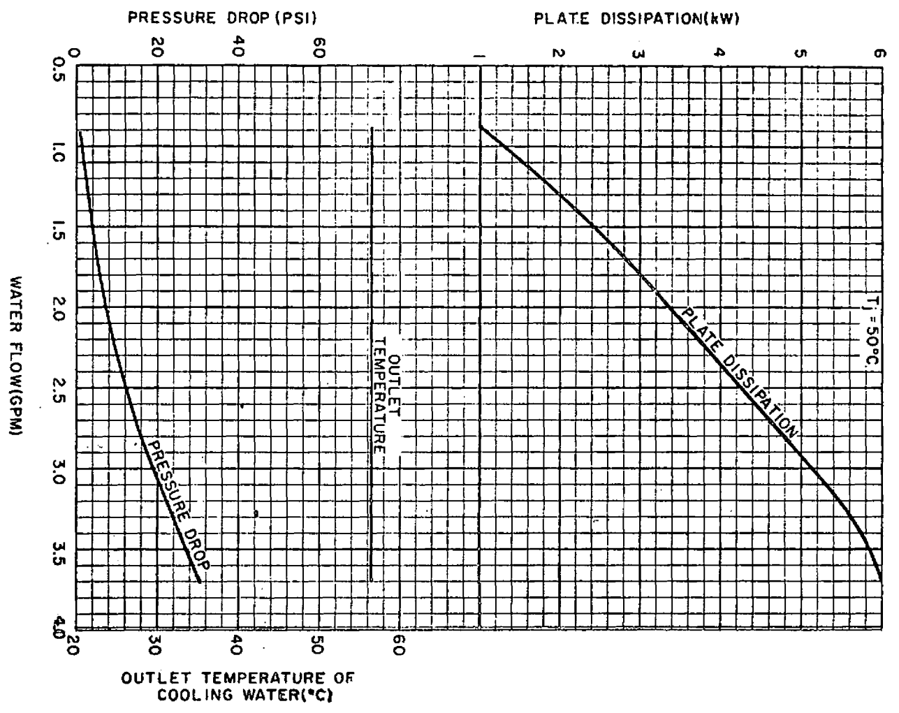
COOLING CHARACTERISTICS
