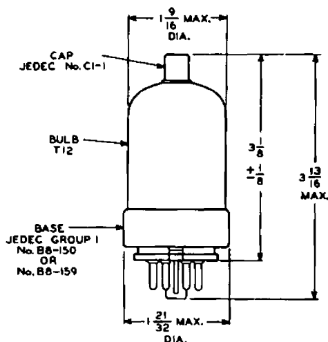
DIMENSIONAL OUTLINE
