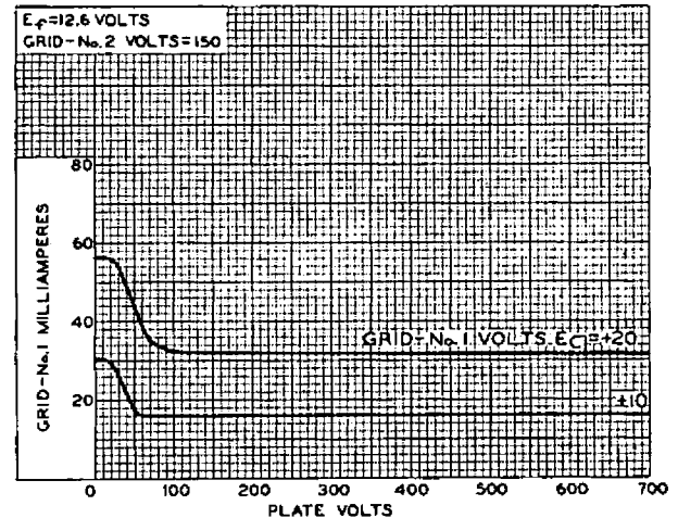
TYPICAL CHARACTERISTICS
