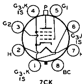
TERMINAL CONNECTIONS
