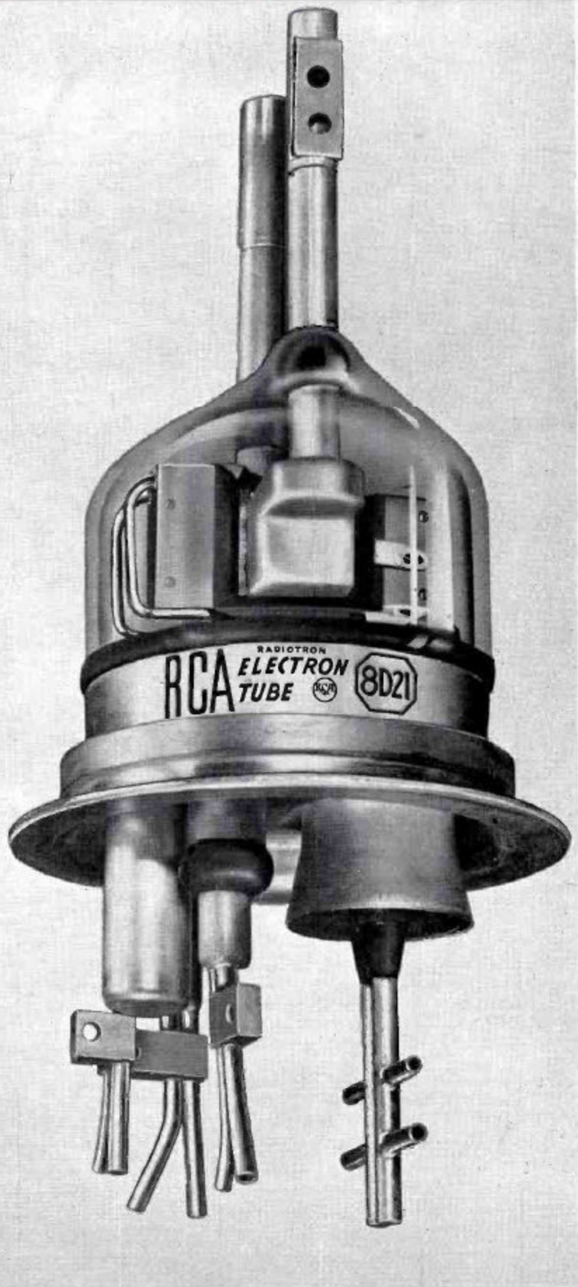
FIG. 2. Finished 8D21 showing how the anode-dome assembly (with anode terminals of tetrodes No. 1 and No. 2 projecting from top) is welded to metal header which supports the internal structure of tube. Directly below metal header and to the right are the control-grid terminals of tetrodes No. 1 and No. 2. To left of center, the terminal for the No. 2 grids; and to the extreme left, the filament terminals. The tube is fitted with a special cathode and beam-confining electrodes, and, because of the cathode structure used, must be operated in a horizontal position with plane of the control grids below horizontal plane of the filament leads.
