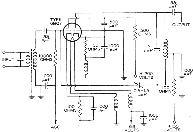
Fig. 11—Driven-grounded-grid circuit.
