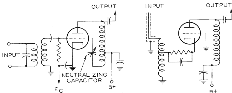
Fig. 1a—Grounded-cathode circuit. Fig. 1b—Grounded-grid circuit.
