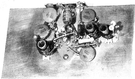
Fig. 5—Layout for direct-coupled driven-grounded-grid circuit using 6BQ7.
