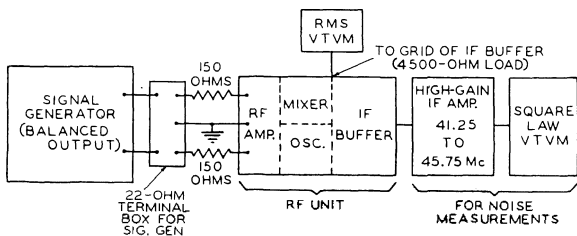
Fig. 9—Block diagram of test set-up.
