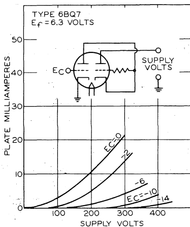
Fig. 7b—Average plate characteristics, series-connected.
