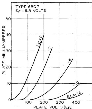
Fig. 7a—Average plate characteristics of each unit.
