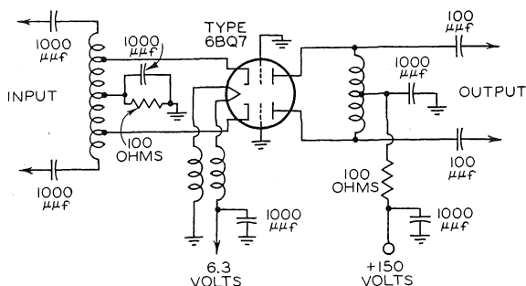
Fig. 10 — Push-pull grounded-grid circuit.
