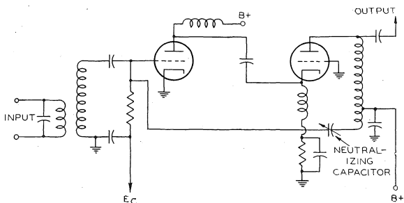
Fig. 3—Driven-grounded-grid circuit.
