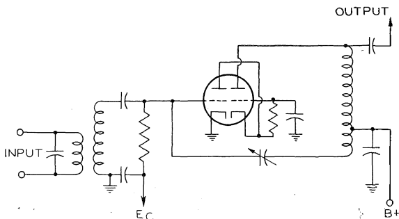
Fig. 4—Direct-coupled driven-grounded-grid circuit.
