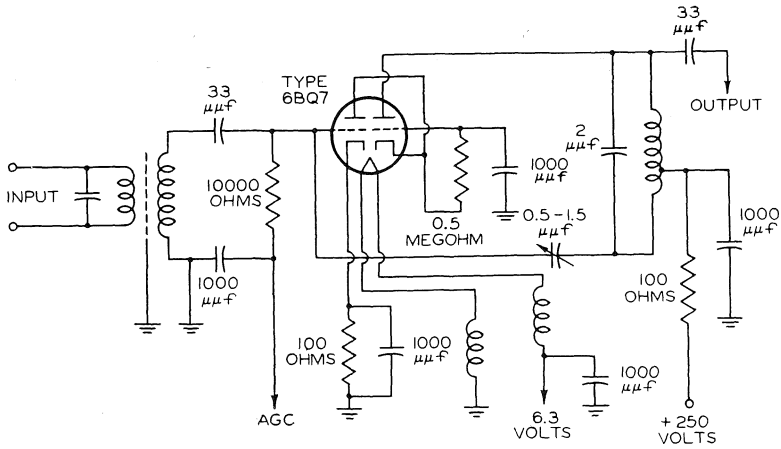
Fig. 12a—Direct-coupled driven-grounded-grid circuit.
