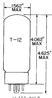
GLASS BULB SHORT MEDIUM-SHELL 5 PIN OCTAL 88-110 OR 88-118 OUTLINE DRAWING JEDEC 12-16
