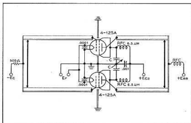
Screen-tuning neutralization circuit for use above 100 Mc. C is a small split-stator capacitor.
