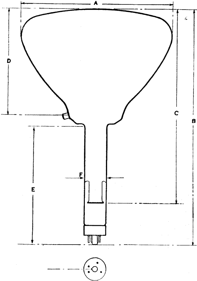
OUTLINE DRAWING OF CRM 71.
