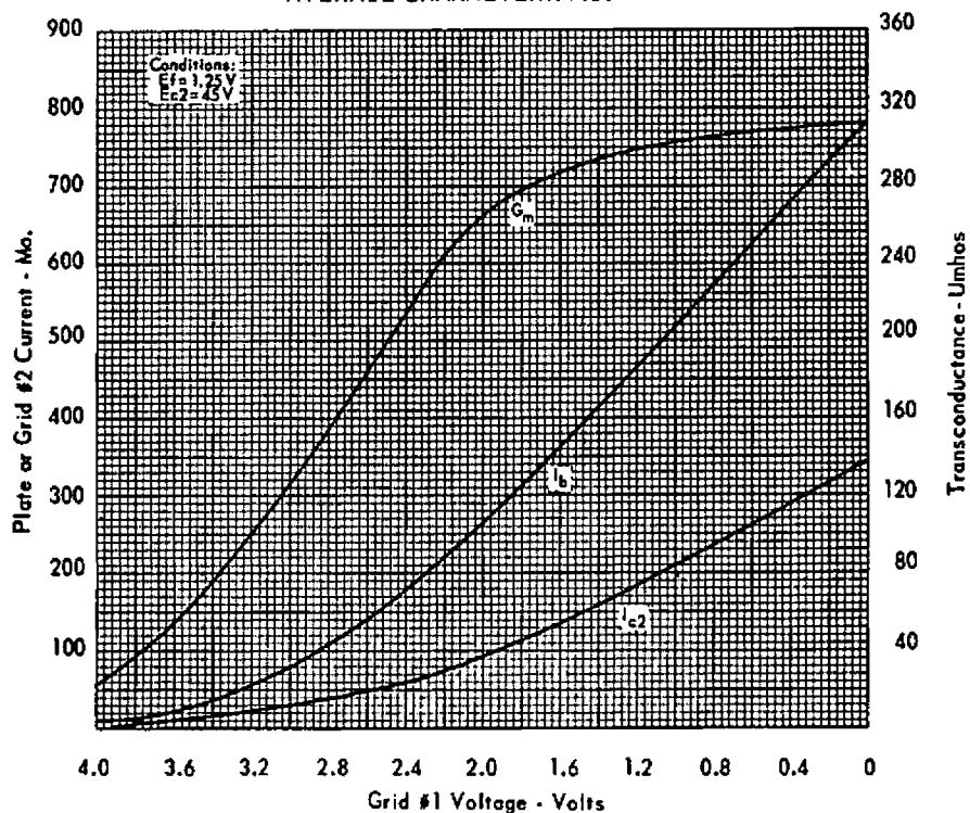
AVERAGE CHARACTERISTICS
