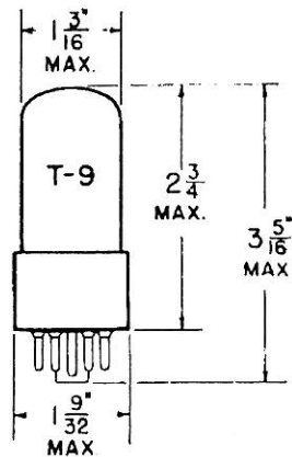
GLASS BULB
