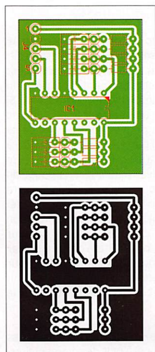
Figure 11A - Implantation composants encodeur. Figure 11B - CI encodeur.
