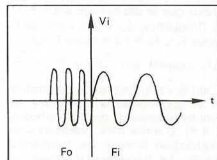
FIGURE 4: MODULATION FSK.
