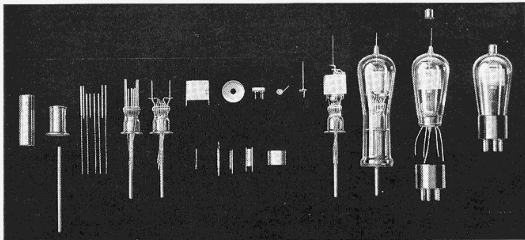
Parts Assembly of the '24-A
