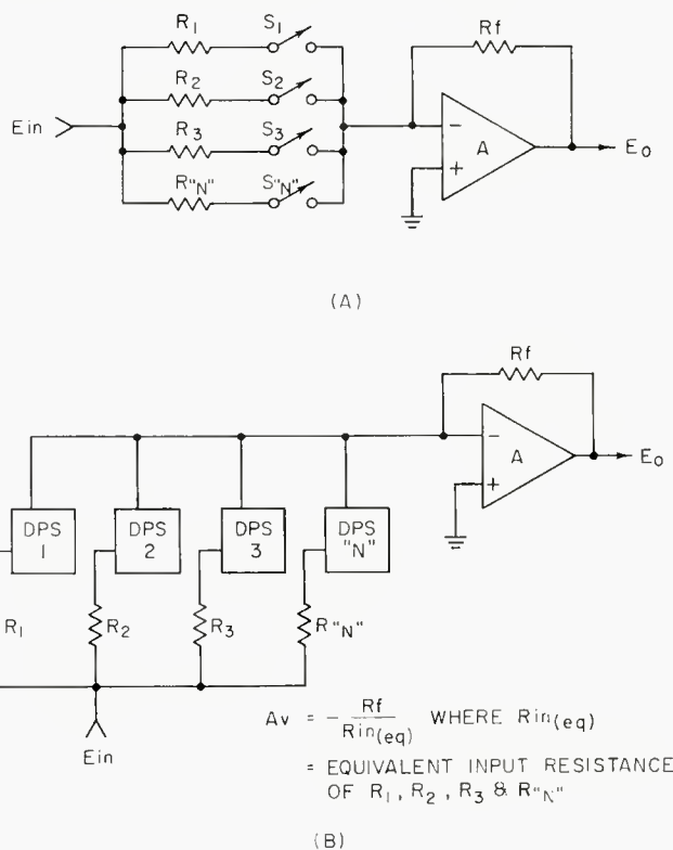
Figure 1. (A) is a programmable attenuator. (B) is the dps programmable attenuator.
