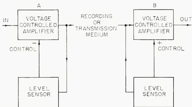
Figure 1. A linear compressor-expander system using voltage controlled amplifiers.
