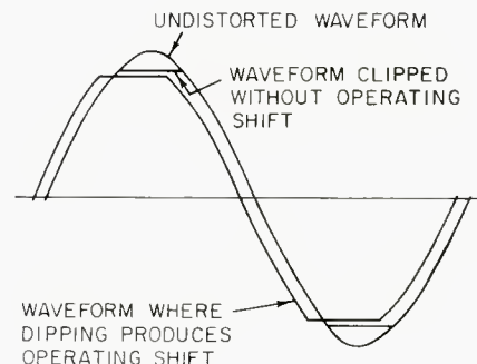
Figure 2. Some waveforms to show different possible effects of clipping, at the same nominal level (a slight difference in clipping level is shown, only to avoid confusion between the two shapes).
