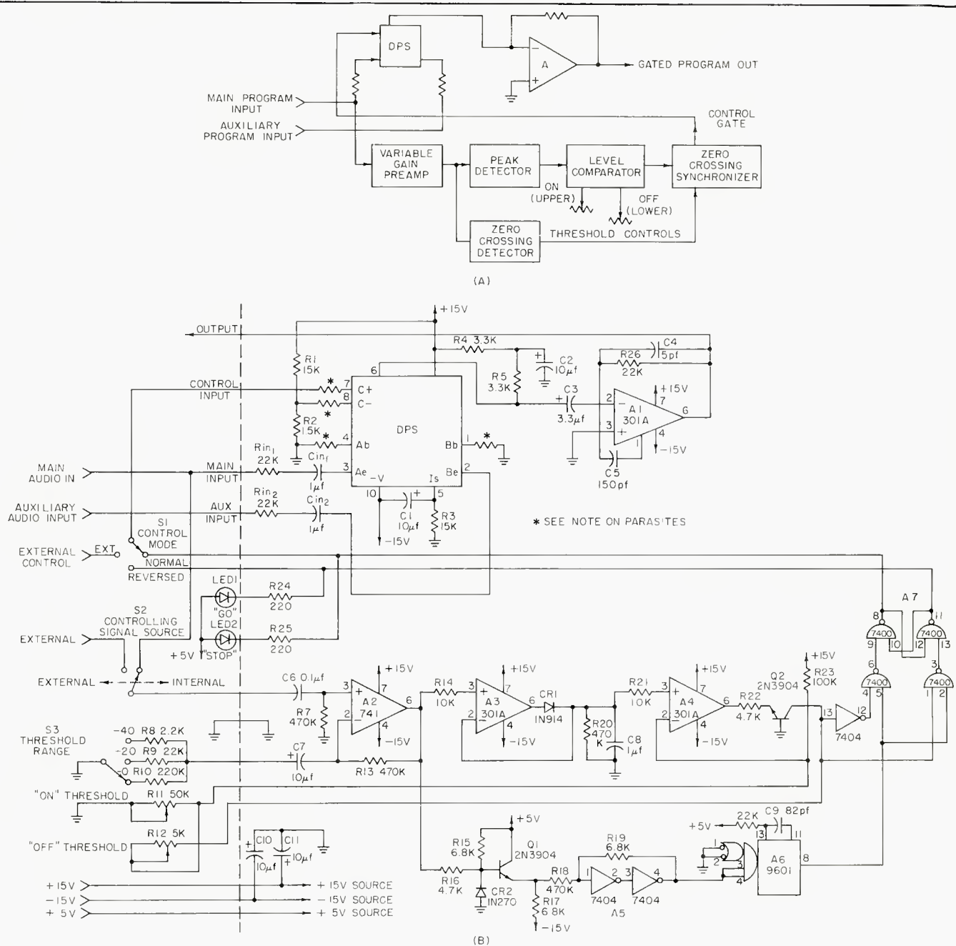
Figure 5. A level-controlled synchronous audio gating system. The level-controlled audio gate system shown in (A) and (B) is a good example of automated signal processing in a couple of senses. Basically, this current is a on-off switch using a dps. However the key to its versatility is in how it accomplishes the switching. This it does in quite a sophisticated manner.
