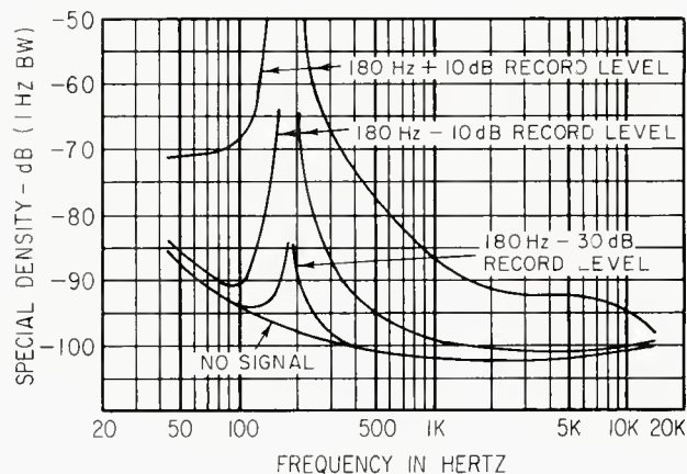
Figure 2. Noise in tape recording.
