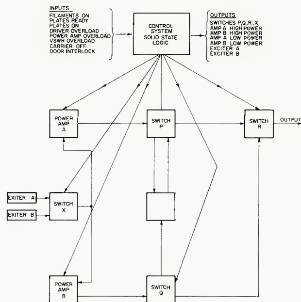
Figure 1. An automated transmitter switchover system.
