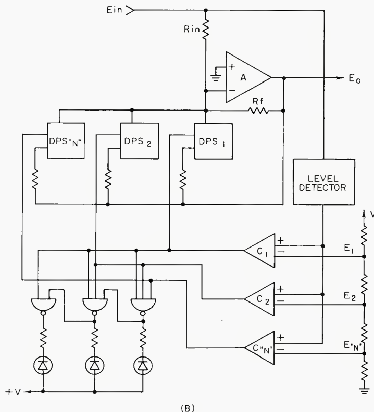
Figure 4. At (A) a programmable gain amplifier using dps elements in the feedback loop. At (B) is a distortionless agc system with led gain reduction readout.
