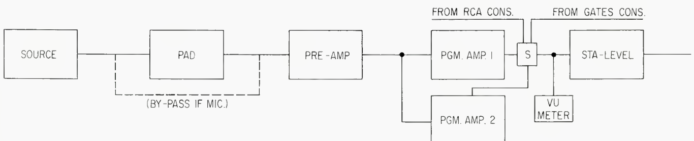
Figure 1. A block diagram of the Langevin console. The VU meter bridges (through a Langevin bridging card) the program line after the output selector switch (s) thereby tracking any source feeding the transmitter.
