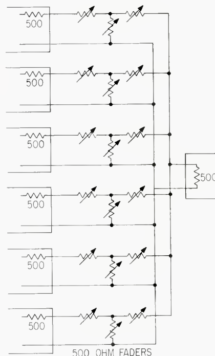
Figure 4. Using a 6-way mixer, fed from ideally-matched line amplifiers, and feeding into another, all of the impedances being 500 ohms.
