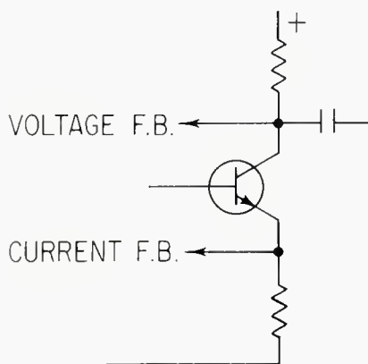
Figure 5. Different ways of using feedback for internal impedance control. To control output impedance, voltage or current feedback can be used to control input impedance, series or shunt injection can be used.
