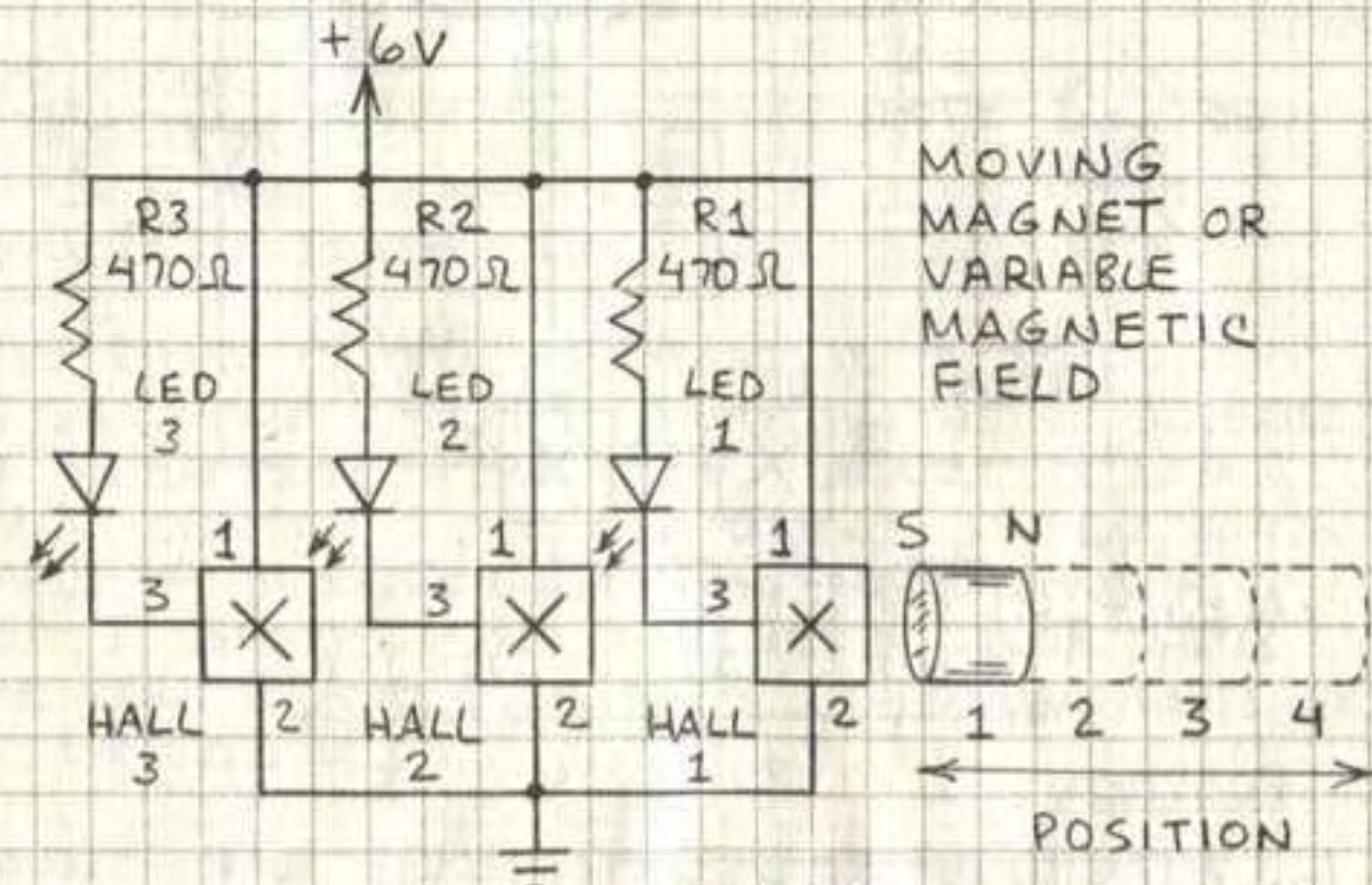
STACKED HALL SENSORS (A3141)
