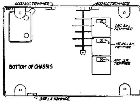
Fig. 2—Tube Arrangement & Location of Trimmers
