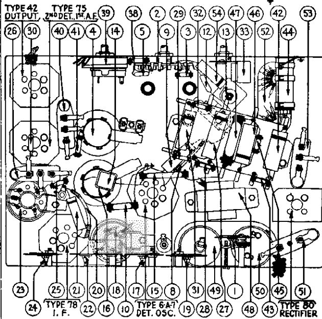
Fig. 4—Base View
