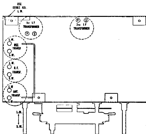
Figure E—Location of Line-Up Capacitors
