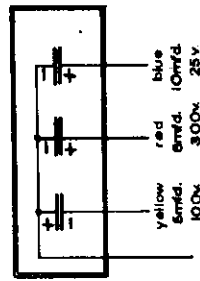
Detail of 4.681 Electrolytic Cond.
