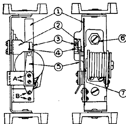
No. I No. II 1. Reed Assembly 4. Stop-Post 2. Stop Post mtg. block 5. Contact Spring Assm. 3. Stop Post locking-screw 6. Cam-nut adjustment 7. Air-gap
