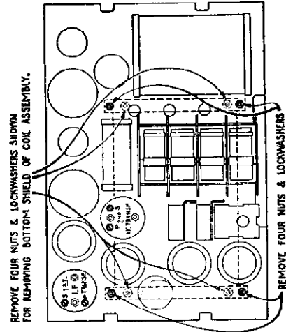
Figure D—Location of nuts and lockwashers holding coil assembly
