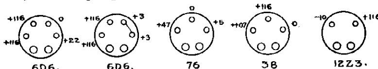
CHASSIS CM BOTTOM VIEW.
