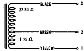
INTERNAL CONNECTIONS OF INPUT TRANSFORMER
