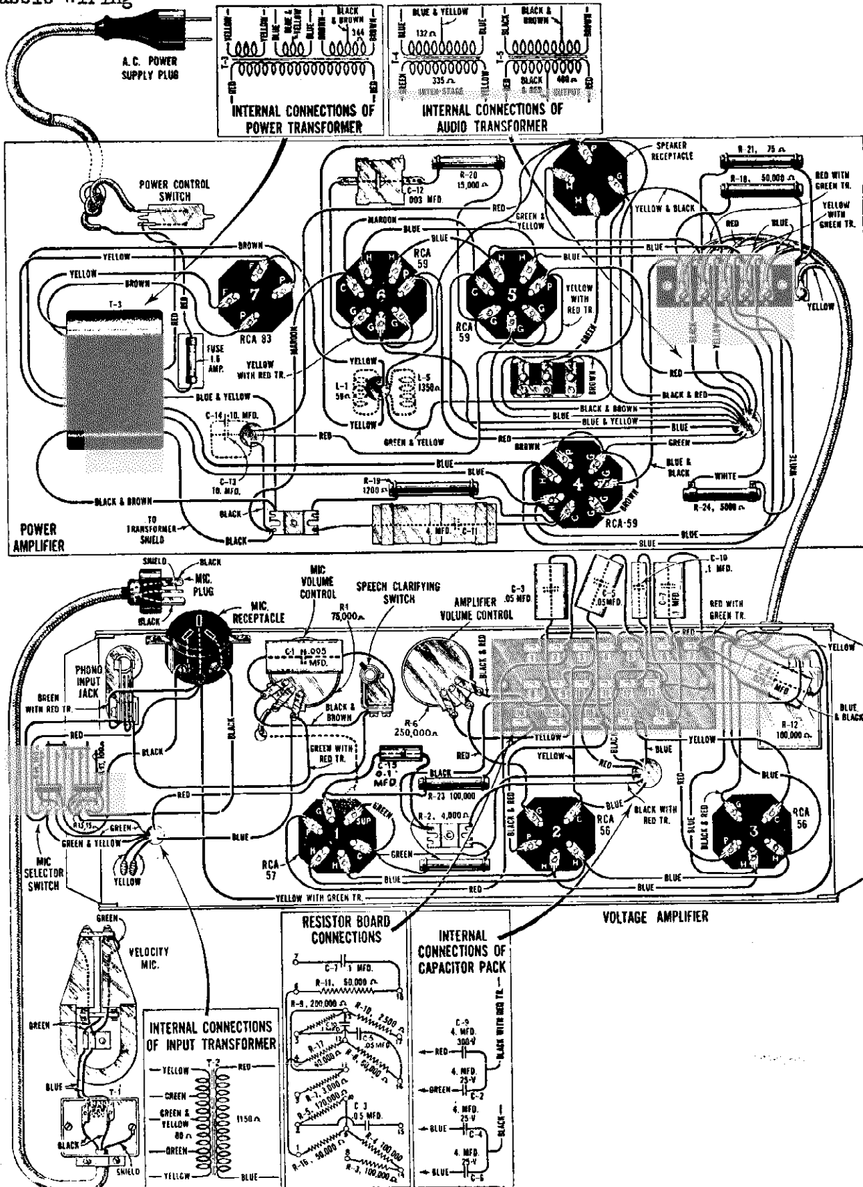
Figure 10—Wiring Diagram—Universal Amplifier
