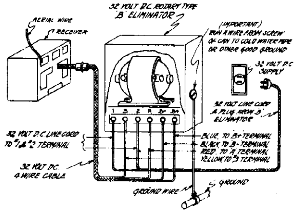
FIG. 3 SKETCH SHOWING CABLE CONNECTIONS TO B ELIMINATOR FOR 32 VOLT D.C. OPERATION
