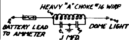
DIAGRAM #1
