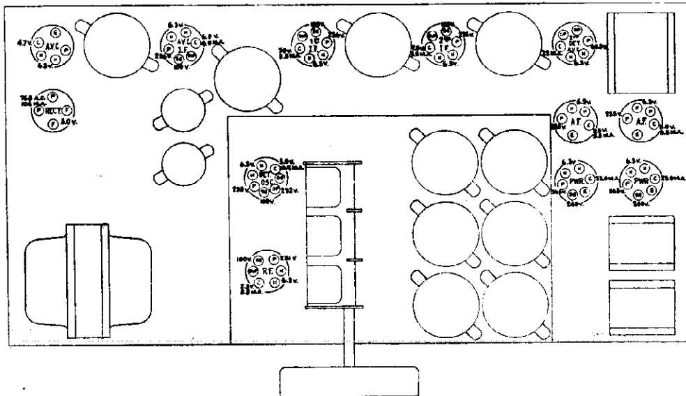
Figure 10—Radiotron Socket Voltages
