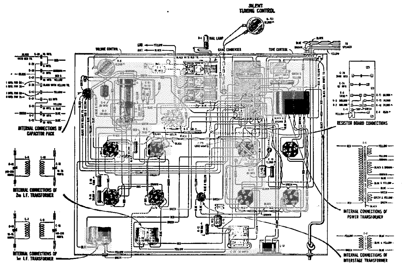
Figure 4—Chassis Wiring Diagram
