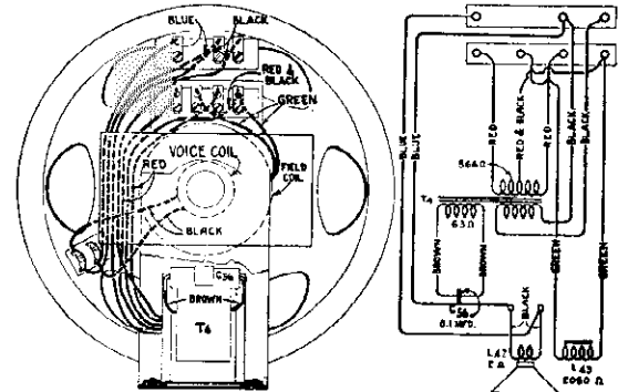
Figure 6—Loudspeaker Wiring
