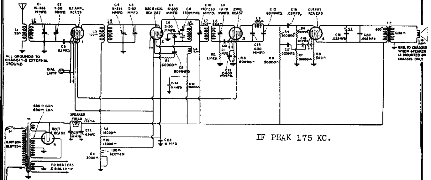
Figure 1—Schematic Circuit Diagram
