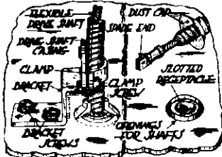
Fig. 6—Details of Flexible Shaft Attachment
