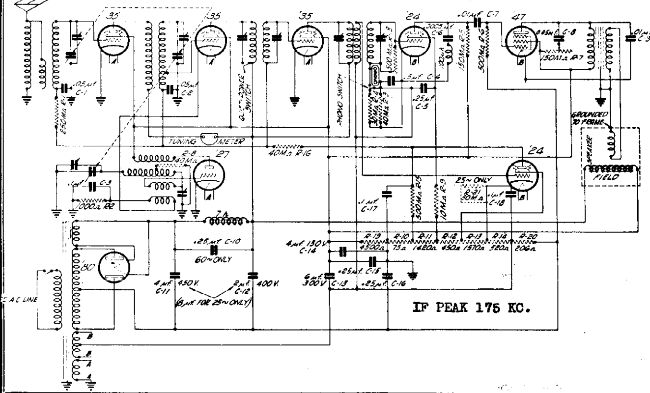
SCHEMATIC WIRING DIAGRAM SERIES 40-A 60 & 25 CYCLE
