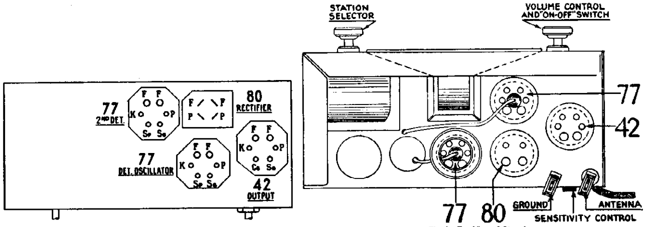
Fig. 1—Tube Socket Layout (Viewed from Bottom)
