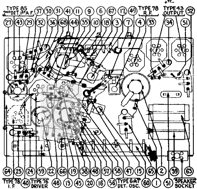
Fig. 4—Bottom View
