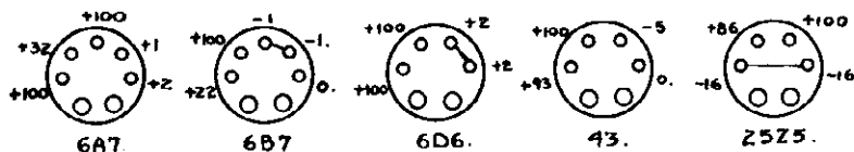
CHASSIS D & DSP BOTTOM VIEW.
