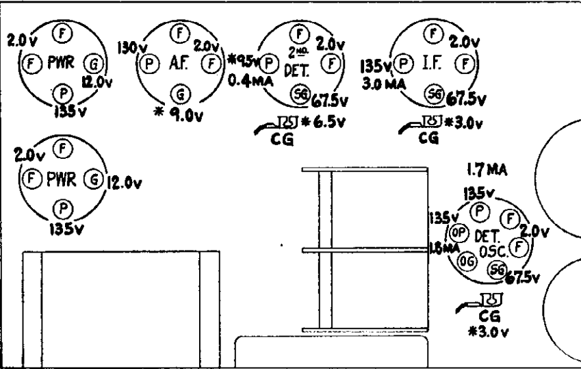
Figure 5—Socket Voltage Readings
