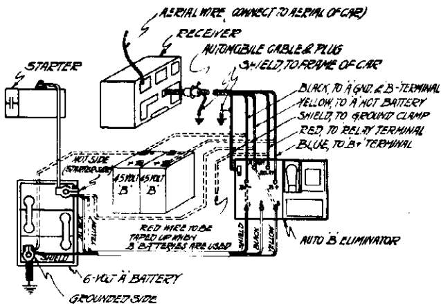
FIG. 2 SKETCH SHOWING CABLE CONNECTIONS TO B BATTERIES FOR 6 VOLT A AUTO OPERATION
