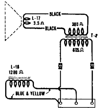
INTERNAL CONNECTIONS OF SPEAKER
