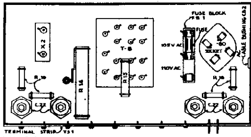
LINCOLN DE LUXE SW 33 - POWER PACK BOTTOM PLAN
