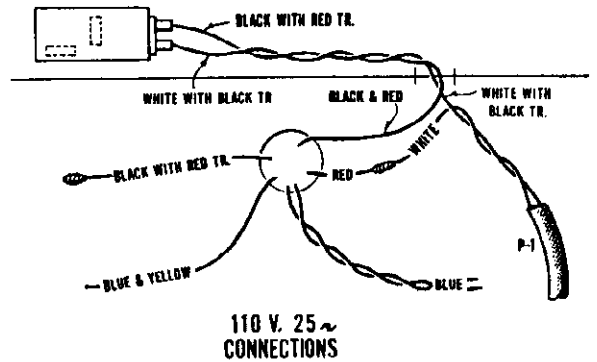
Figure I—100-115 Volt Connection of 25-60 Cycles Transformer
