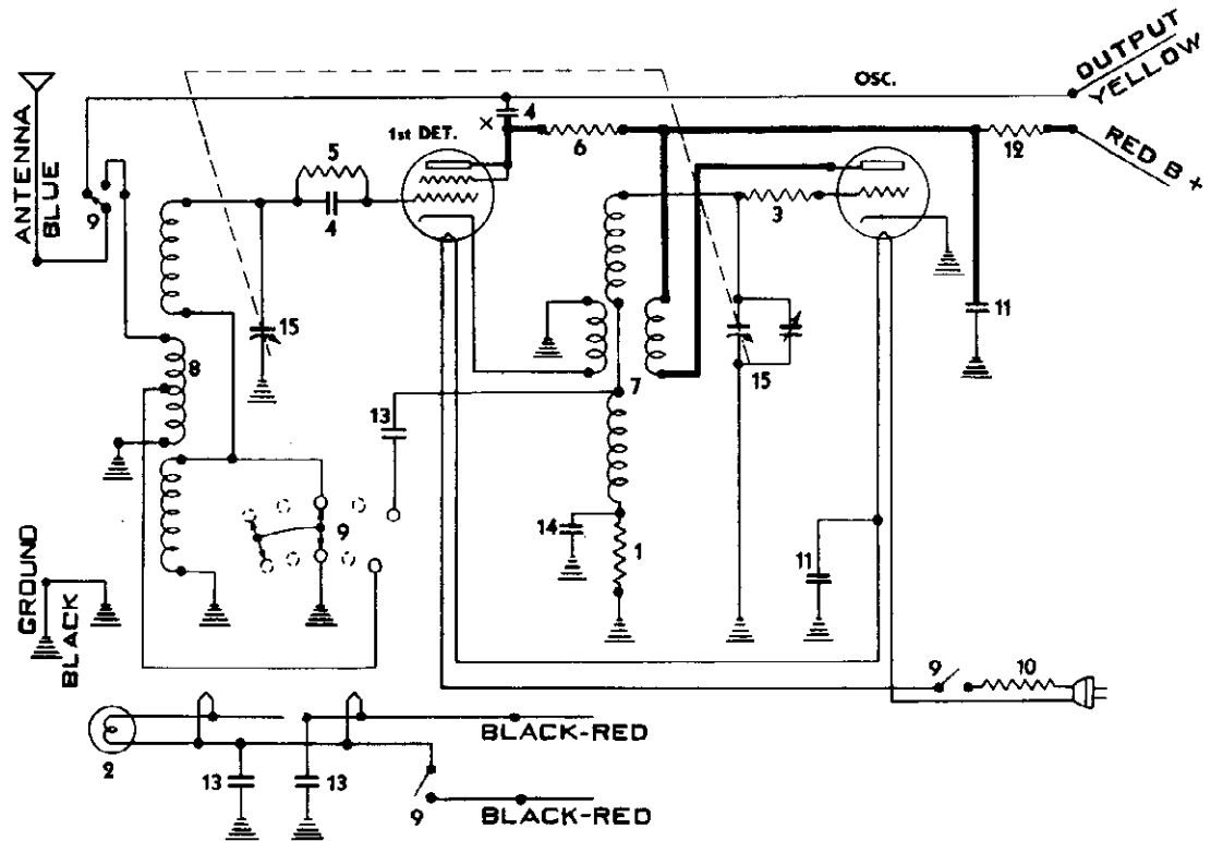
FILAMENT WIRING OF R-114
