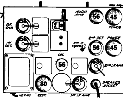
Fig. 2—Tube Arrangement
