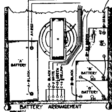
Tube Arrangement and Battery Connections
