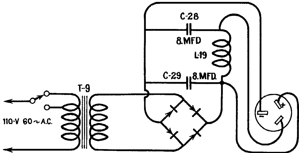
Schematic Wiring Diagram
