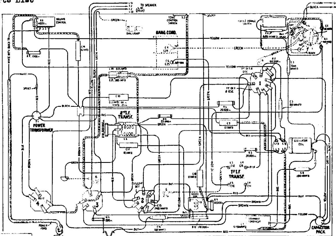
Figure B—Wiring Diagram
