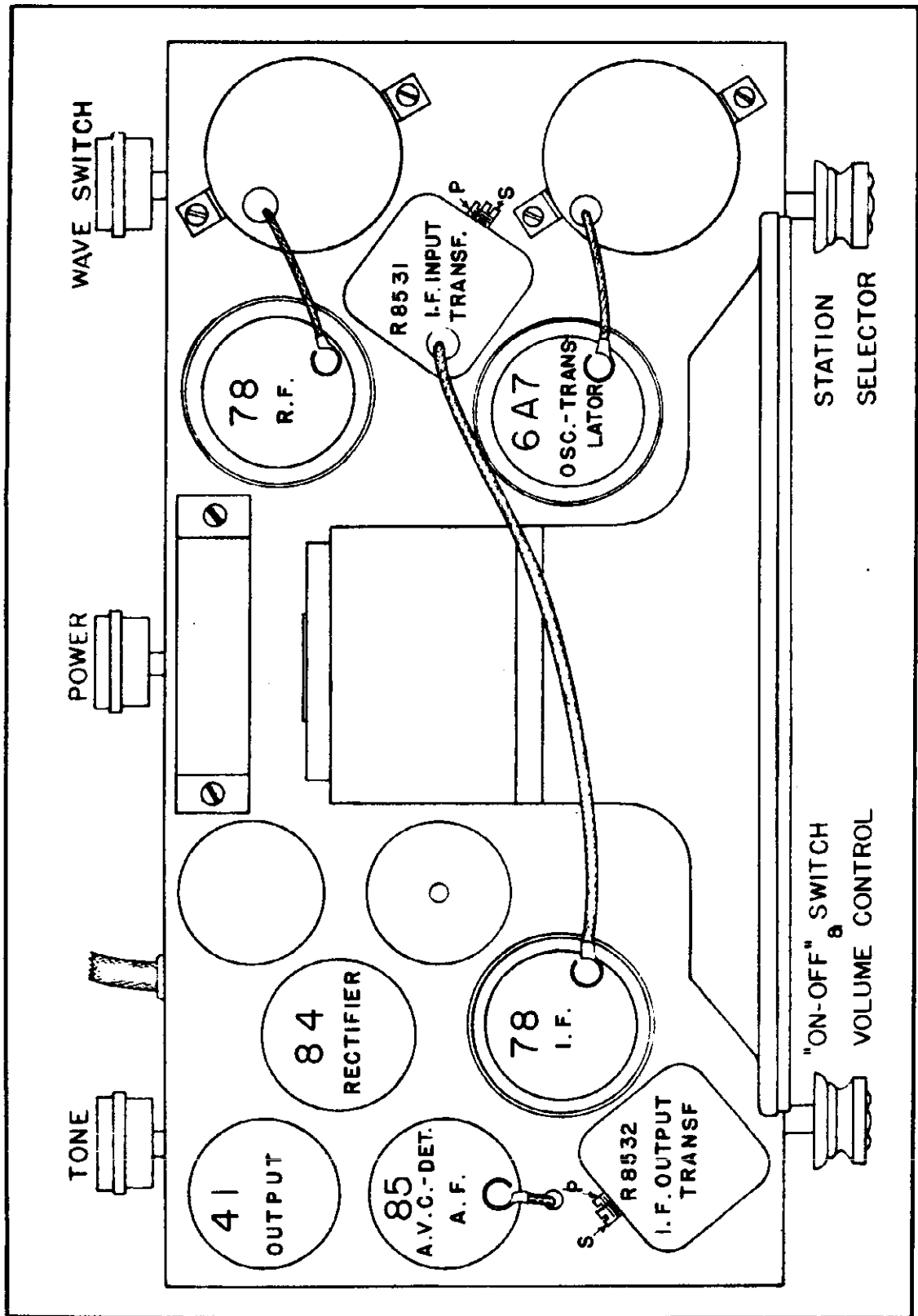
FIG. 50. SERVICE ILLUSTRATION - MODEL 400
