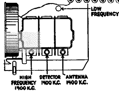
Fig. 5—Top View of Chassis showing Comp. Cond. mfd. on Tuning Condenser, Model 19, also Low Freq. Compensating Condenser.
