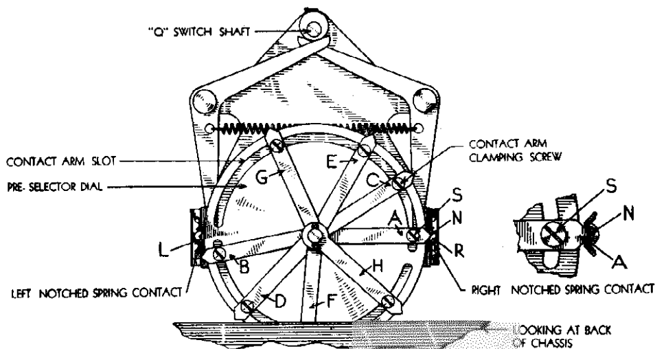
Fig. 2. Pre-selector Mechanism
