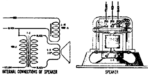
Figure C—Loudspeaker Wiring
