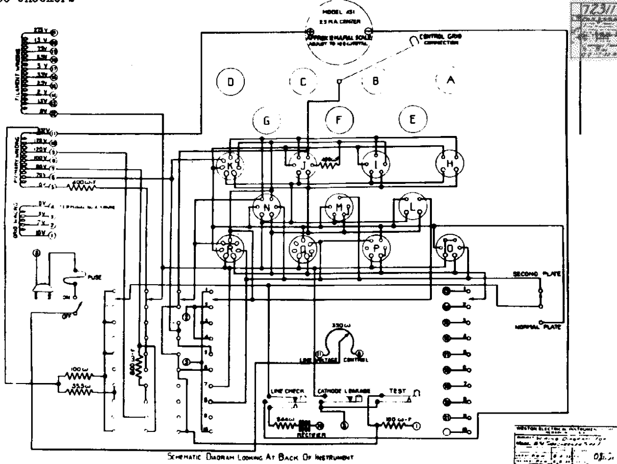
SCHEMATIC DIAGRAM LOOKING AT BACK OF INSTRUMENT
