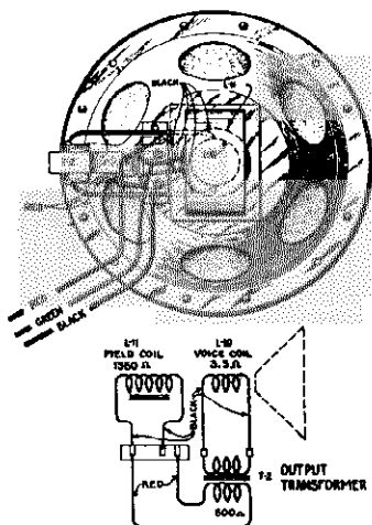
Figure C—Loudspeaker Wiring
