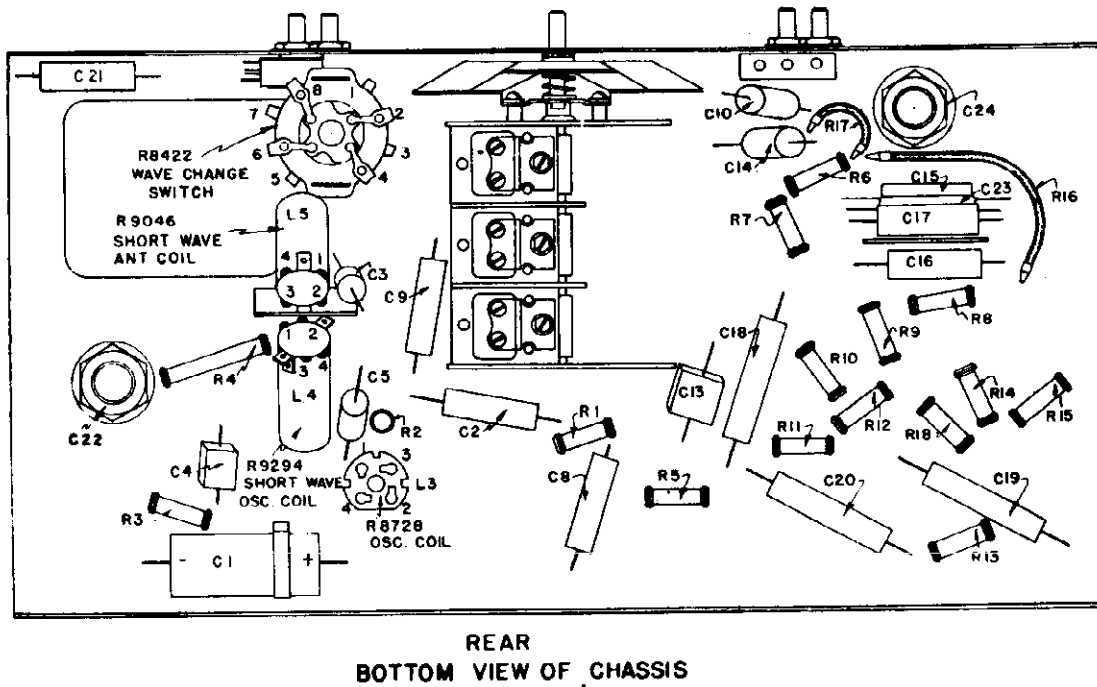
FIG. 70. SERVICE ILLUSTRATIONS - MODEL 601
