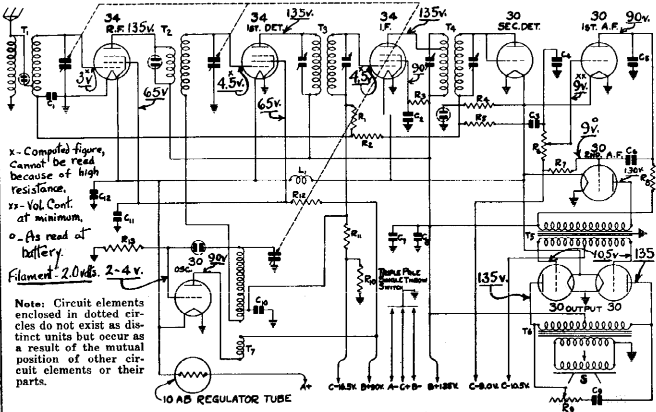
Fig. 2.—Tube Arrangement and Battery Connections
