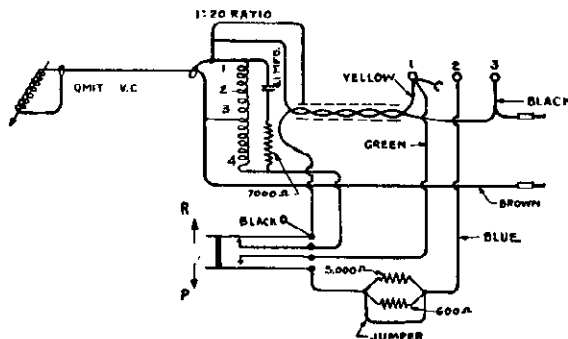
Figure H—End Table Connections
