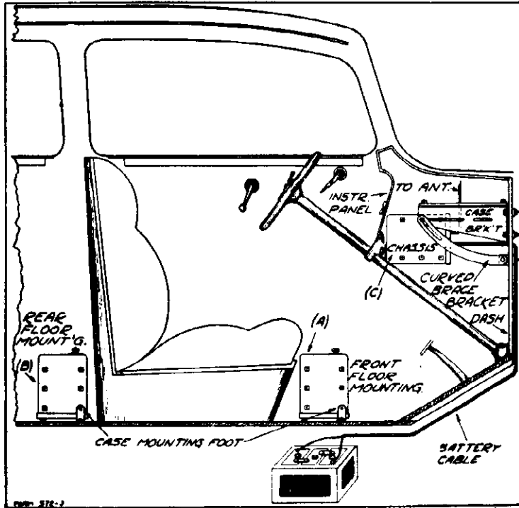
Fig. 1—Integral Mounting—Side View
