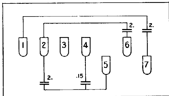
Model 77 Condenser Block Part No. 3870
