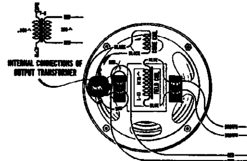
Figure A—Loudspeaker Wiring
