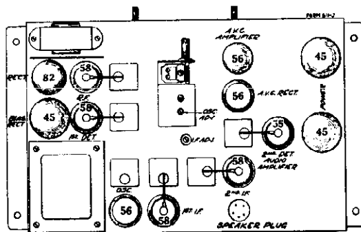
Tube Arrangement
