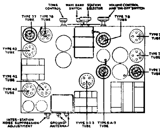
Fig. 1—Top View of Chassis, showing Tube Locations, and Major Parts
