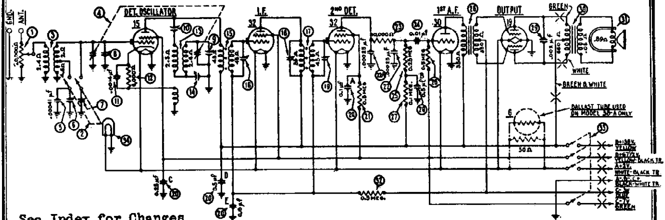
Fig. 3—Schematic Wiring Diagram
