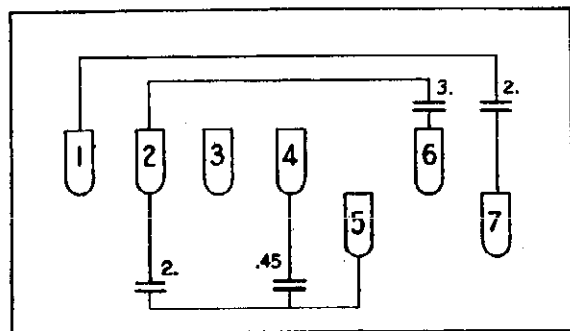
Model 77A Condenser Block Part No. 3871
