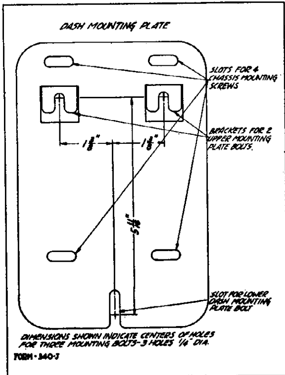
Fig. 5—Dash Mounting Plate
