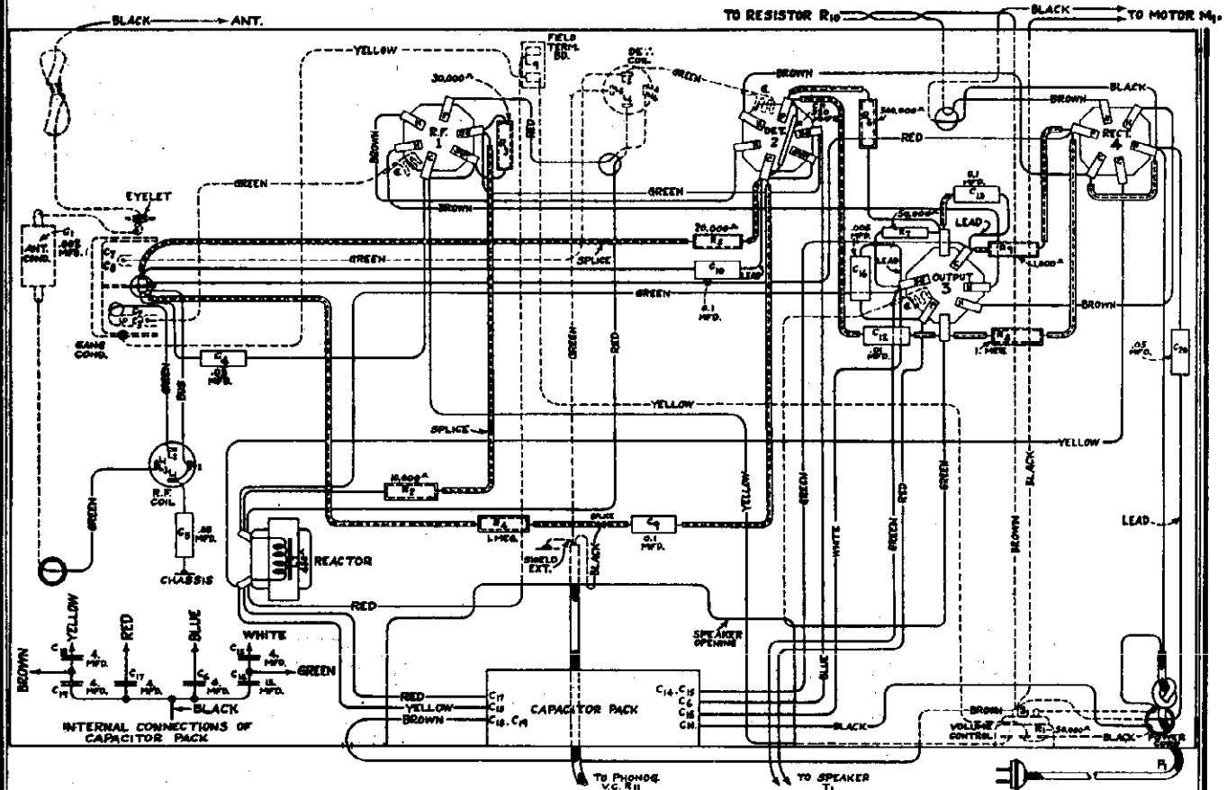
Figure D—Wiring Diagram
