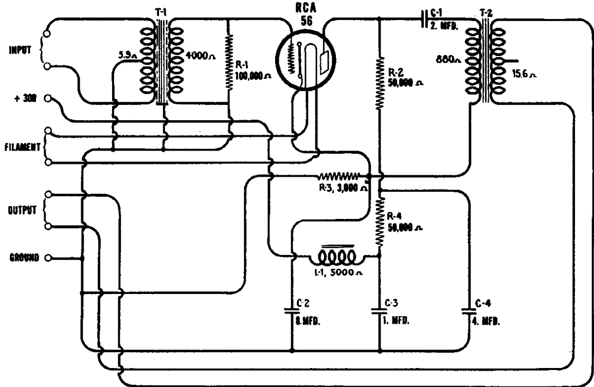
Schematic Wiring Diagram
