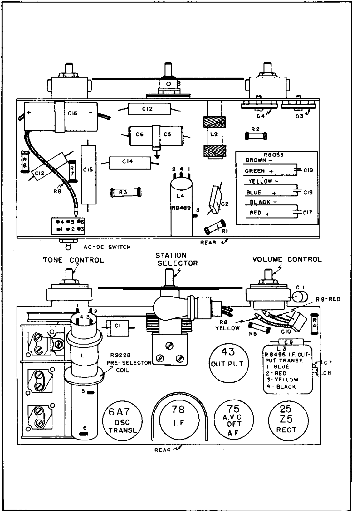
FIG. 63 - SERVICE ILLUSTRATIONS - MODEL 501
