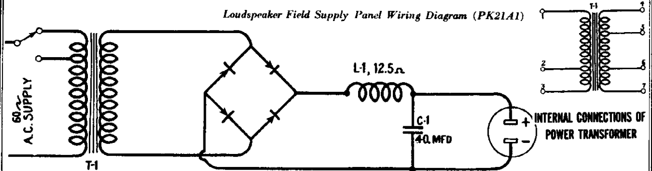
Schematic Wiring Diagram
