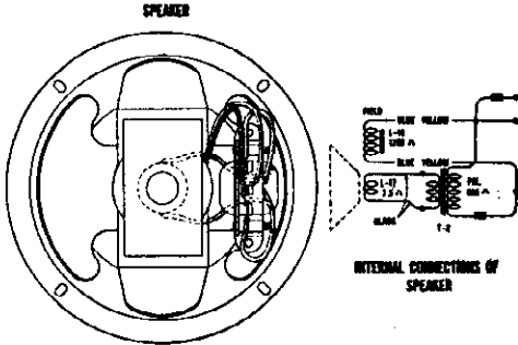
Figure C—Loudspeaker Wiring
