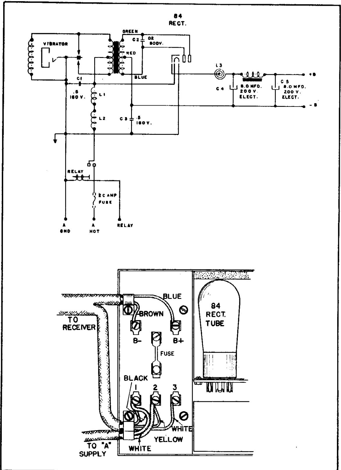
FIG. 56. SCHEMATIC - MODEL 106B POWER SUPPLY UNIT
