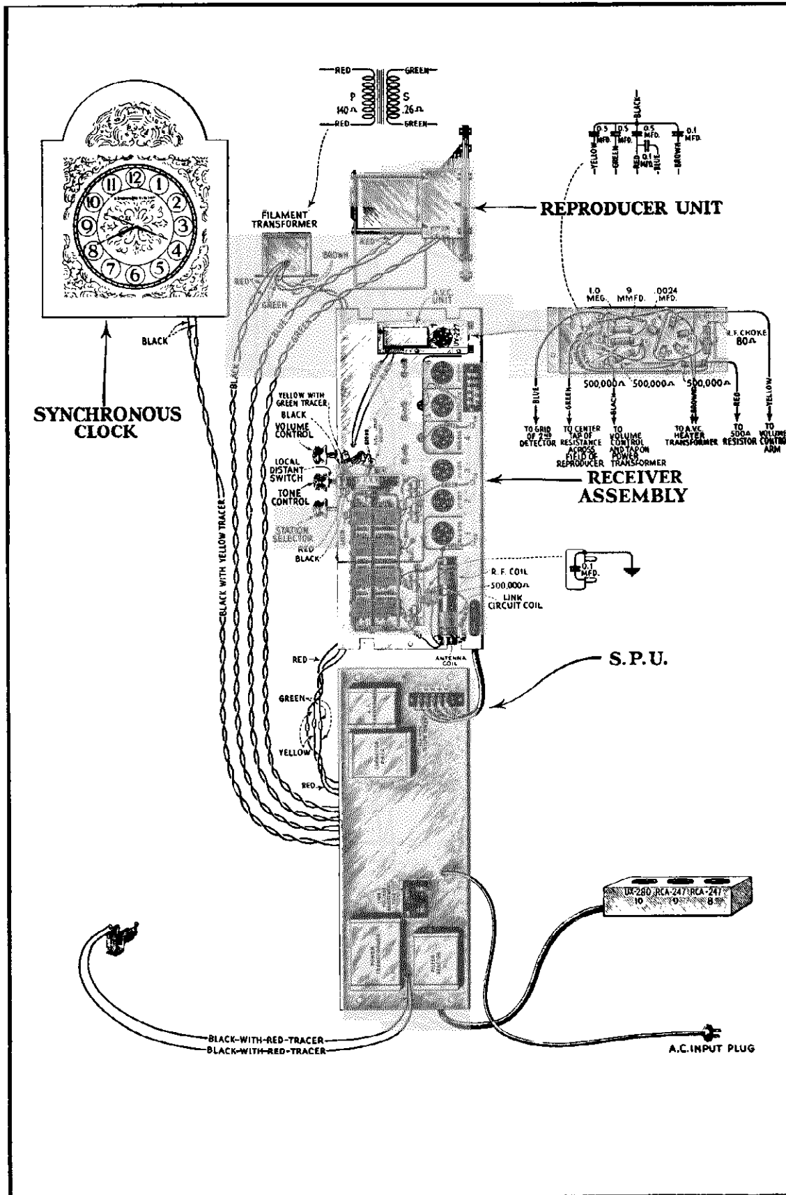
Figure 8—Assembly Wiring of Model H-91
