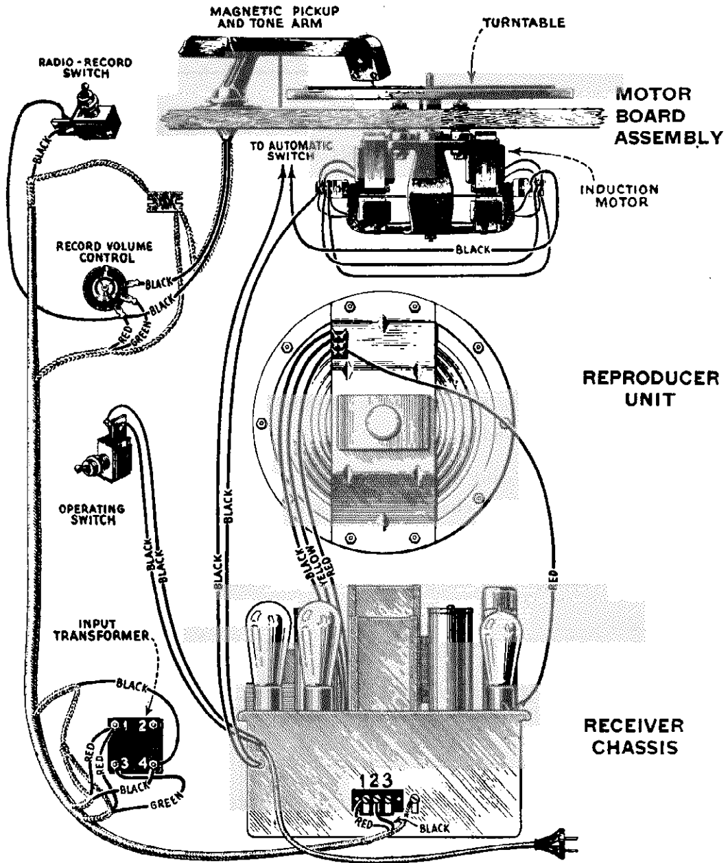
Figure 2—Assembly Wiring Diagram of Model RE-16A
