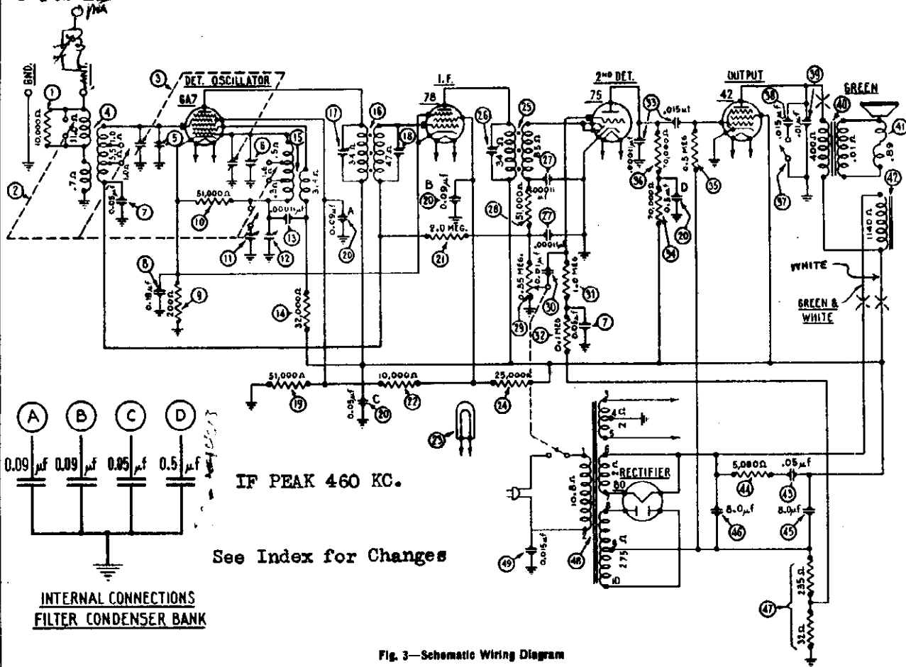
Fig. 3—Schematic Wiring Diagram
