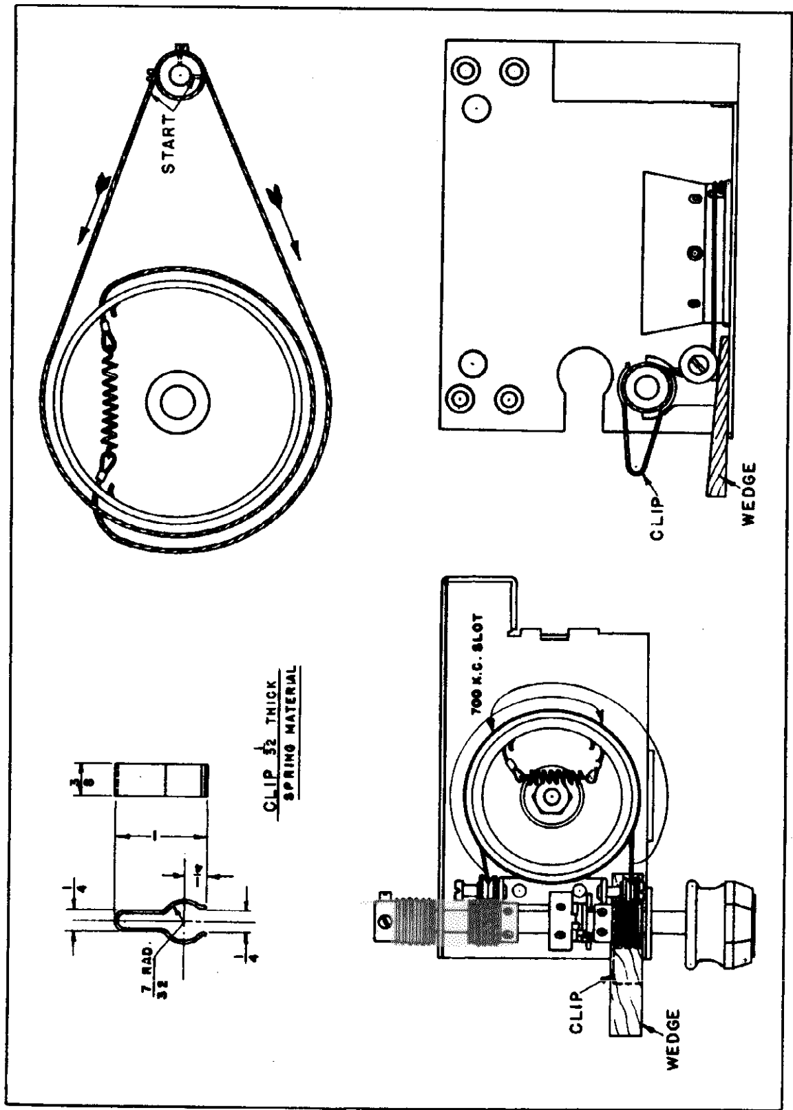
FIG. 34. REPLACING THE DRIVE CABLES
