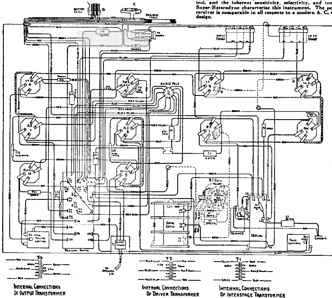
Figure B—Wiring Diagram
