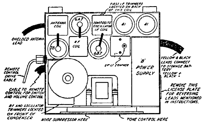
- TOP VIEW OF RECEIVER WITHOUT COVER -
