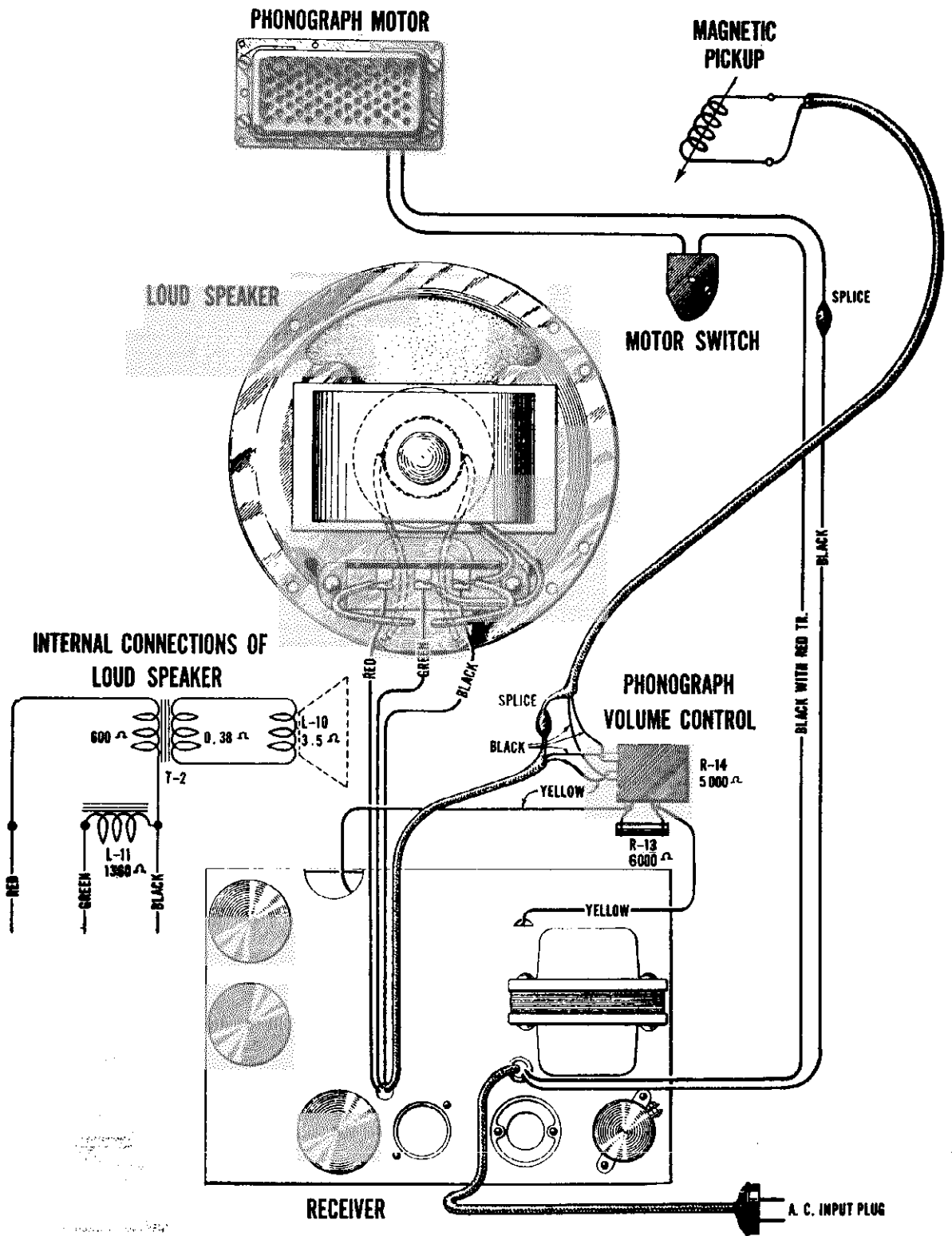
Figure 11—Assembly Wiring
