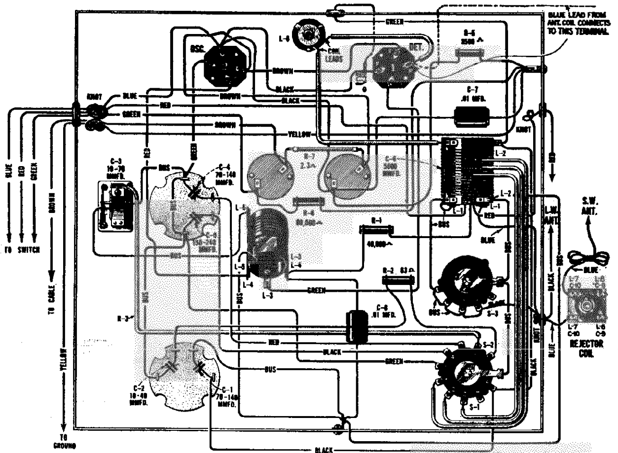
Figure 5—Wiring Diagram of Battery SW-3
