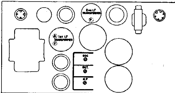
Figure C—Location of Line-up Capacitors
