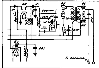
Fig. 7—Revised Audio Circuit in No. 1200 Chassis above Serial No. 1189197
