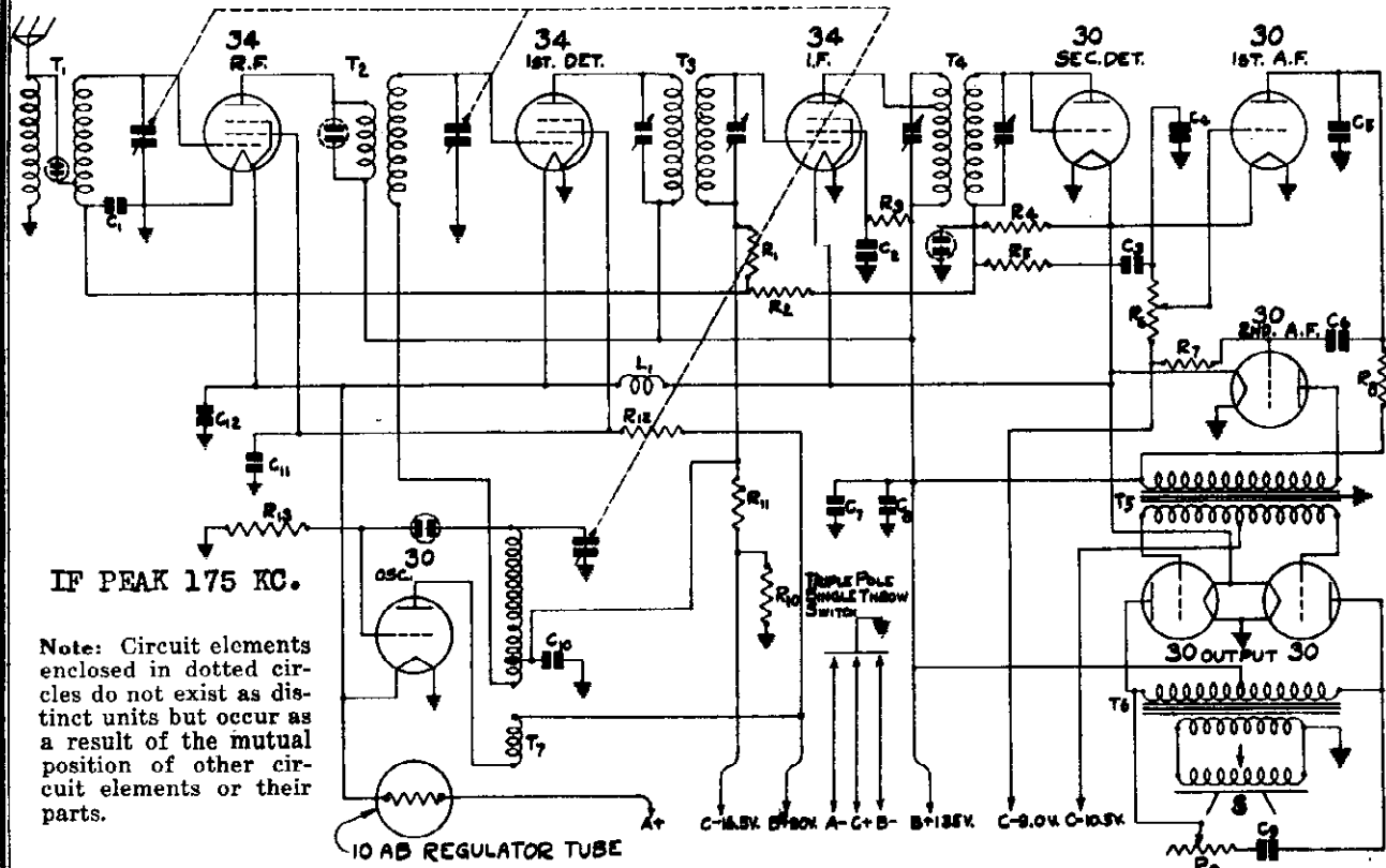
Tube Arrangement and Battery Connections
