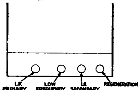
Fig. 3—Back of Model 57 Chassis, showing location of Compensating Condensers and Regeneration Control.
