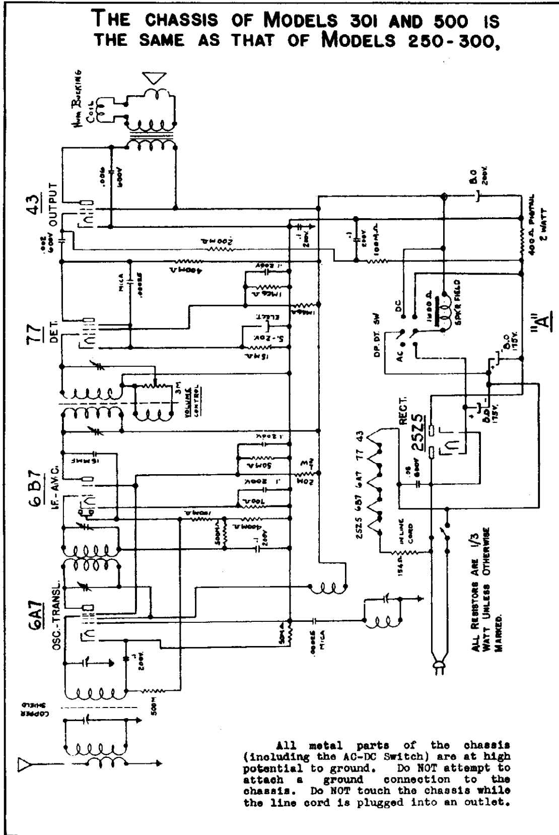
FIG. 19. 128 "A" SCHEMATIC.
