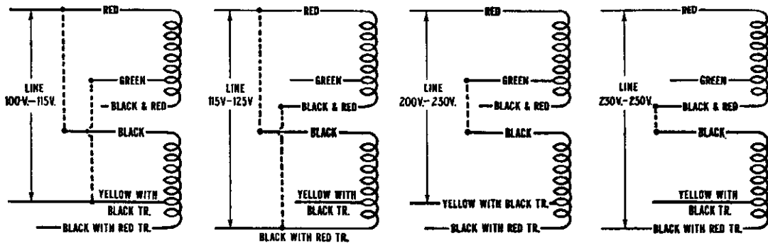
Figure H—End Table Connections
