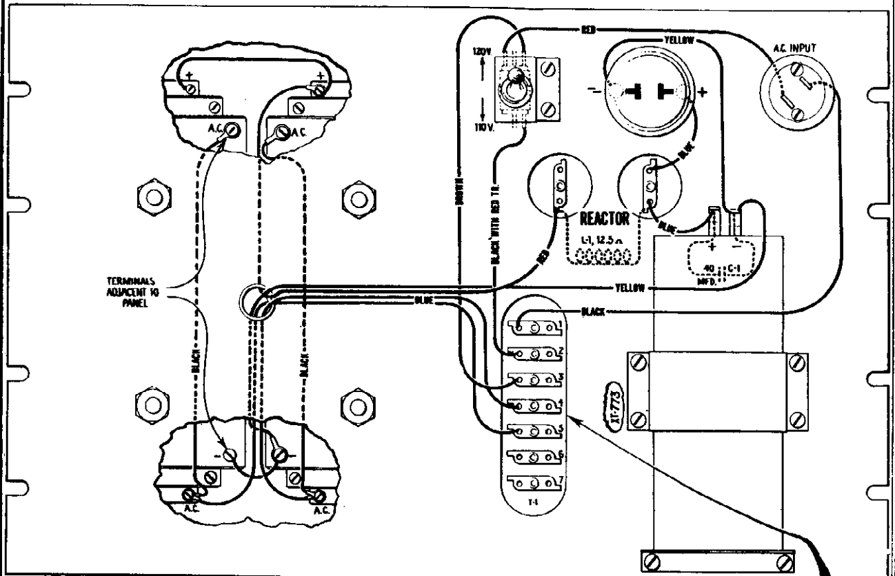
Loudspeaker Field Supply Panel Wiring Diagram (PK21A1)
