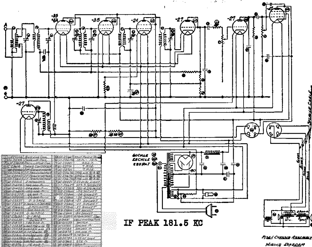
-Circuit Diagram, Model 134-1
