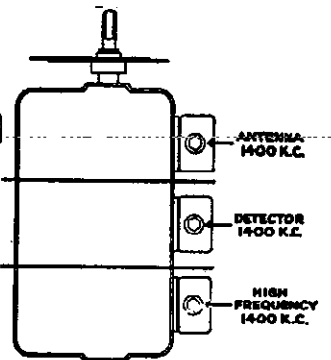
(Above) Back of Philco Model 37 chassis, showing locations of compensating condensers. The 2nd i.f. secondary condenser is mounted on the front of the chassis, but is accessible through the opening in the back, as shown. Fig. 4. (Right) Indicating the locations of the additional compensating condensers.
