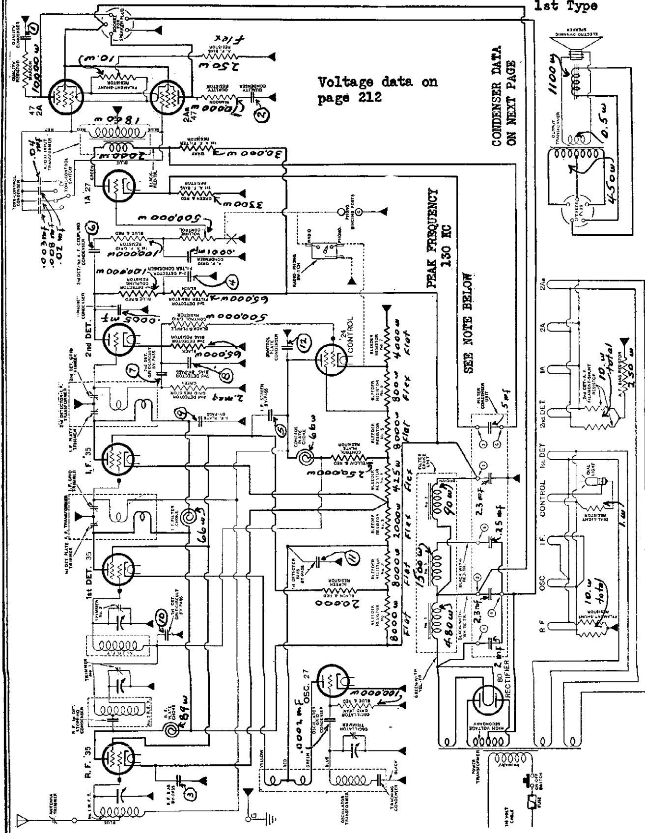
DIAGRAM OF MODEL 89, 89-F, AND 89-P (A. C.-OPERATED). The 2nd-detector grid resistor and the 2nd-detector grid-circuit by-pass are NOT used in this set, and the grid-return of the 2nd-detector connects directly to the chassis. Later types of this Model have No. 1 and No. 2 R. F. transformers connected ahead of the R. F. tube, as shown in the diagram of Model 87 The phonograph-switching circuit in 89-P is shown above in dotted lines.
