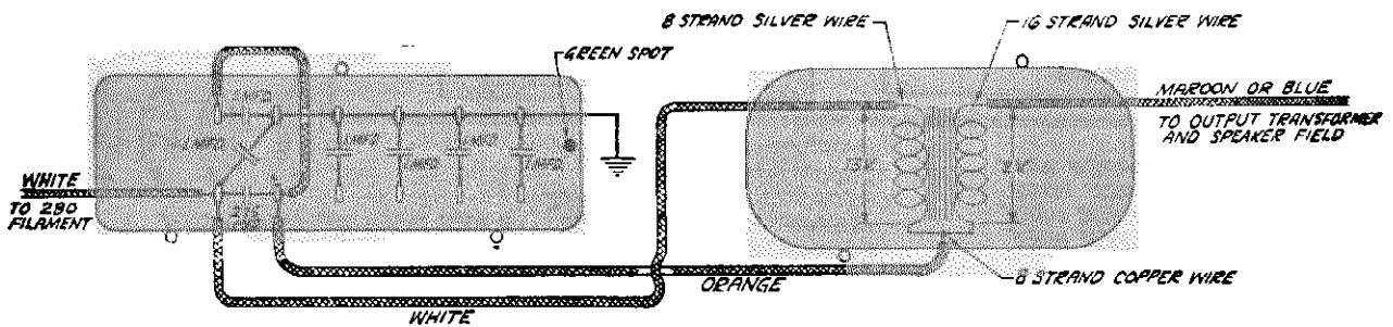
CONNECTIONS OF FILTER CHOKE AND CONDENSERS
