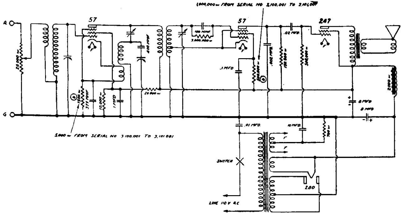
SCHEMATIC DIAGRAM
