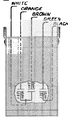
CONNECTIONS OF 25 CYCLE ADDED FILTER CONDENSERS
