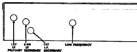
(Above) Back of Philco Model 37 chassis, showing locations of compensating condensers. The 2nd i.f. secondary condenser is mounted on the front of the chassis, but is accessible through the opening in the back, as shown. Fig. 4. (Right) Indicating the locations of the additional compensating condensers.
