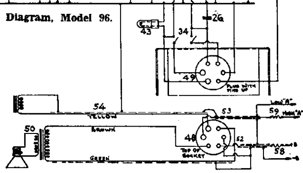
CHASSIS ASSEMBLY WIRING DIAGRAM
