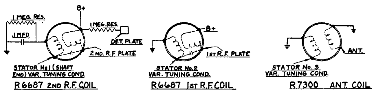
COIL CONNECTIONS VIEWED FROM BOTTOM OF CHASSIS
