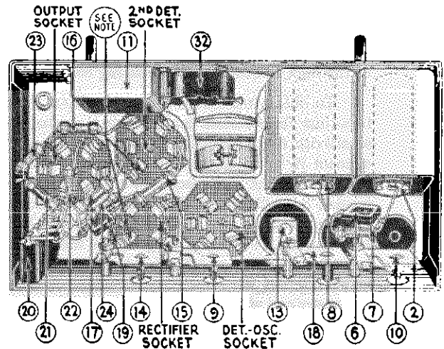
Fig. 3—Bottom View of Chassis, Showing Parts
