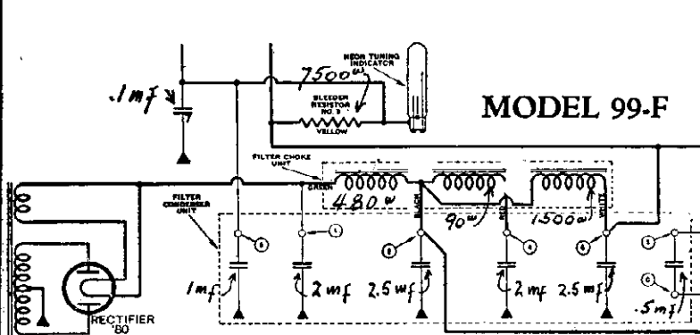
FILTER CIRCUIT OF MODEL 99-F
