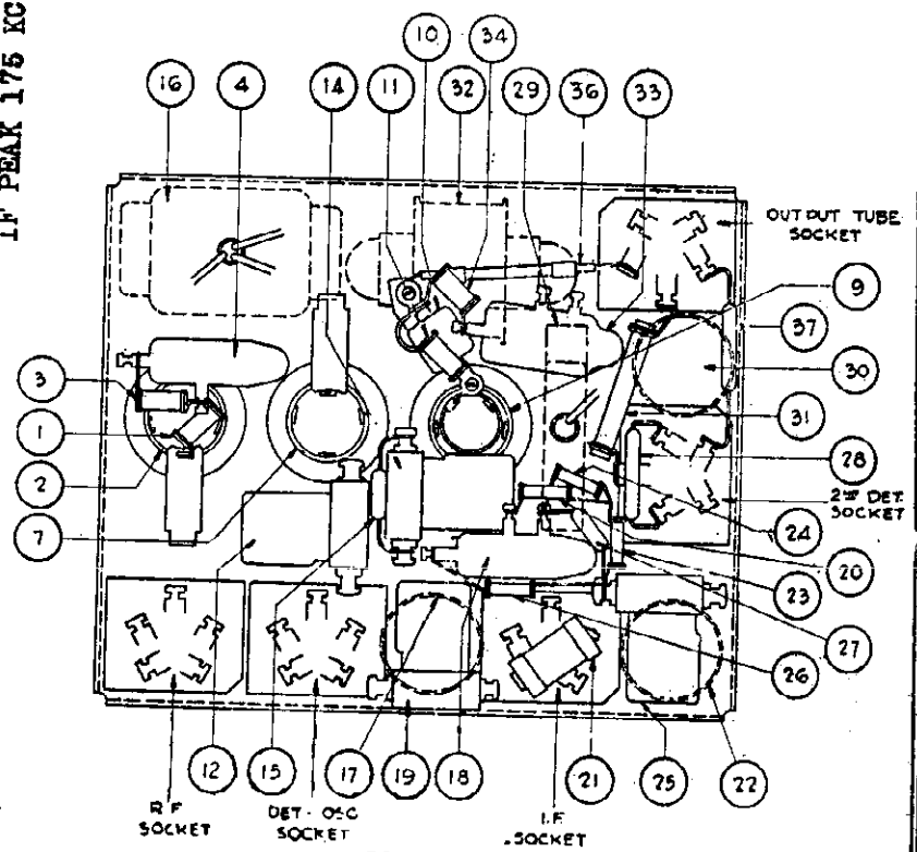
Model 7—Chassis
