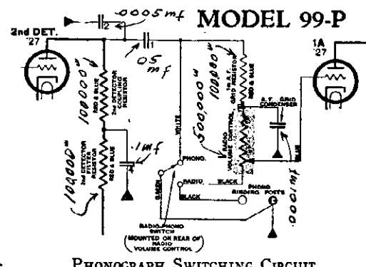
PHONOGRAPH SWITCHING CIRCUIT
