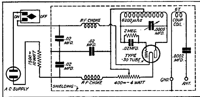
Model 60 Oscillator
