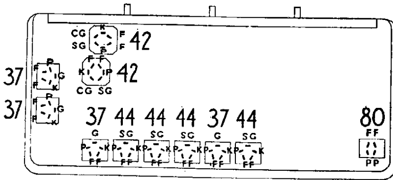
Fig. 1—Tube Sockets F Filament SG Screen Grid K Cathode P Plate CG Control Grid
