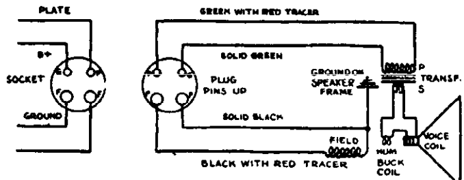
SPEAKERS 297 AND 305-J FOR CHASSIS 122
