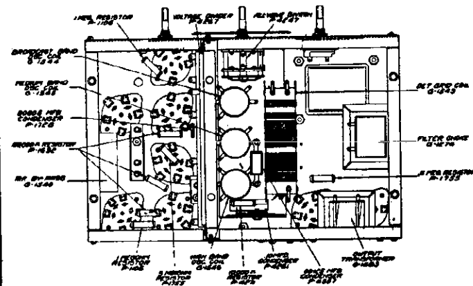
G-240 CHASSIS BOTTOM VIEW
