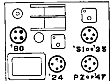
TUBE LOCATIONS
