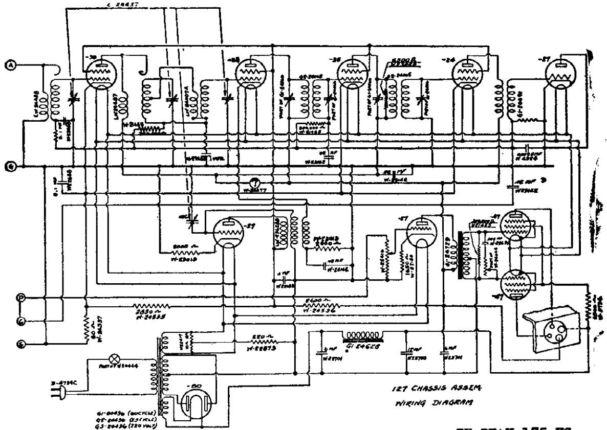
-Circuit Diagram, Model 127.
