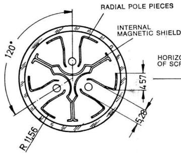
LOCATION OF RADIAL-CONVERGING POLE PIECES
