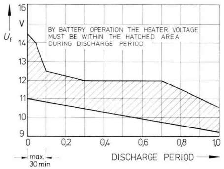
Heater voltage for battery operation.
