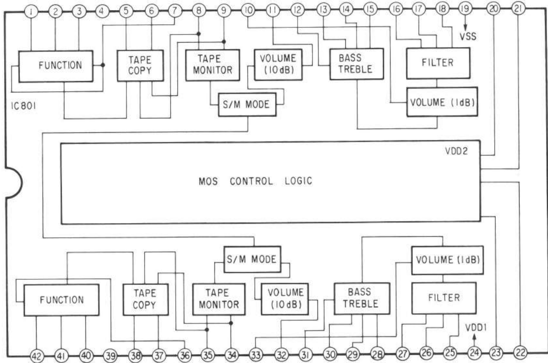
IC801 CX789
