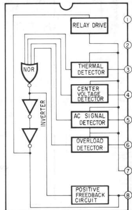
IC401 HAI2002
