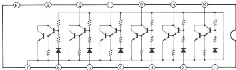
IC706 M54517P
