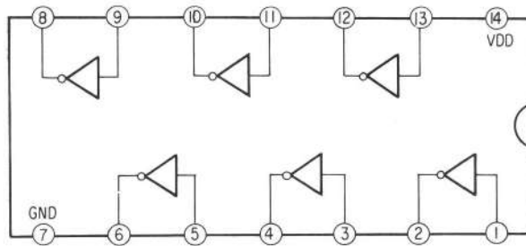
IC704 MB84069B
