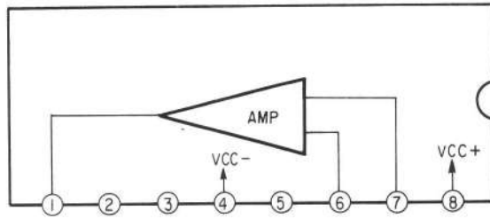
IC101, 151, 802, 804 CX550
