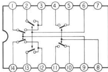
IC803 CX770
