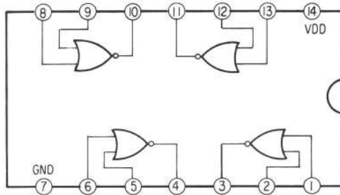
IC705 MB84001B
