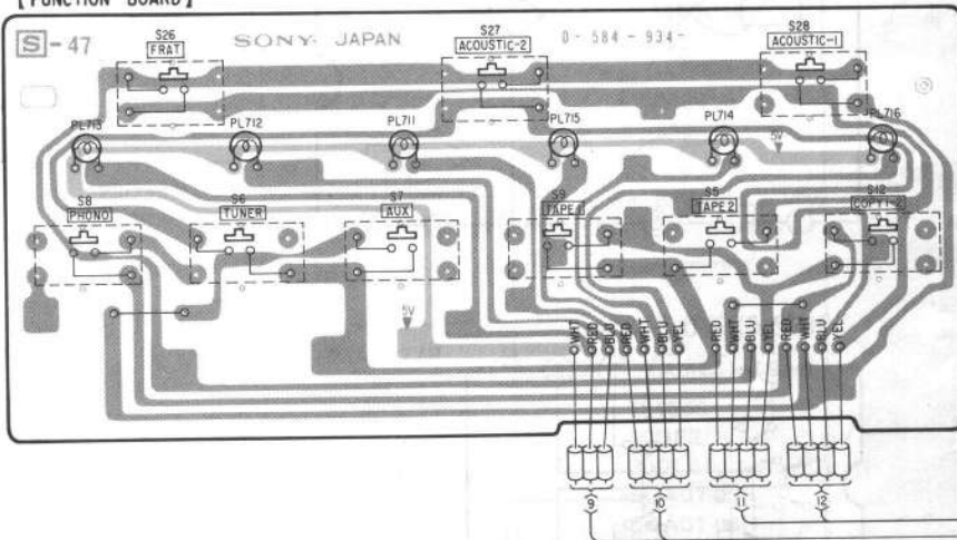
[FUNCTION BOARD]
