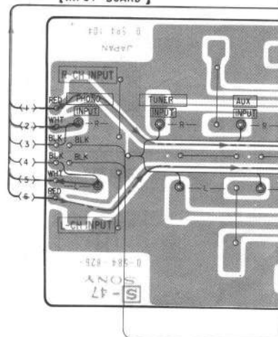
[ INPUT BOARD ]
