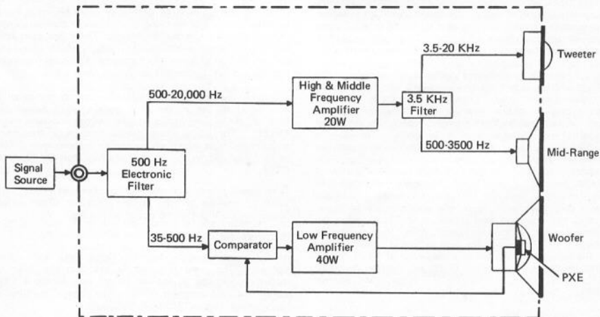
Figure 1, Block Diagram
