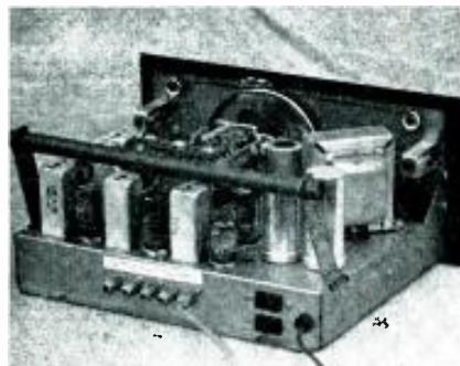
Rear view of the AFM tuner. Inputs and outputs are conveniently grouped on the rear of the chassis. The bar is the AM antenna.
