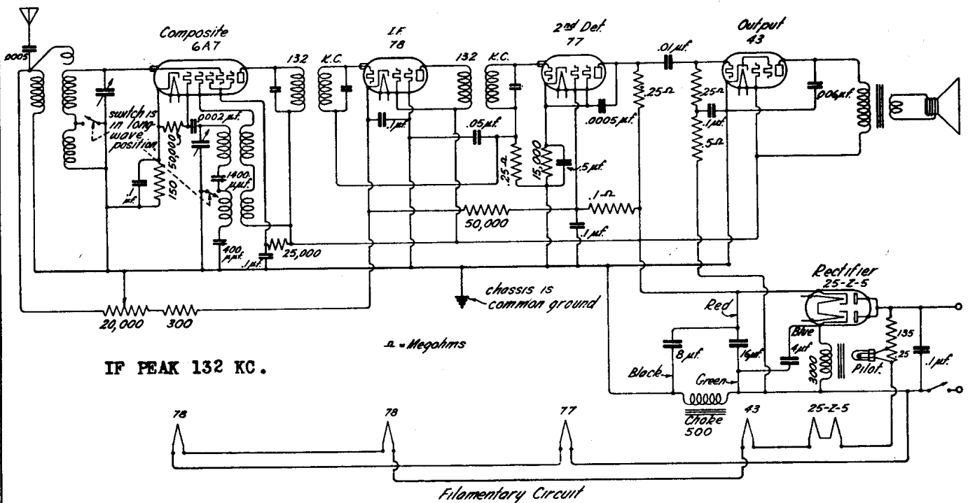
SCHEMATIC CIRCUIT OF MODEL H-5-L
