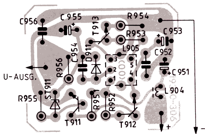
30 V WANDLER-PLATTE 30V TRANSFORMER BOARD
