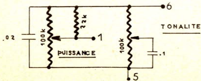
POTENTIOMETRES
