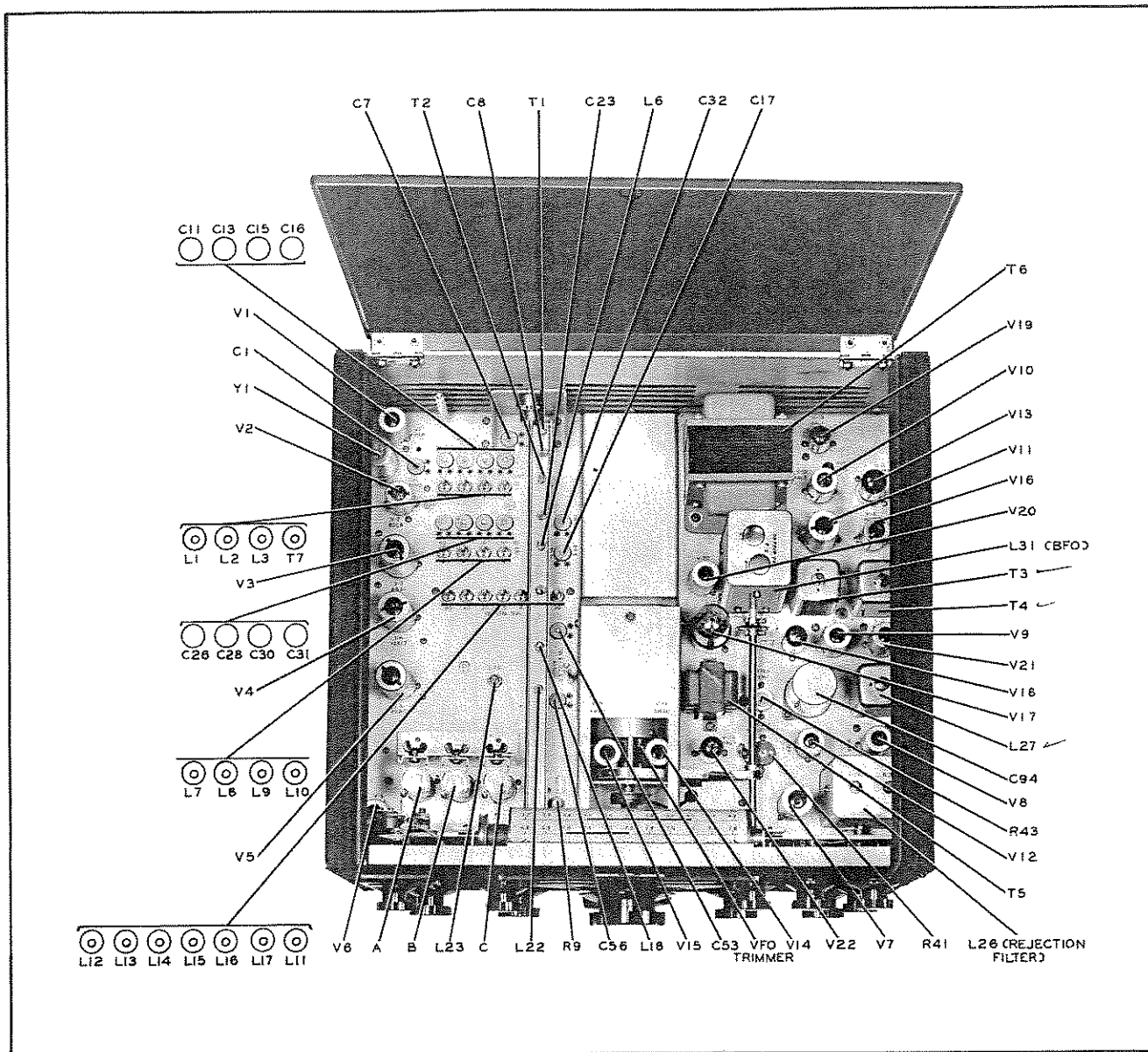
Figure 5-2. 75A-4, Top View
