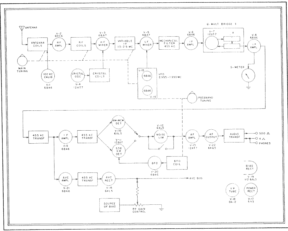
Figure 1-1. 75A-4 Receiver and Block Diagram
