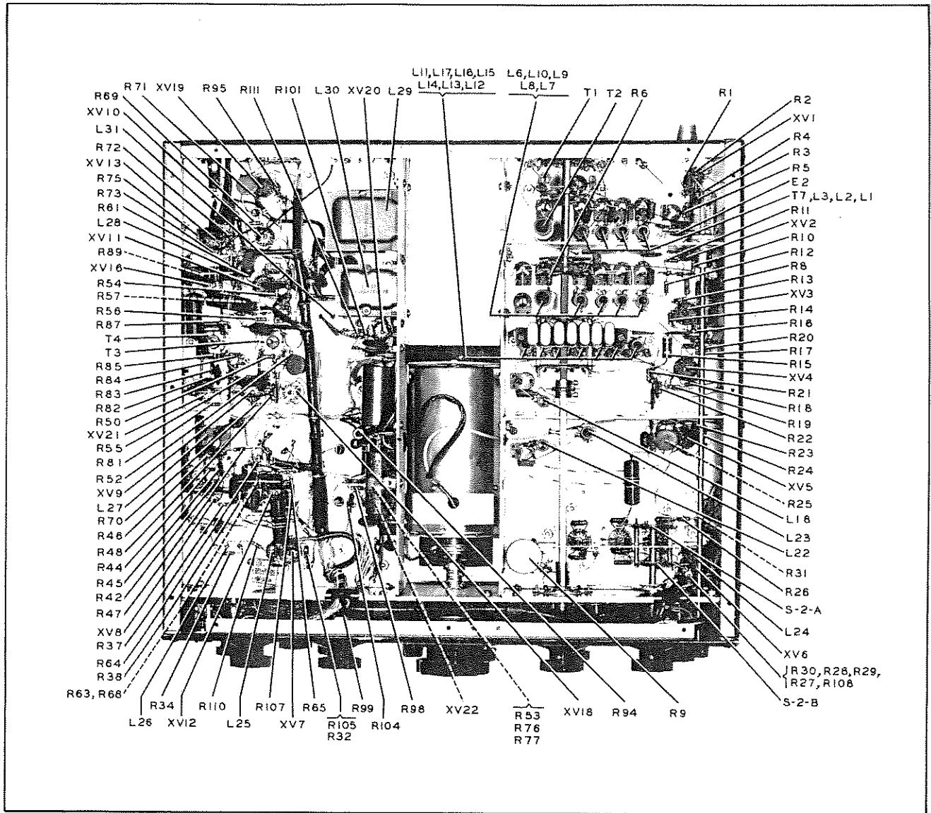
Figure 5-3. 75A-4, Bottom View, Page 2
