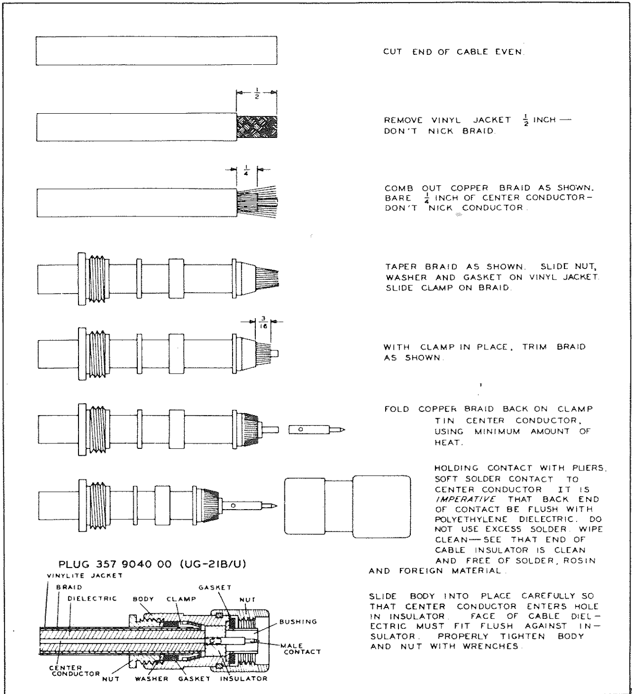
Figure 5-6. Assembling Plug UG-21B/U to Cable RG-8/U
