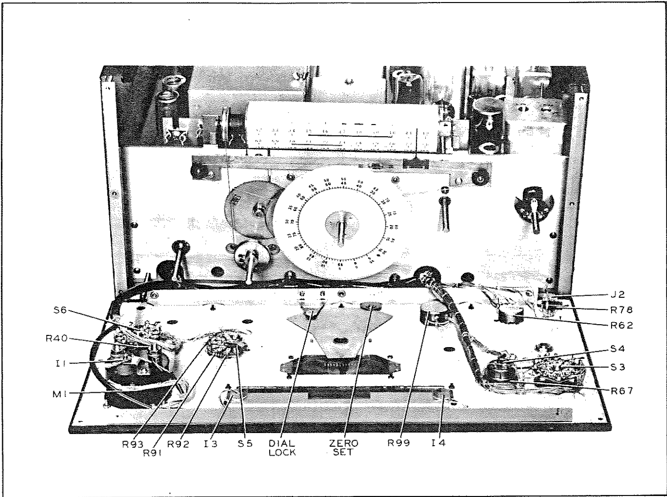
Figure 5-4. 75A-4, Front Panel Lowered
