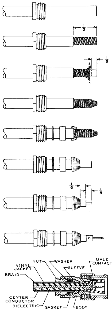
Figure 5-8. Assembling Plug UG-260/U to Cable UG-58/U
