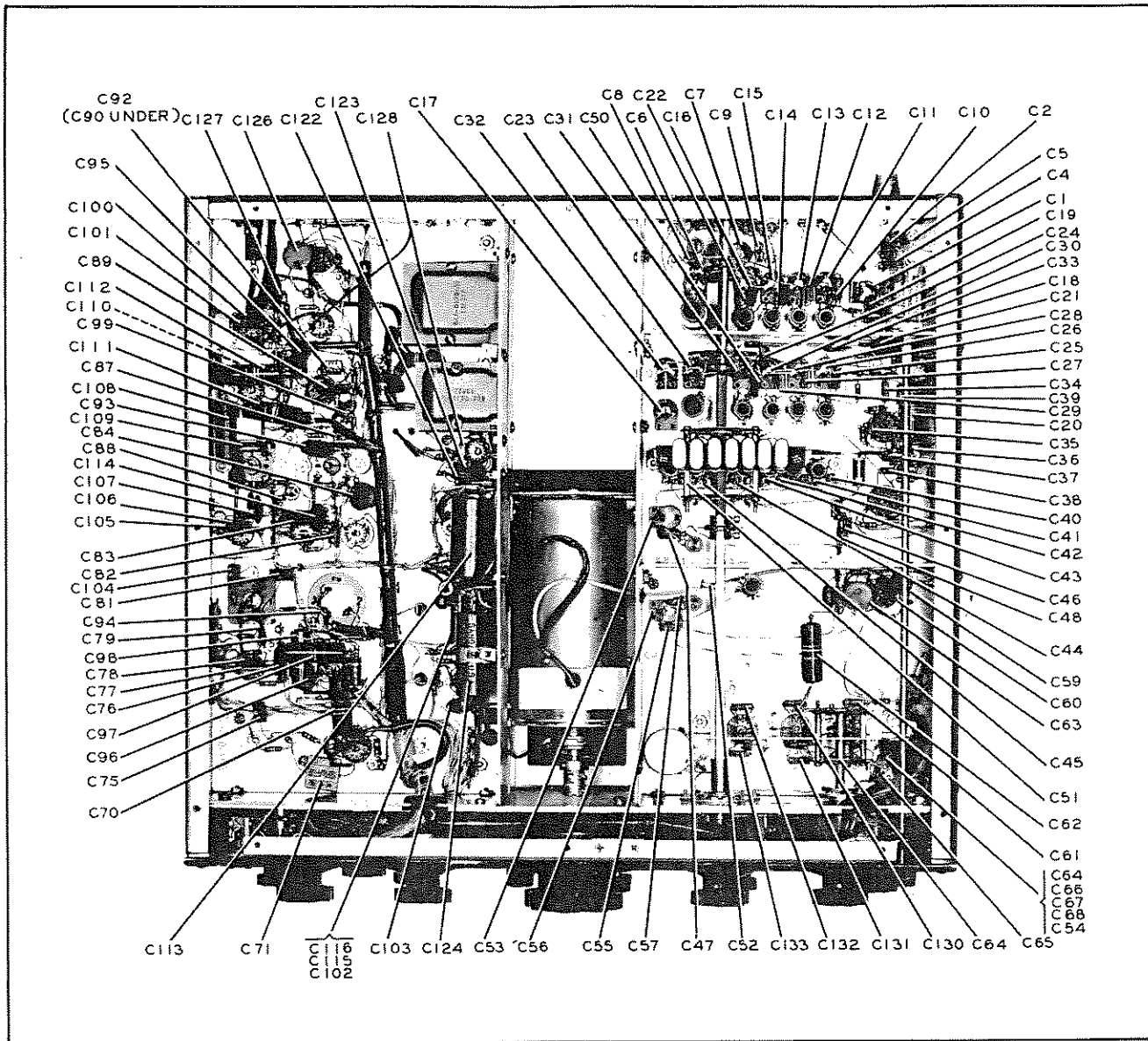
Figure 5-3. 75A-4, Bottom View, Page 1
