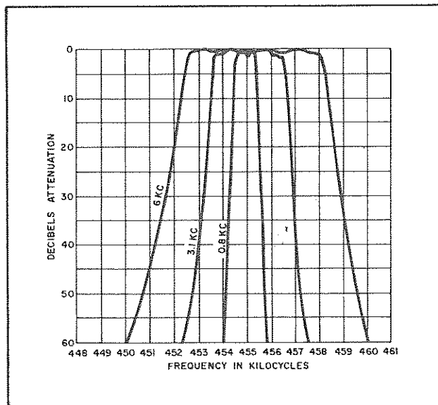
Figure 1-3. 75A-4 Selectivity Curves
