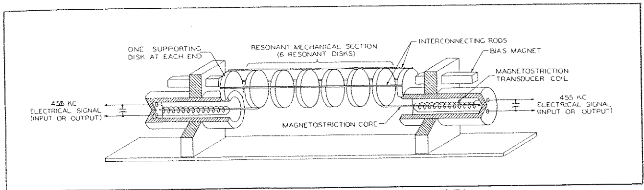
Figure 4-2. A Collins Mechanical Filter, Functional Diagram
