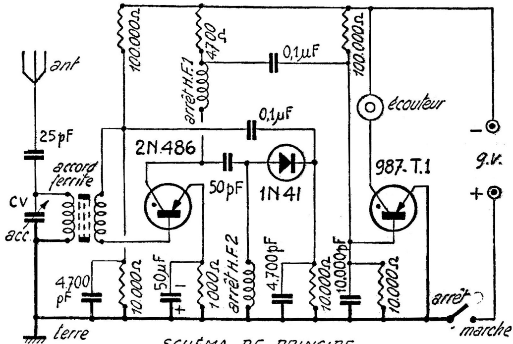
SCHEMA DE PRINCIPLE
