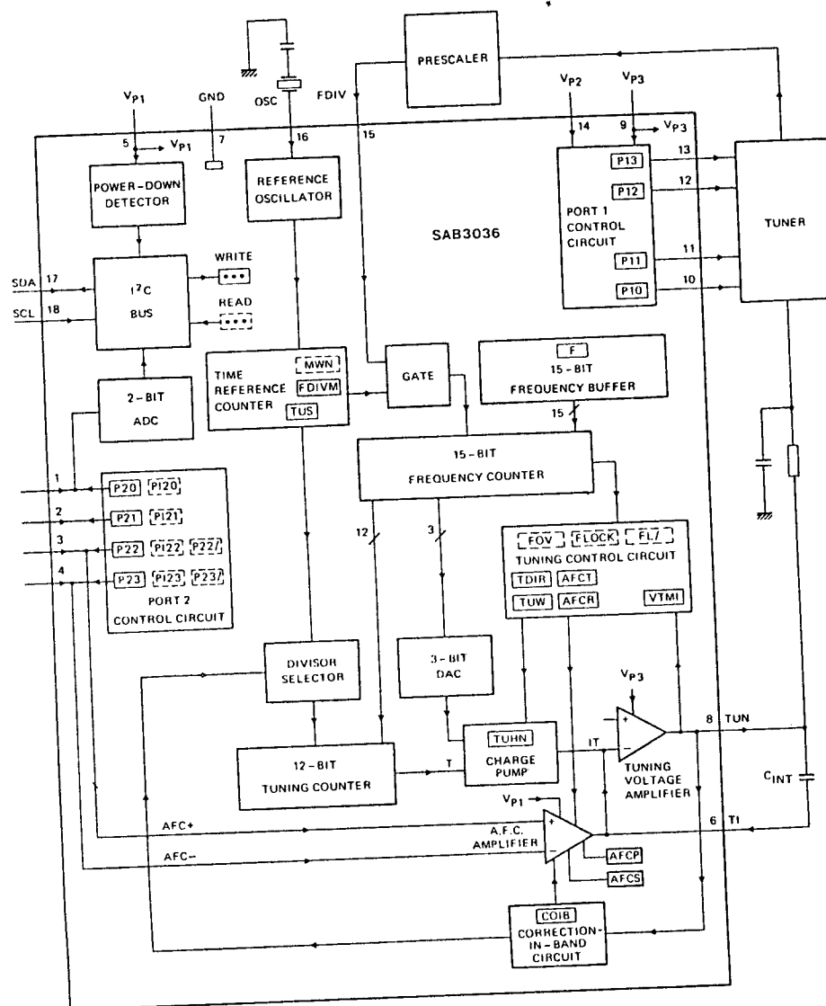
Fig. 1 Block diagram.
