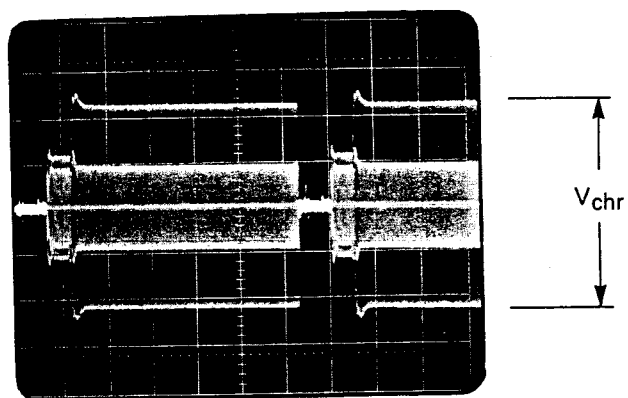
Fig. 56 Chroma signal SECAM pattern purity cyan
