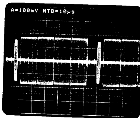
Fig. 52 Chroma signal PAL D,G,I,N
