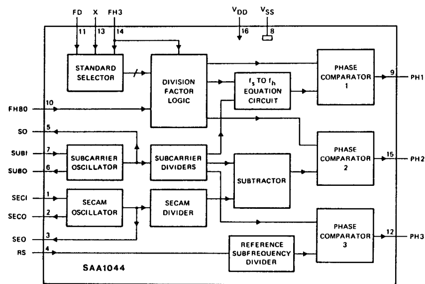
Fig. 1 Block diagram.
