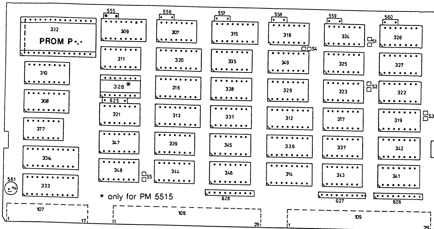
Fig. 108 Unit 1: digital unit
