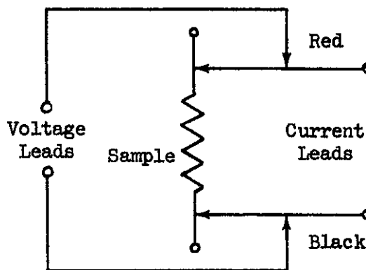
FIGURE 4. Two-terminal connection.
