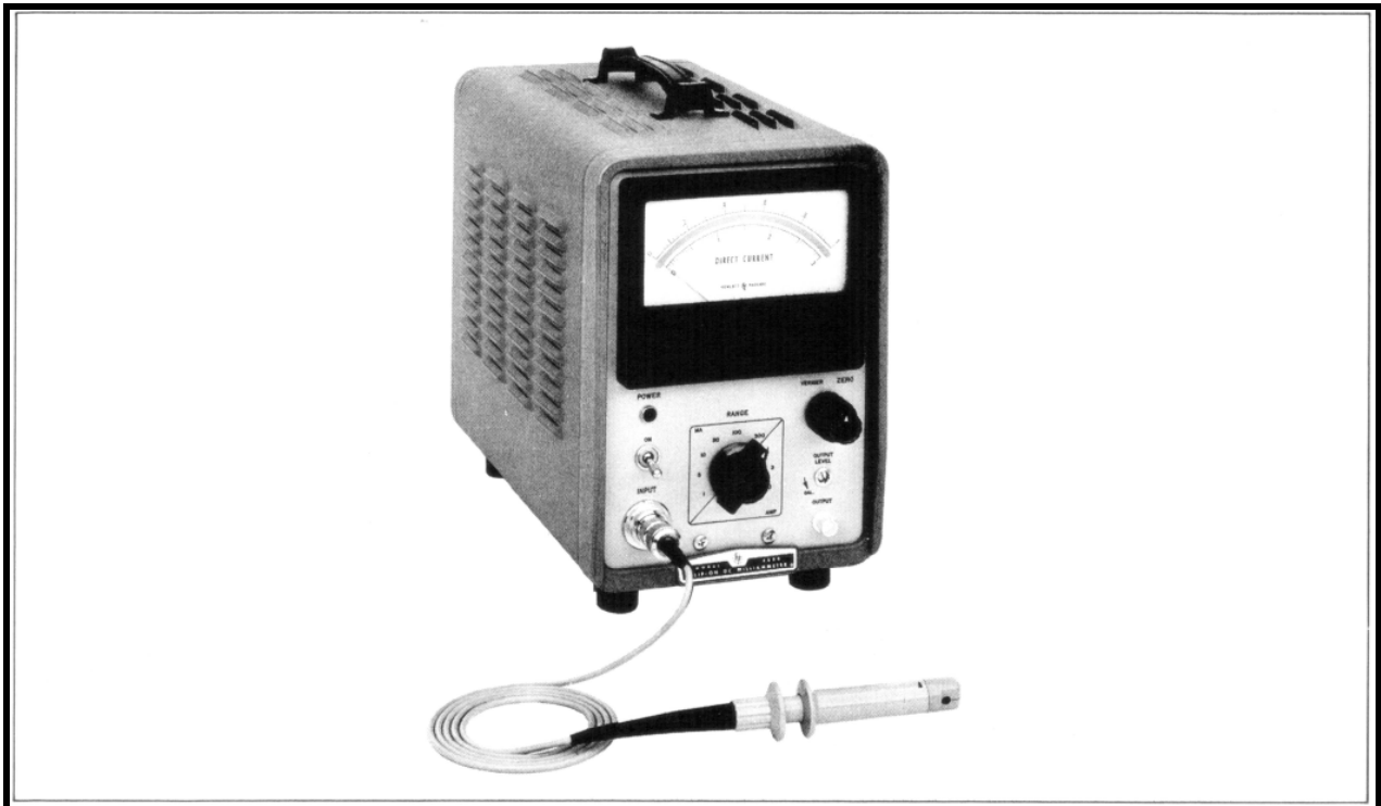
Figure 1-1. Model 428B Clip-On Milliammeter
