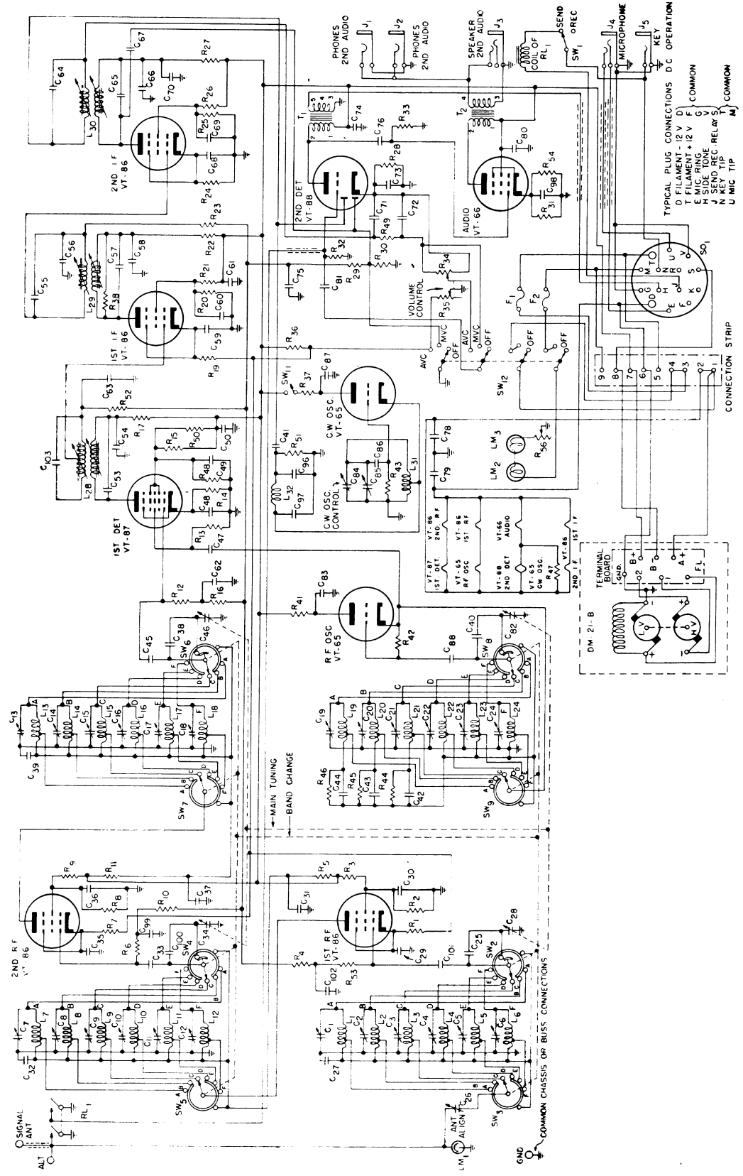
FIGURE 6. RADIO RECEIVER BC-312-N, CIRCUIT DIAGRAM.
