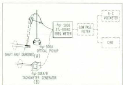
Fig. 11. Set-ups for measuring torsional vibration in rotating equipment. (A) shows use of hp -optical pickup, (B) use of hp -tachometer generator for converting mechanical effect to electrical signal.
