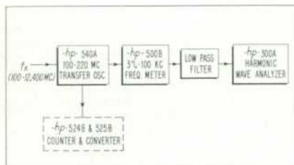
Fig. 8. Set-up for measuring components of f-m modulating waveform in frequencies from 100 to 12,400 mc.
