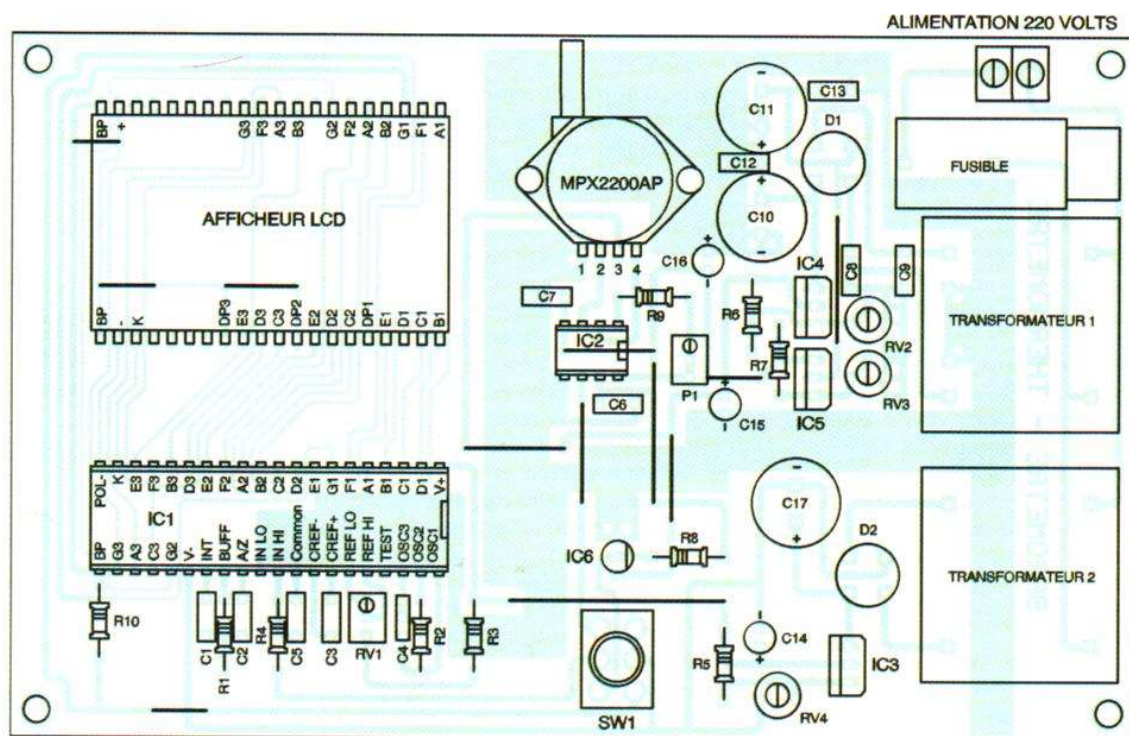
Figure 8 - Implantation des composants.
