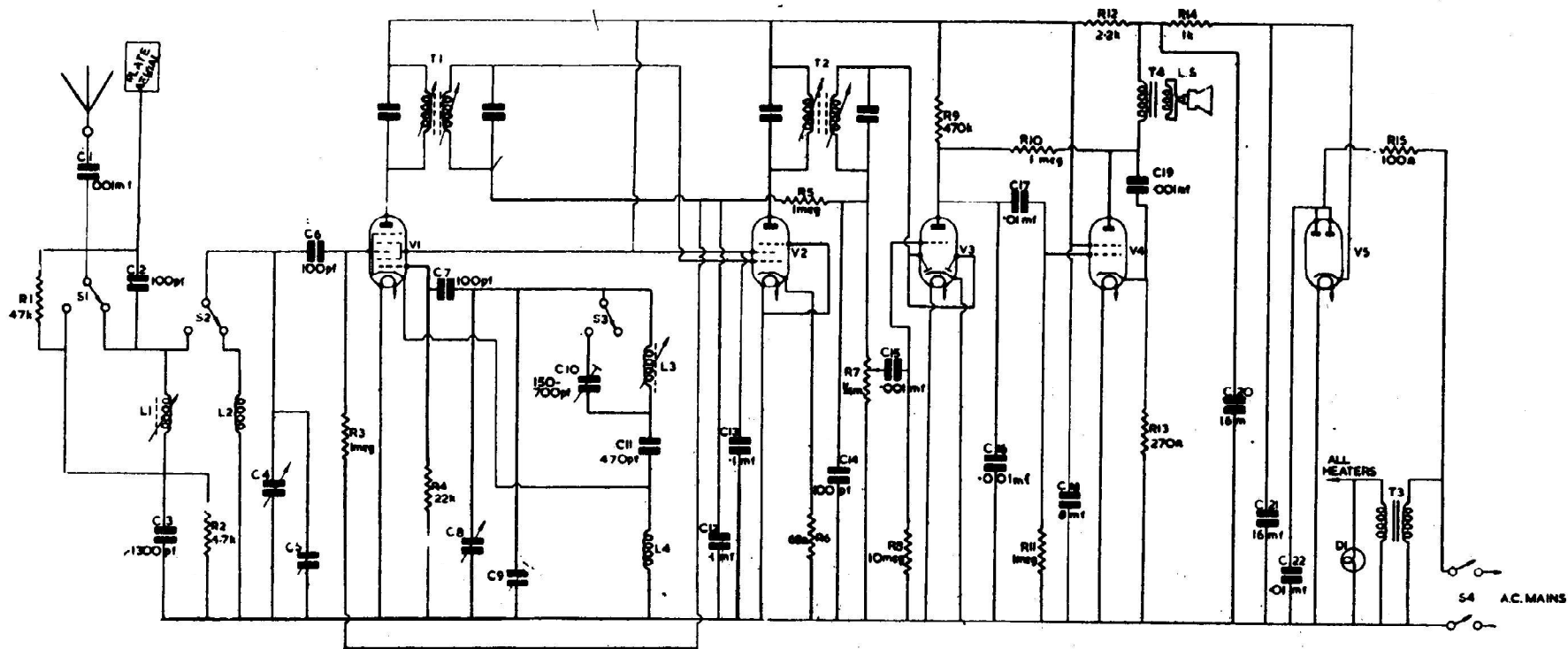
CIRCUIT DIAGRAM—PILOT LITTLE MAESTRO MODEL 10
