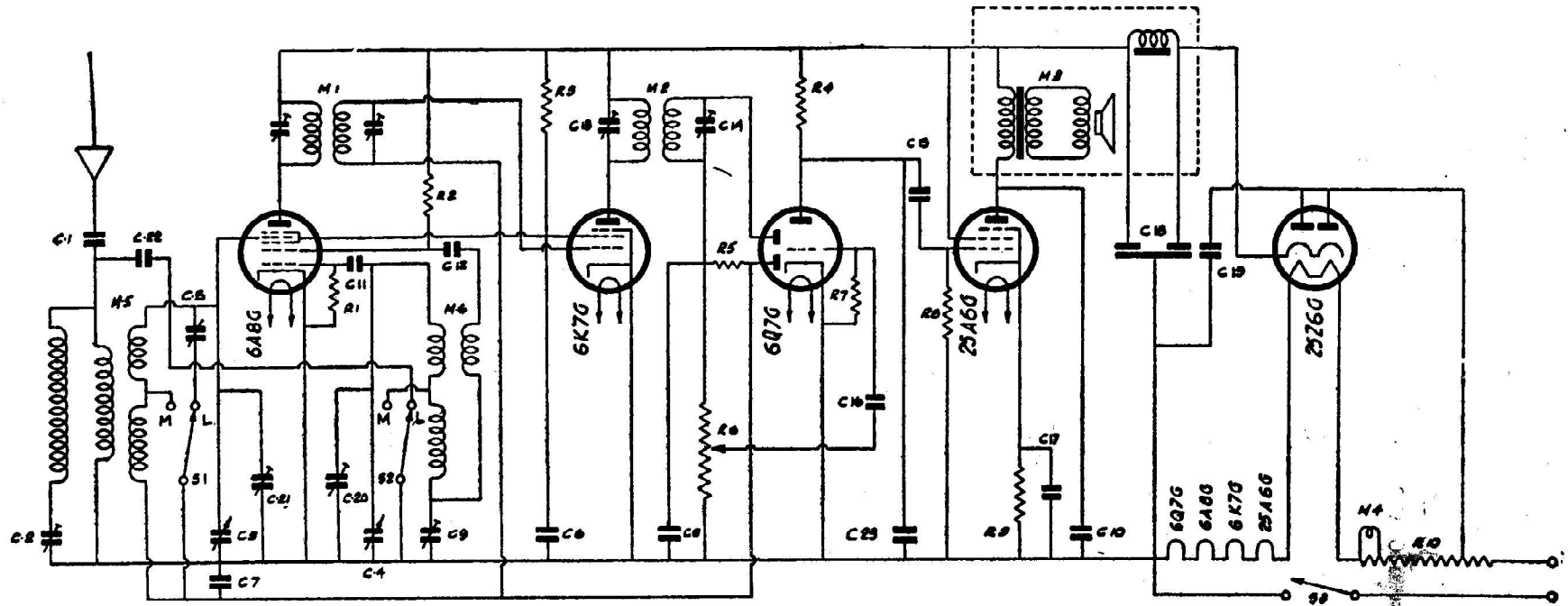
CIRCUIT DIAGRAM—PILOT LITTLE MAESTRO MODEL 1
