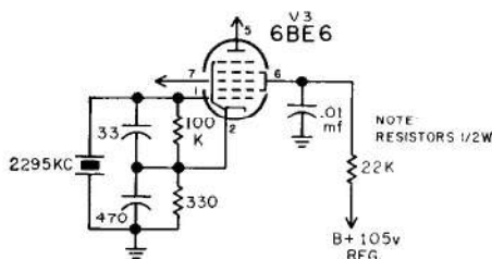
Fig. 1—Crystal controlled second converter.
