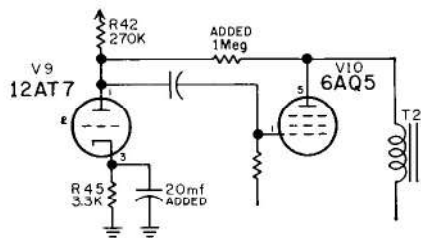
Fig. 2—Two new components improves audio.
