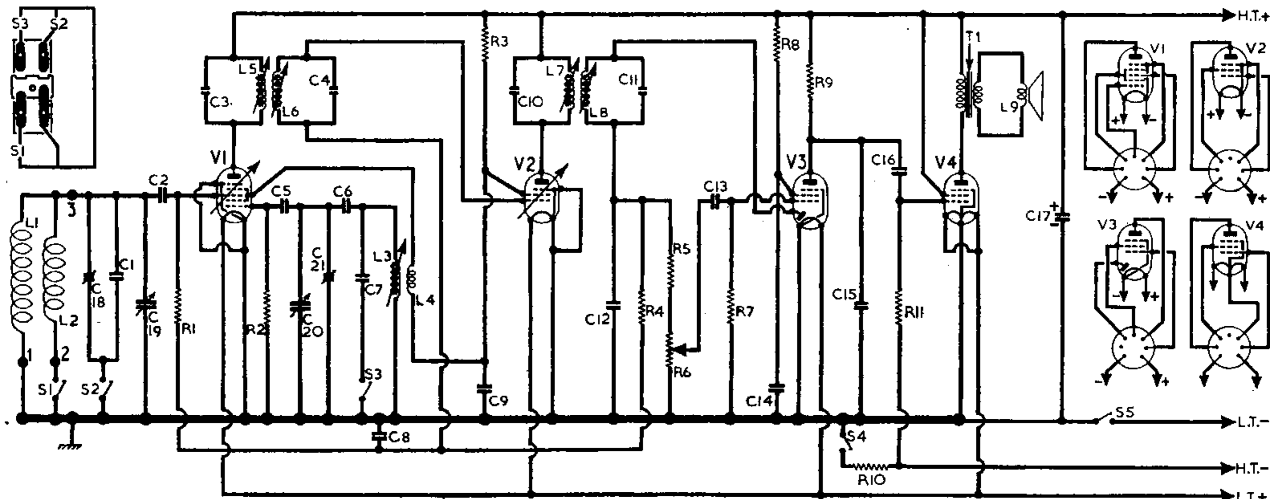
Circuit diagram of the Vidor CN414 all-dry battery portable superhet. Inset in the top left-hand corner is a diagram of the waveband switch.
