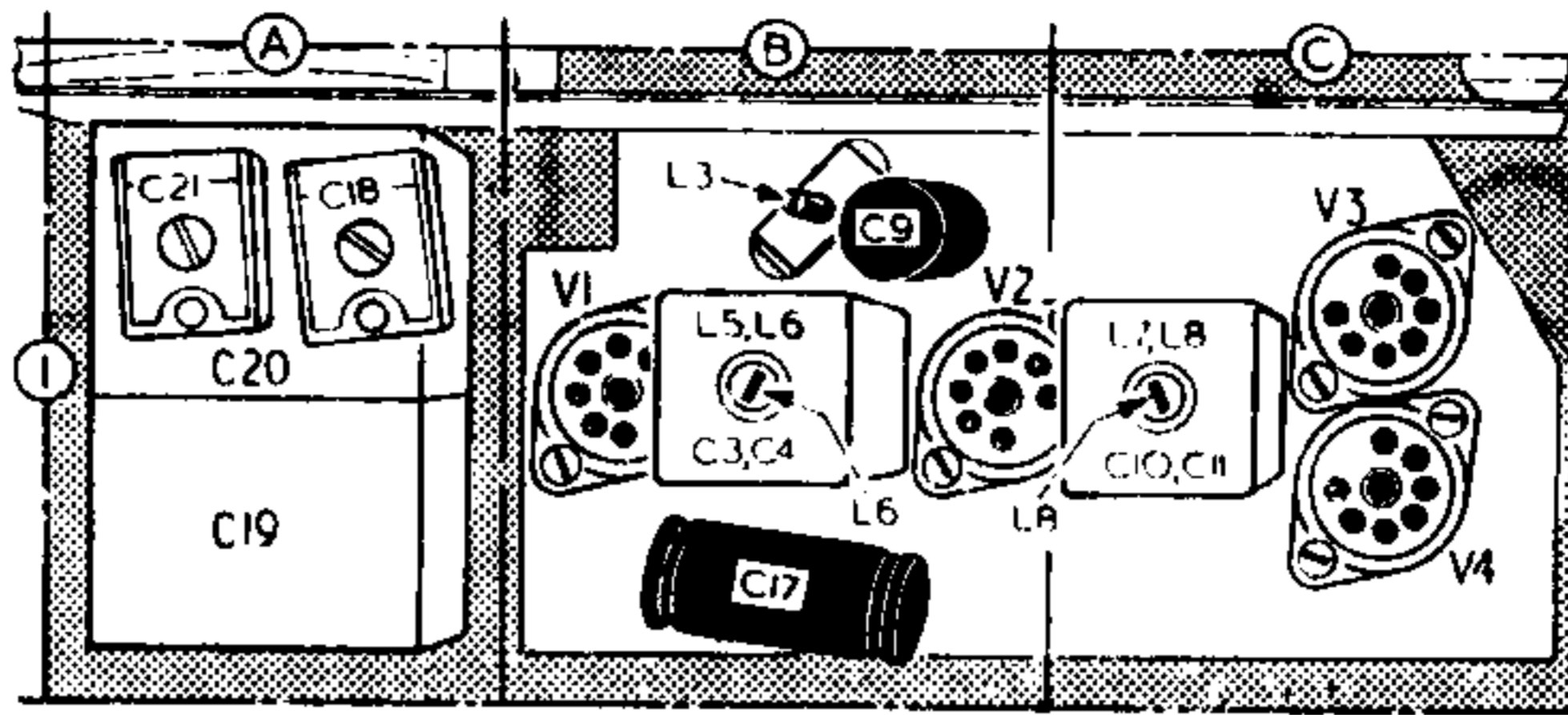
Above: Plan view of the chassis.
