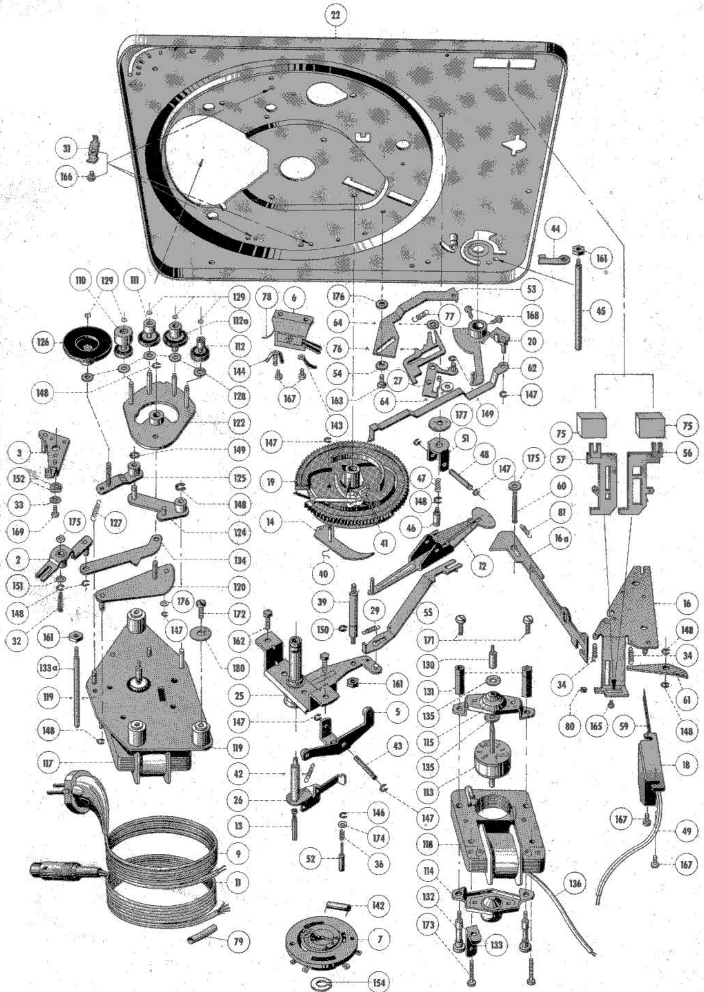
Fig. 15, parts below chassis
