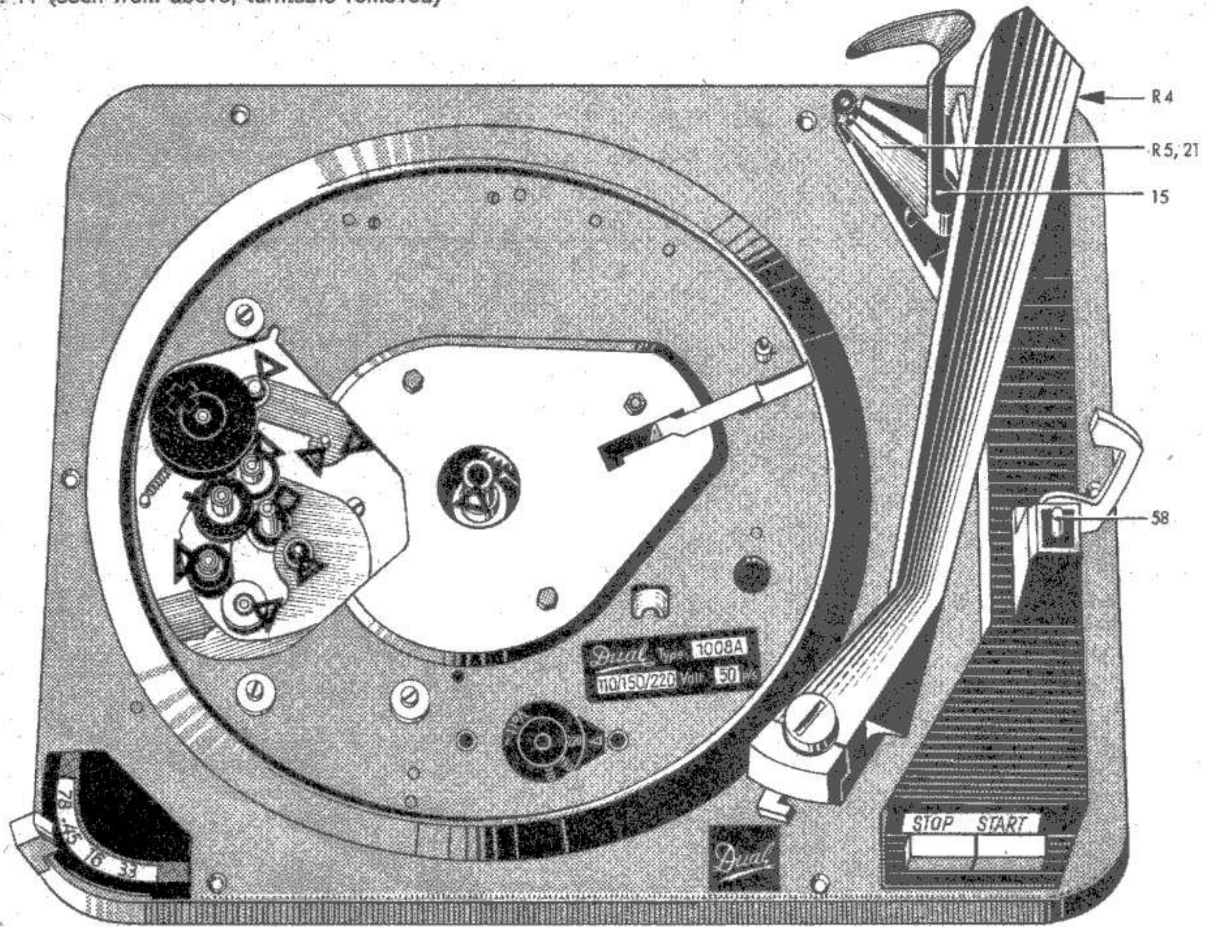
Fig. 11 (seen from above, turntable removed)
