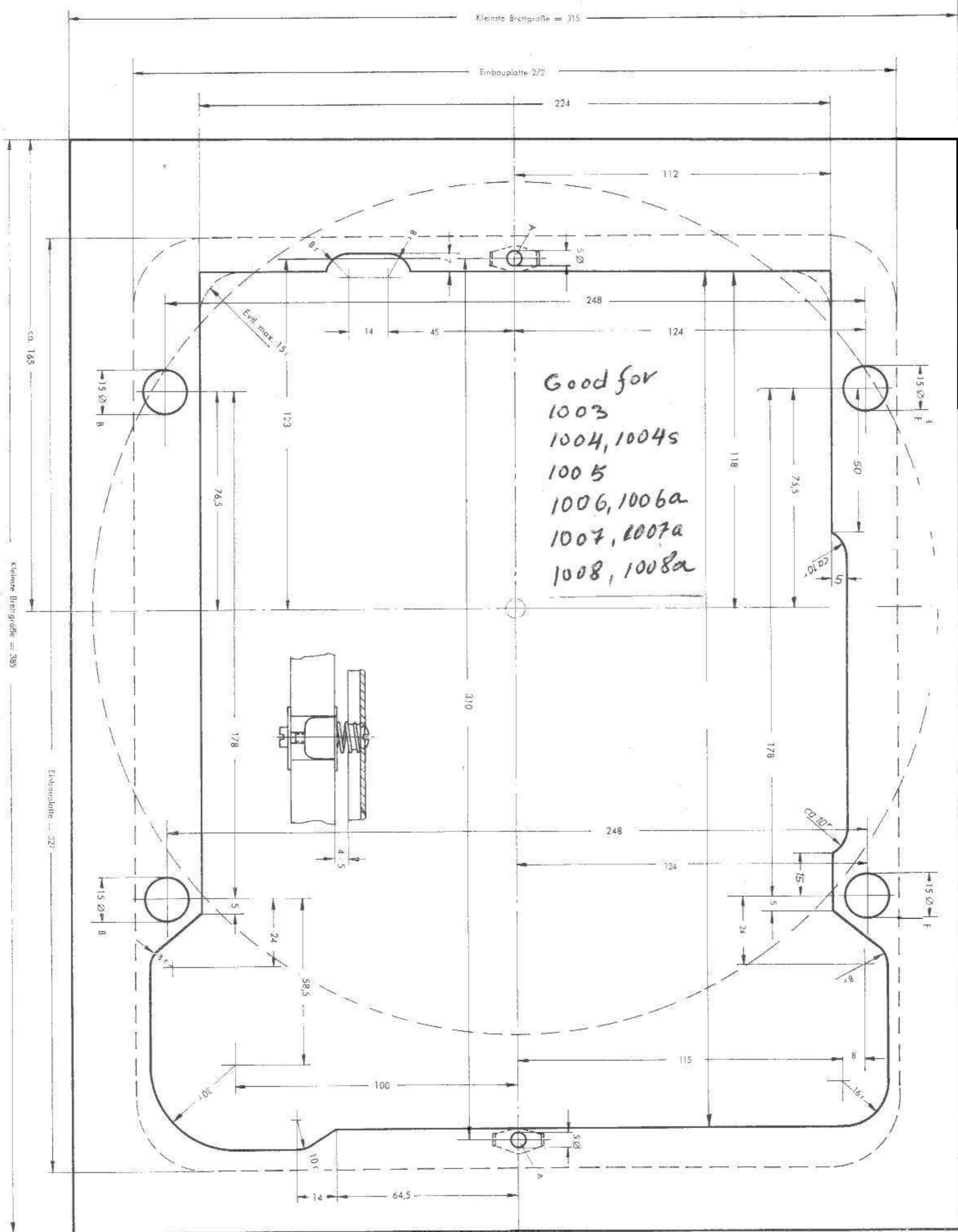
Fig. 13, Mounting Template
