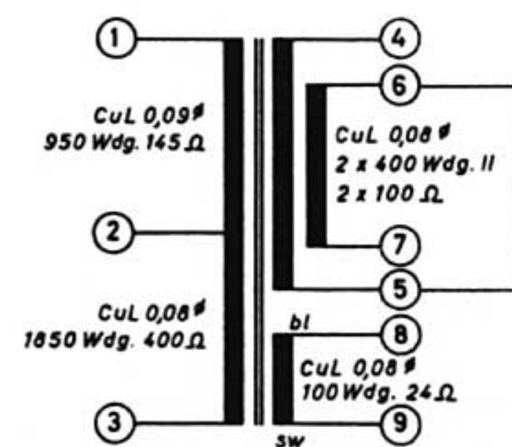
BV 9030-520 Treibtrafo Driver Transformer Transfo Driver
