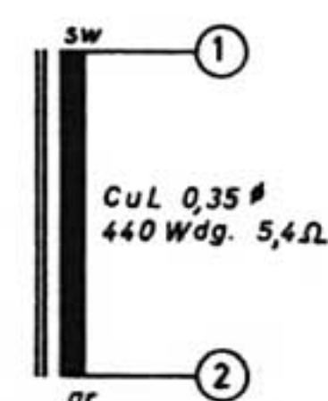
BV 9038-519 Drossel Choke Self
