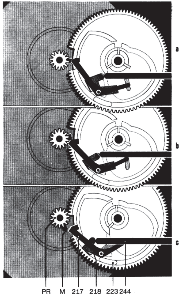
Fig. 16 Actuating "change" or "shut-off"
