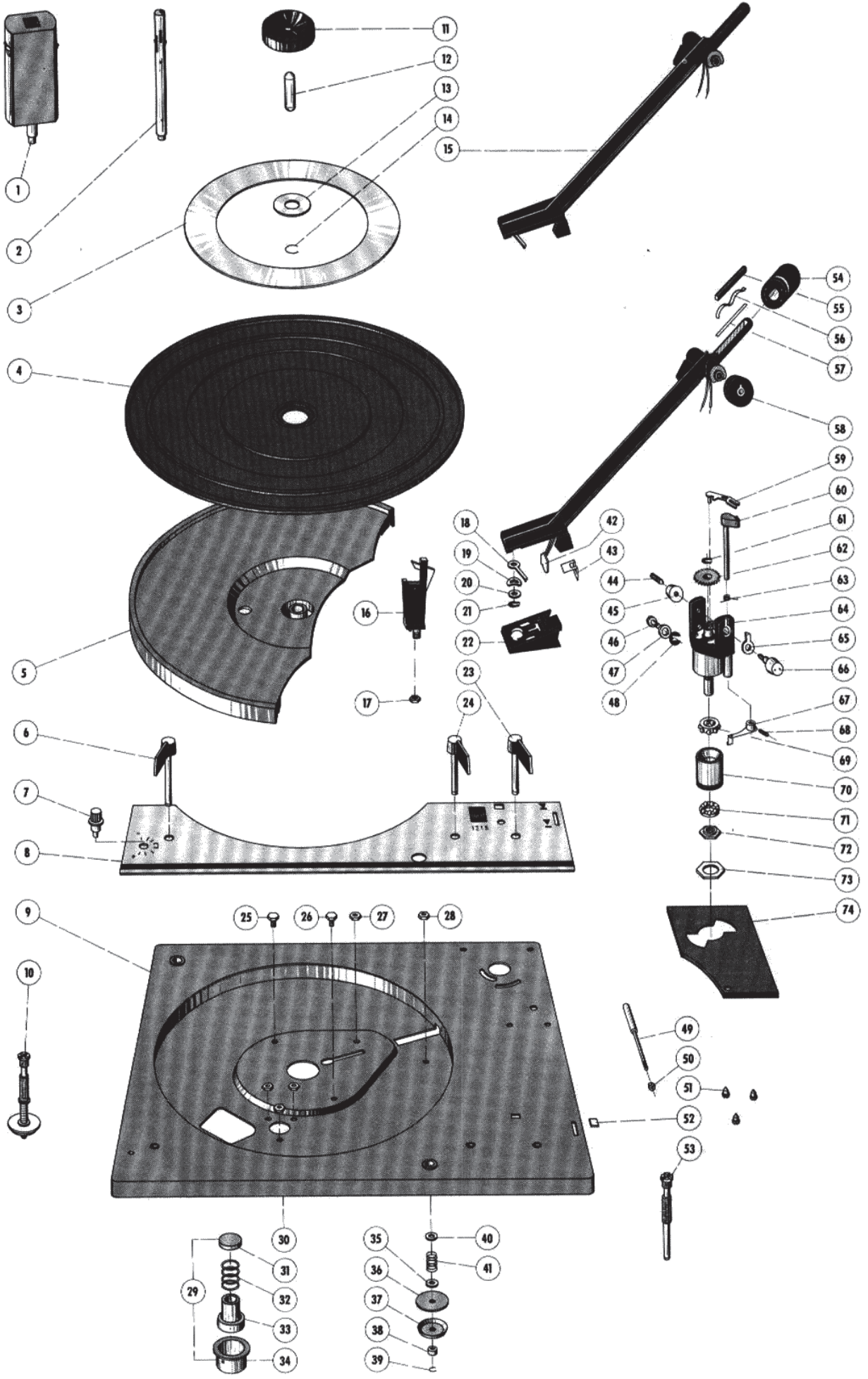
Fig. 24 Exploded view, parts above chassis
