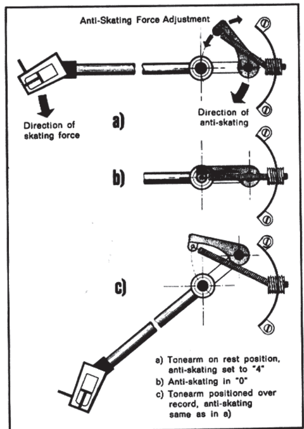
Fig. 9 Anti-skating
