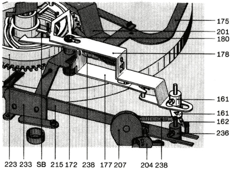
Fig. 13 Stop position
