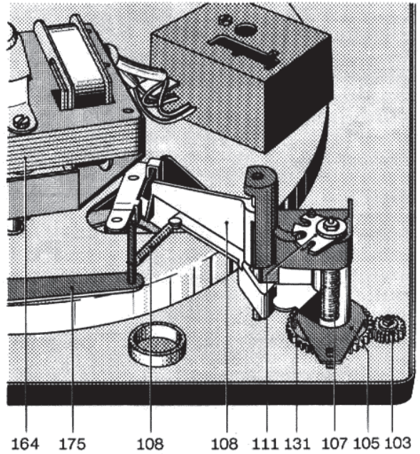
Fig. 5 Turntable speeds and drive wheel shift mechanism
