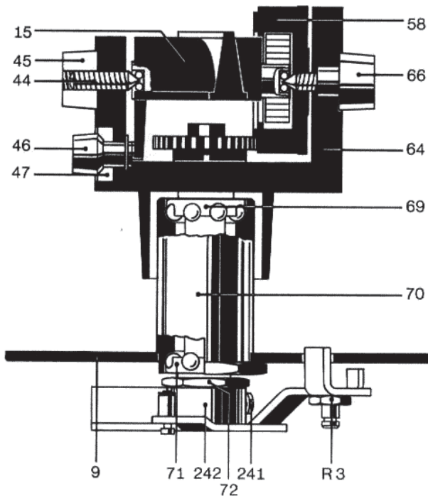
Fig. 7 Tonearm bearing assembly
