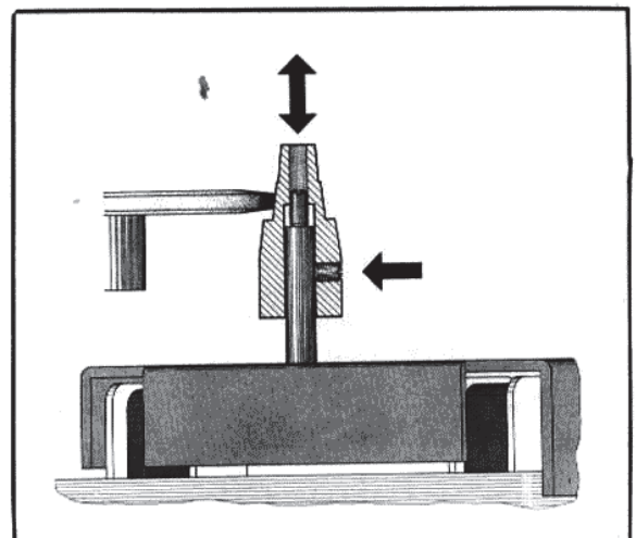
Fig. 6 Motor pulley position
