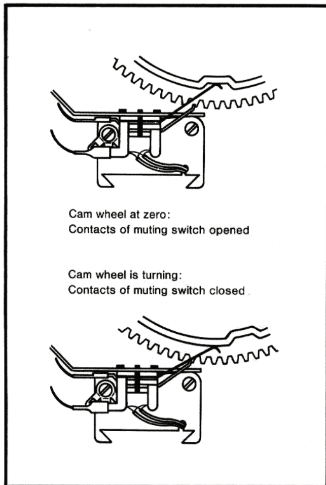
Fig. 14 Muting switch
