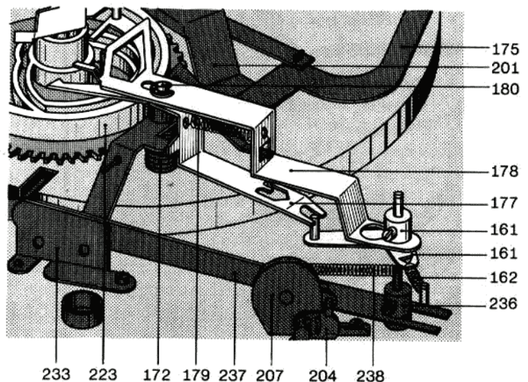
Fig. 12 Start position
