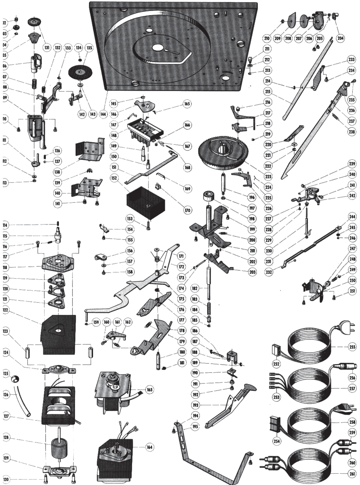
Fig. 25 Exploded view, parts below chassis
