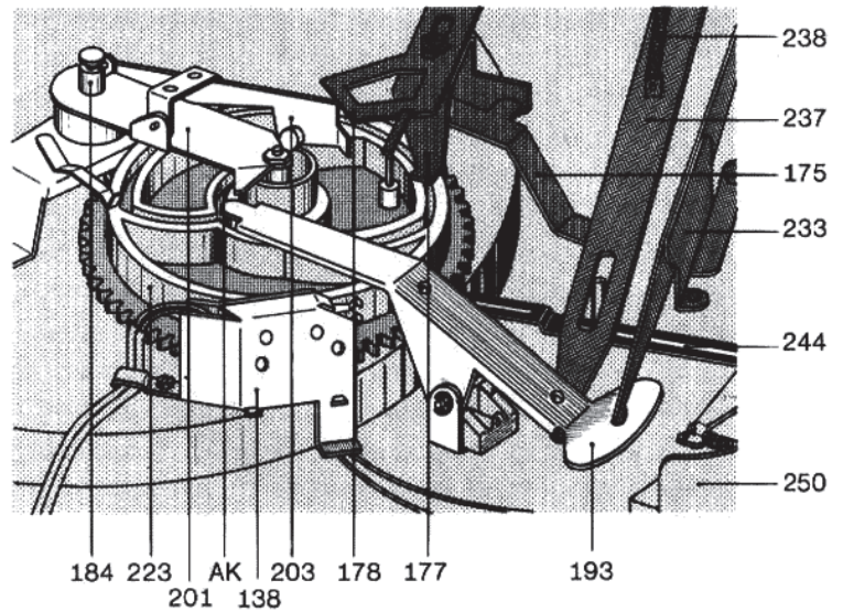
Fig. 15 Record drop
