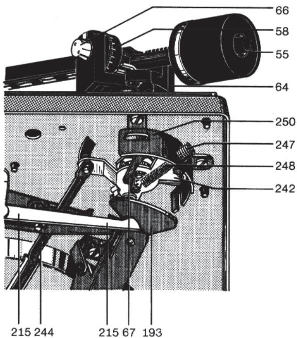
Fig. 8 Tonearm bearing assembly (under view)
