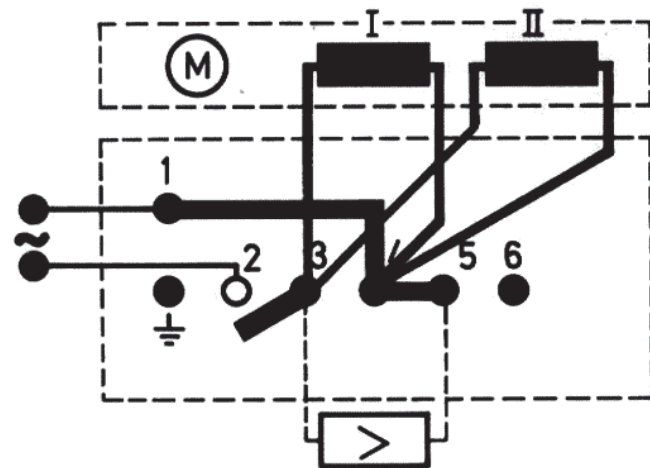
Fig. 3 Motor field connections (less voltage selector)
