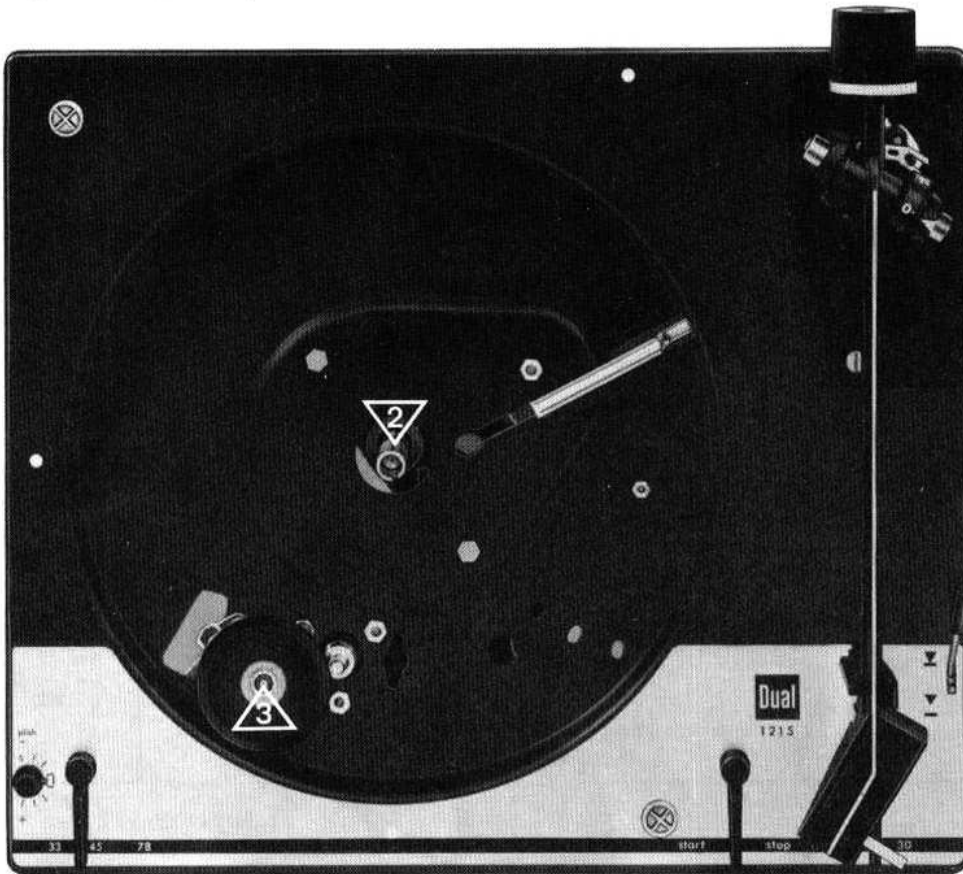
Fig. 26 Chassis, viewed from above
