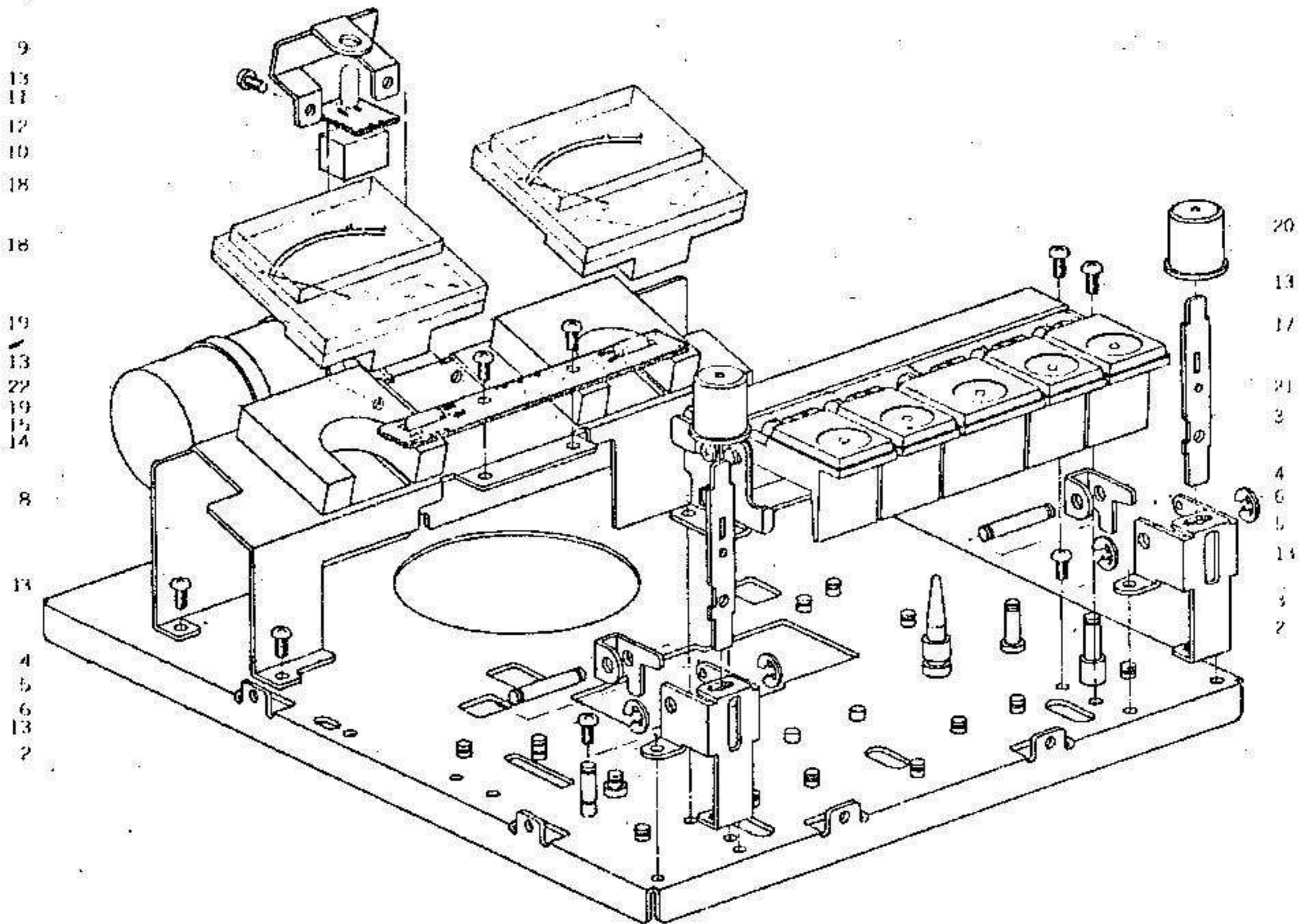
FIG. 4 ILLUSTRATION OF OPERATION BUTTON/METER BASE BLOCK
