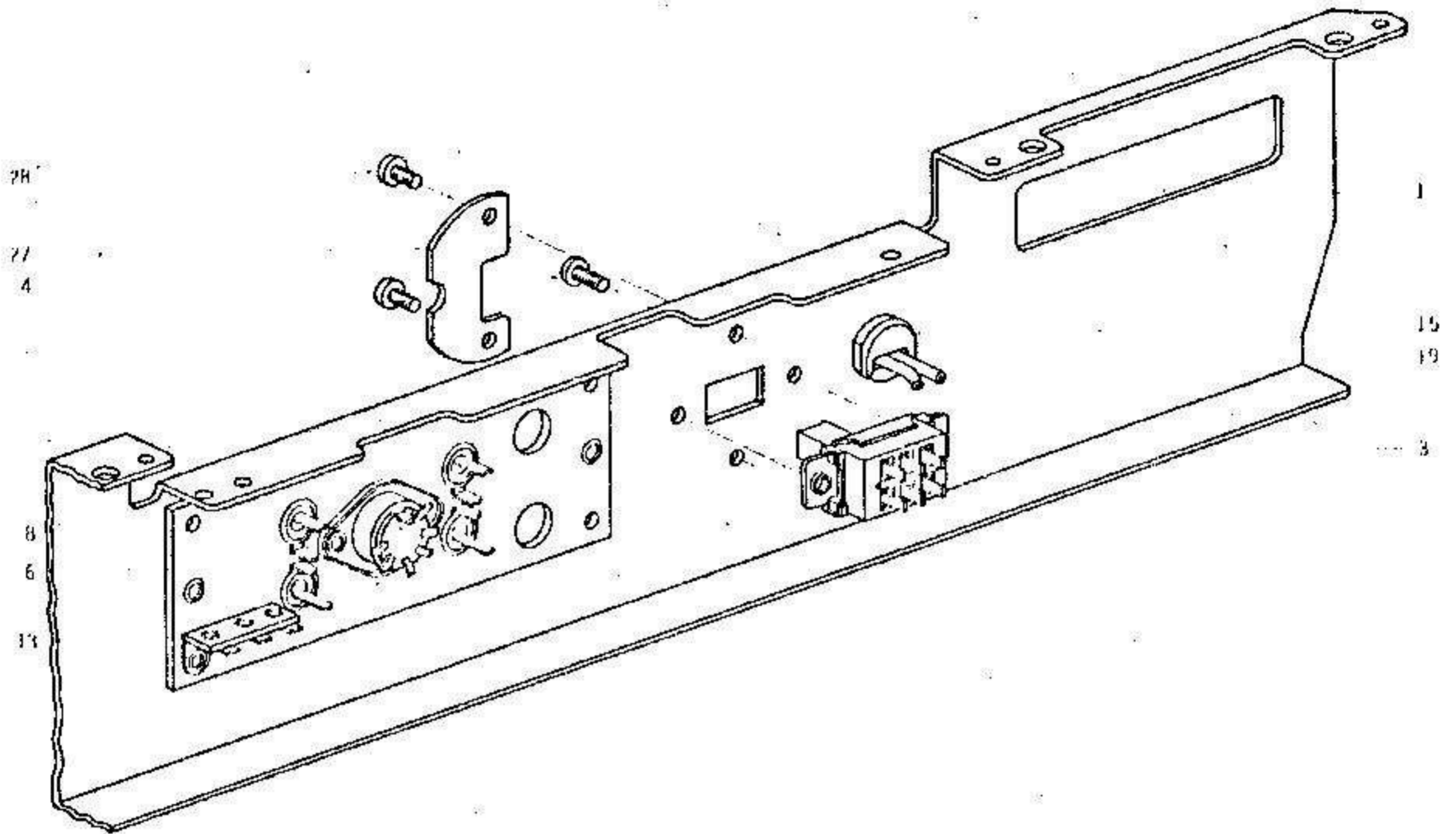
FIG. 11 ILLUSTRATION OF REAR CHASSIS BLOCK
