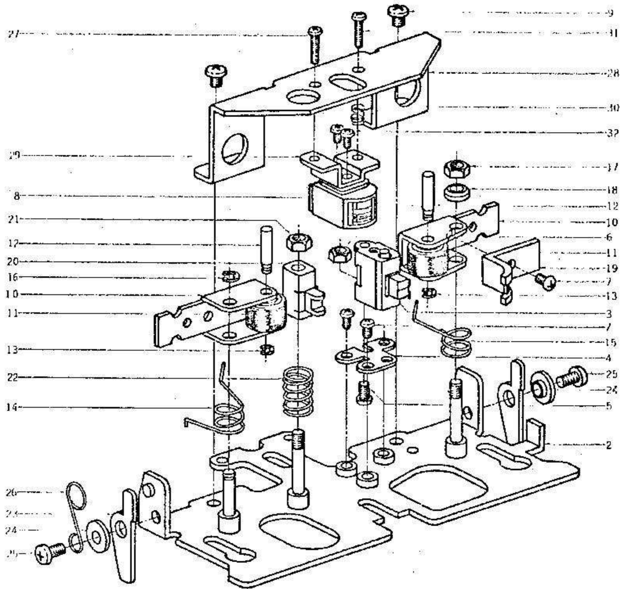
FIG. 1 ILLUSTRATION OF HEAD BLOCK
