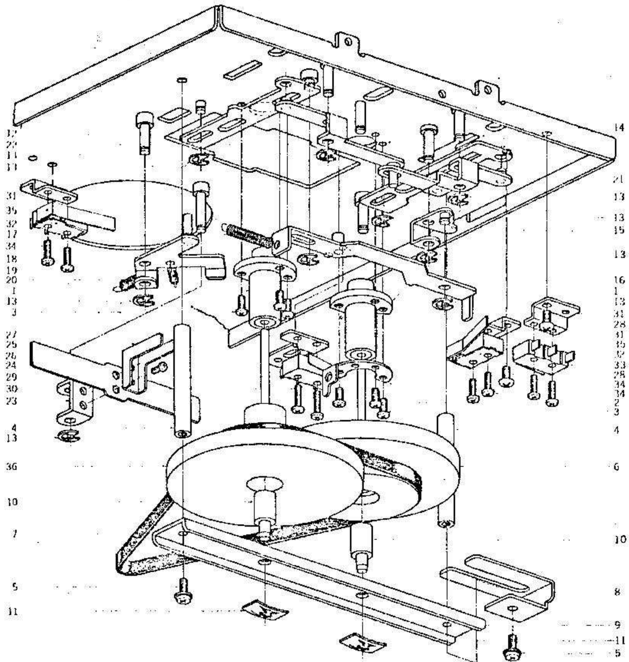
FIG. 7 ILLUSTRATION OF MECH. FRAME BLOCK (2)
