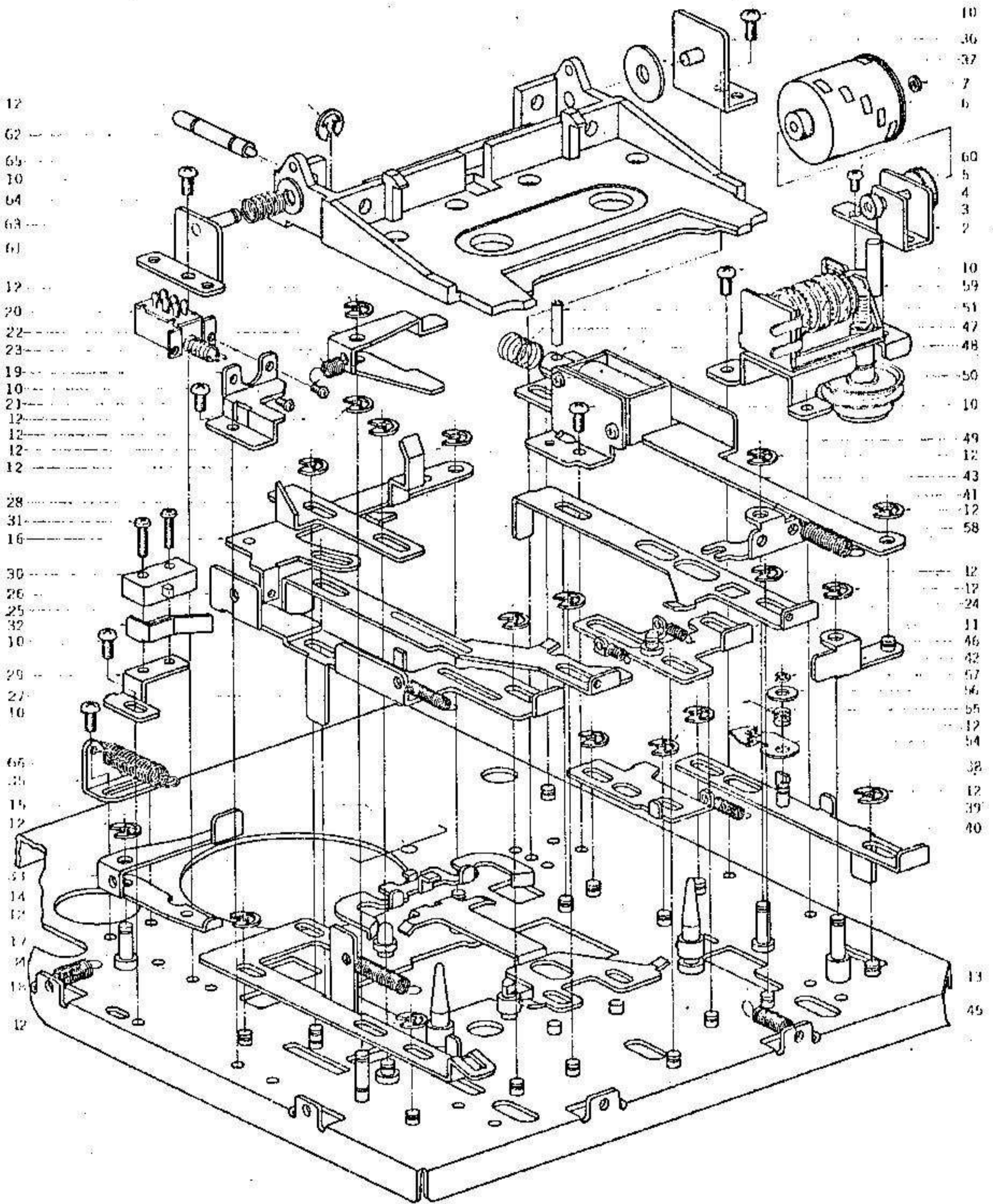
FIG. 6 ILLUSTRATION OF MECH. FRAME BLOCK (1)
