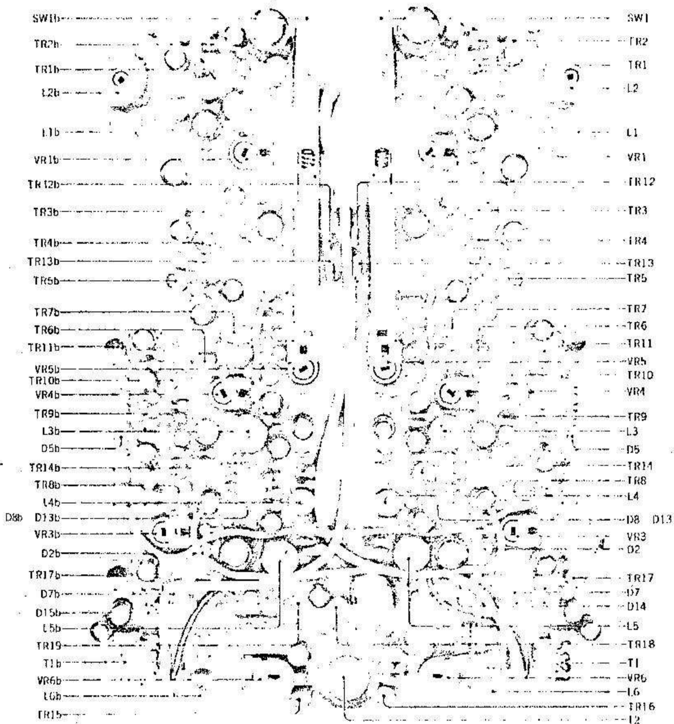
FIG. 8 PHOTO OF PRE-AMP. P.C. BOARD (CW-5214) BLOCK
