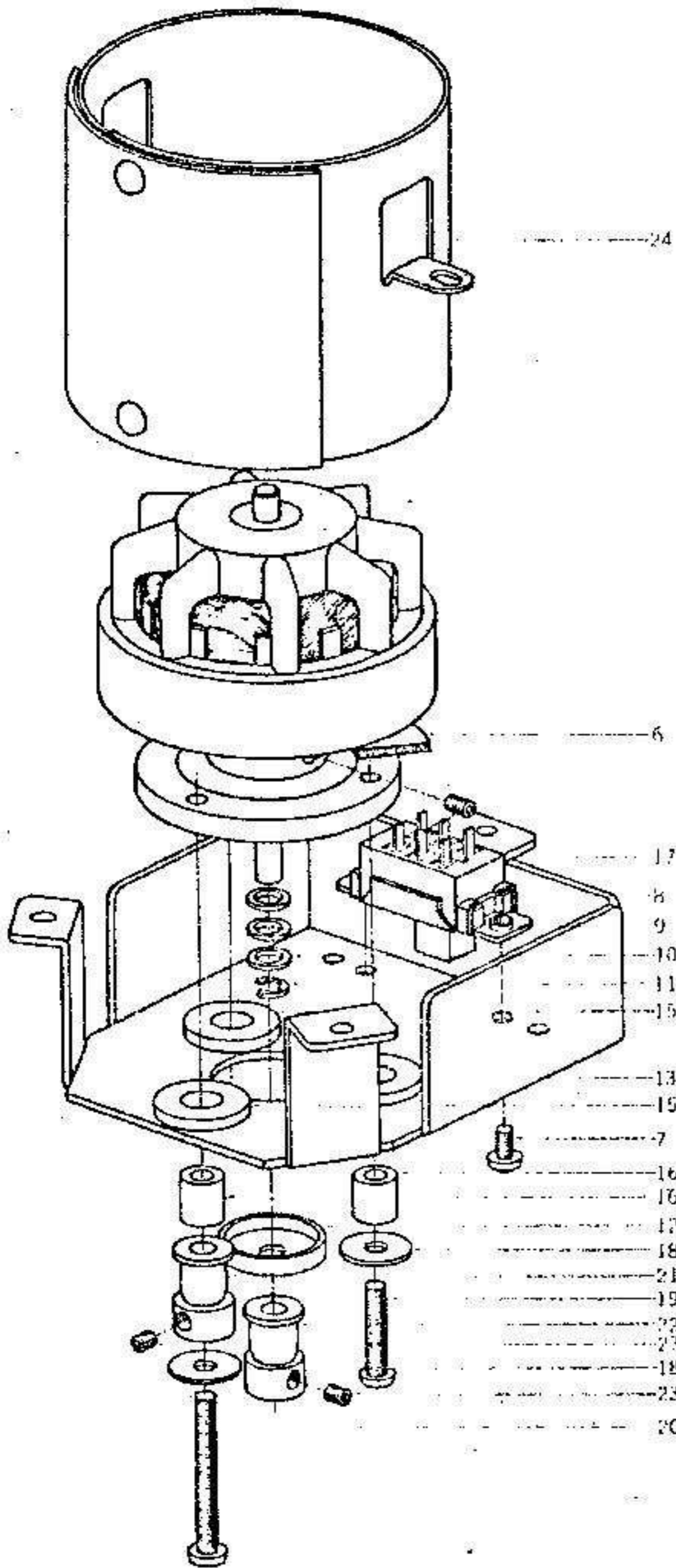
FIG. 2 ILLUSTRATION OF MOTOR BLOCK
