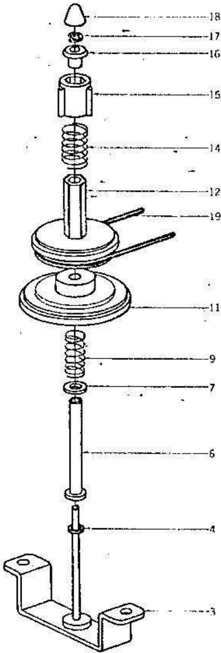
FIG. 3 ILLUSTRATION OF REEL TABLE BLOCK
