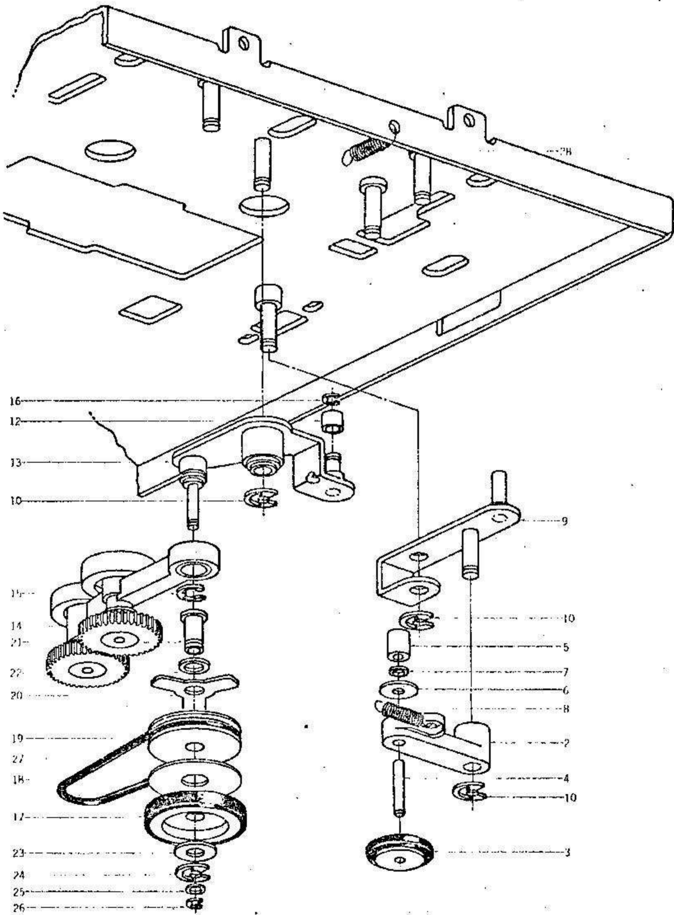
FIG. 5 ILLUSTRATION OF TAKE-UP LEVER/WIND LEVER BLOCK
