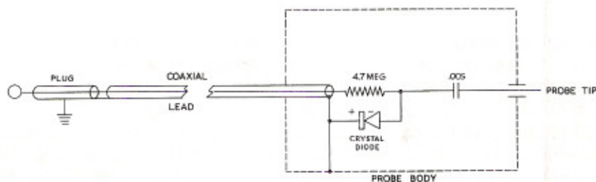
RF PROBE 309-C
