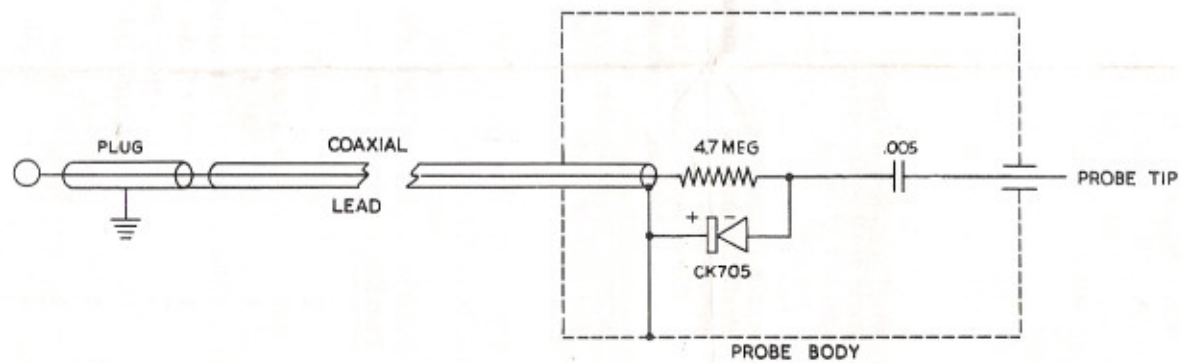
RF PROBE 309-C
