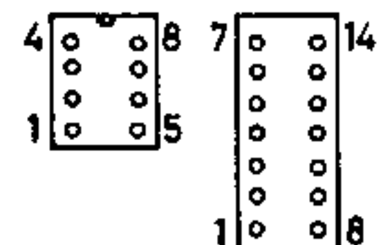
Filter-Anschlüsse (von unten) F-TRANSF. CONNECTIONS (from below)
