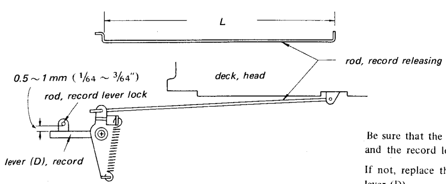
Fig. 11-27 Record releasing rod adjustment
