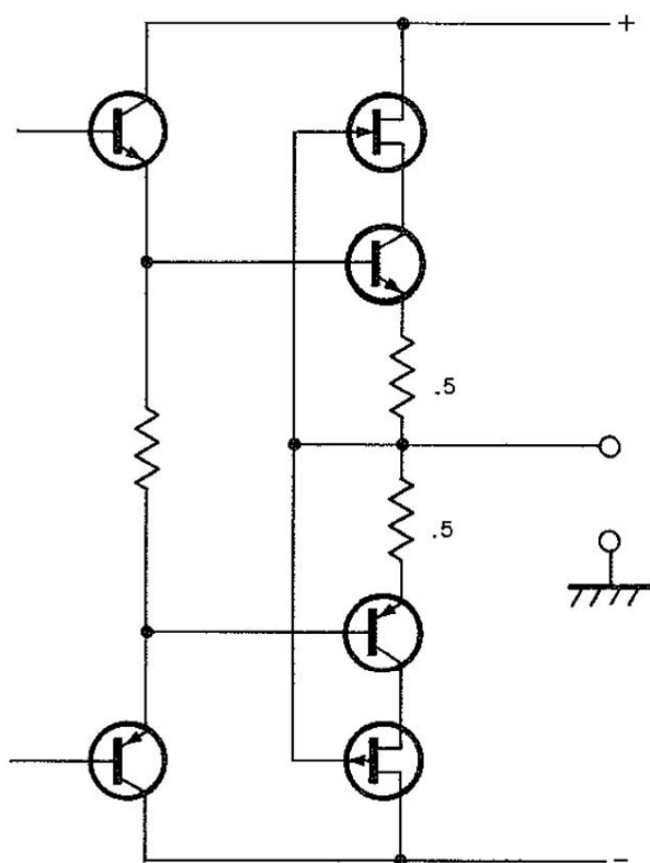
Fig. 4. TA-N7B Simplified Schematic of Power-Output Stage
