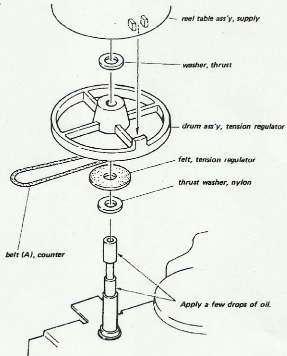
Fig. 2 Tension regulator drum installation
