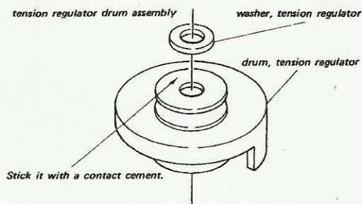
Fig. 1 Tension regulator drum assembly
