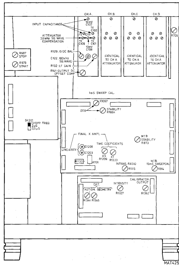
Fig. 3.47. Adjustment points, bottom view
