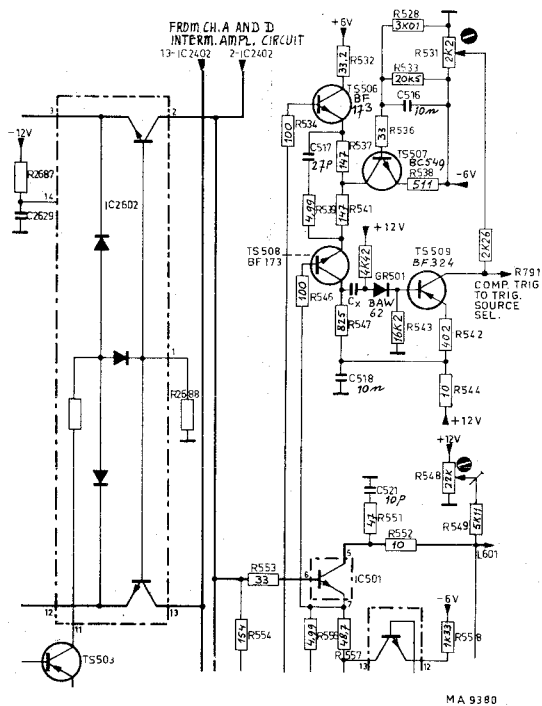
Fig. 3.8. Modified circuit for A.C. composite triggering
