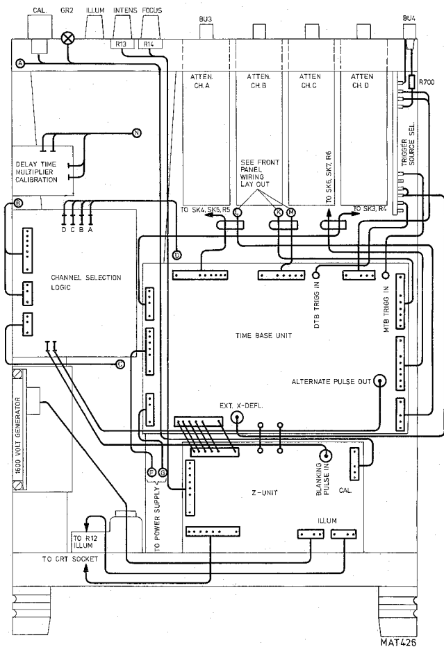
Fig. 3.48. Cable lay-out, bottom view
