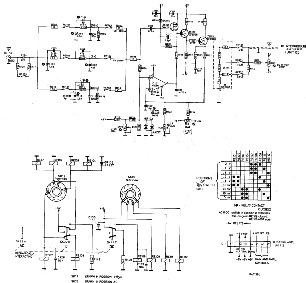
Fig. 3.17. Y-attenuator diagram (unit2)
