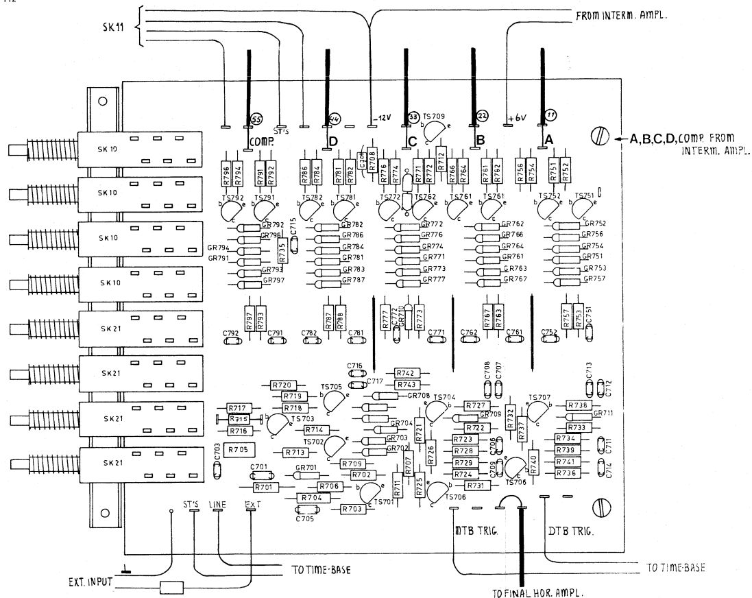
Fig. 3.15. Components lay-out, trigger source selector
