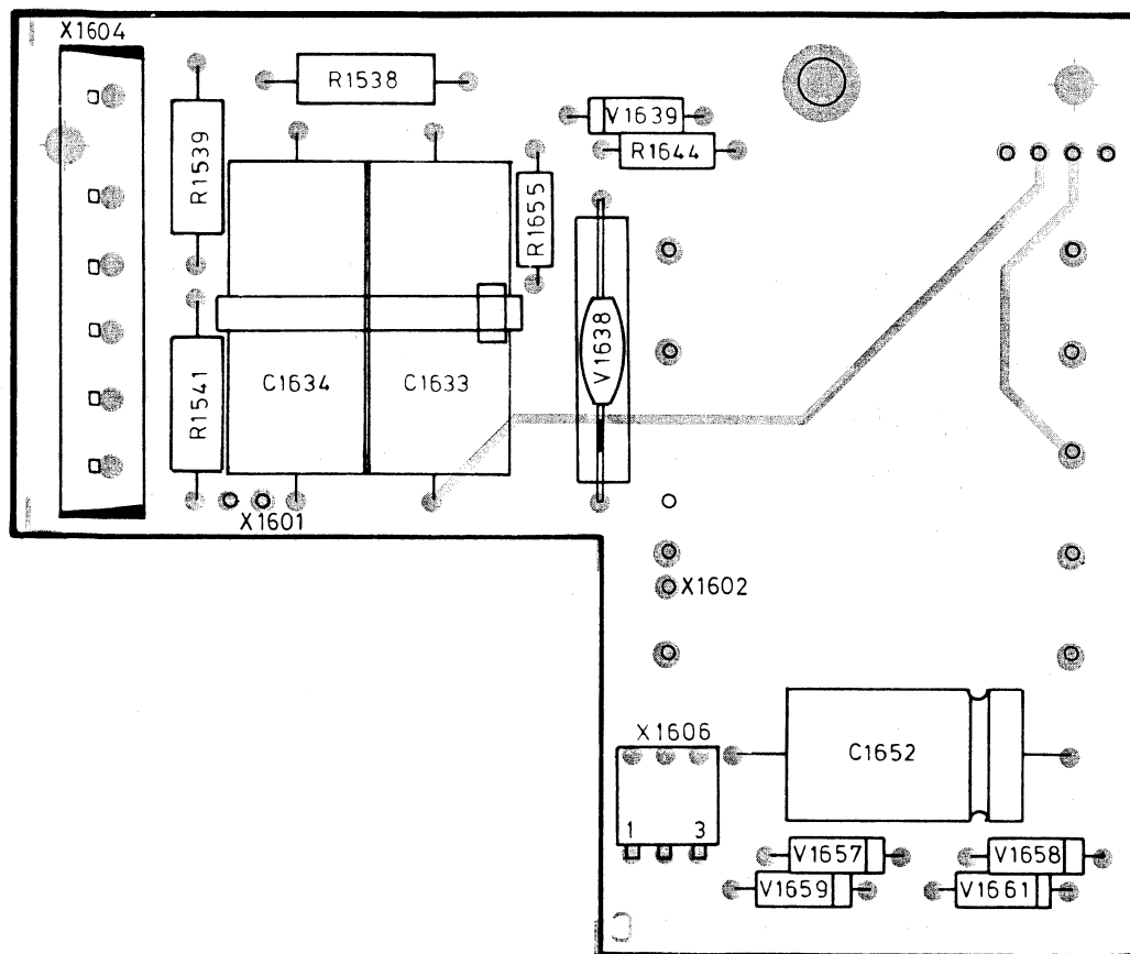
Fig. 8.13. Focus Unit
