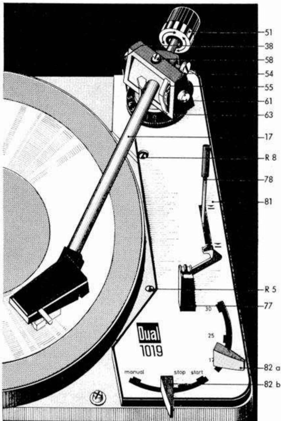
Fig. 12 Operating elements
