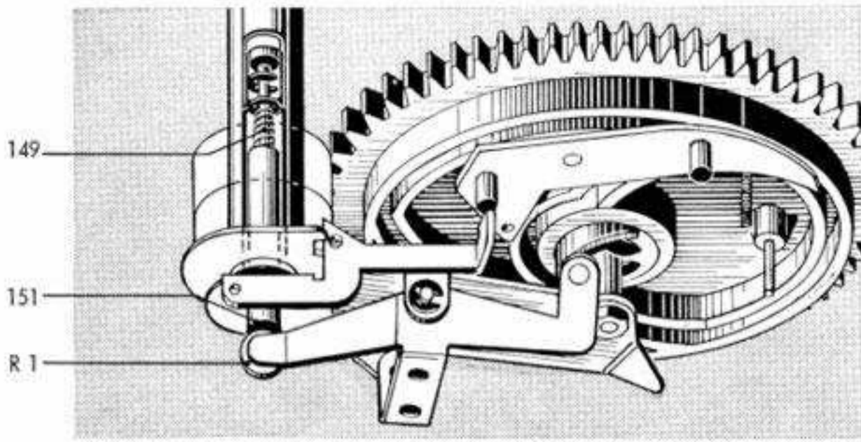
Fig. 16 Changing action
