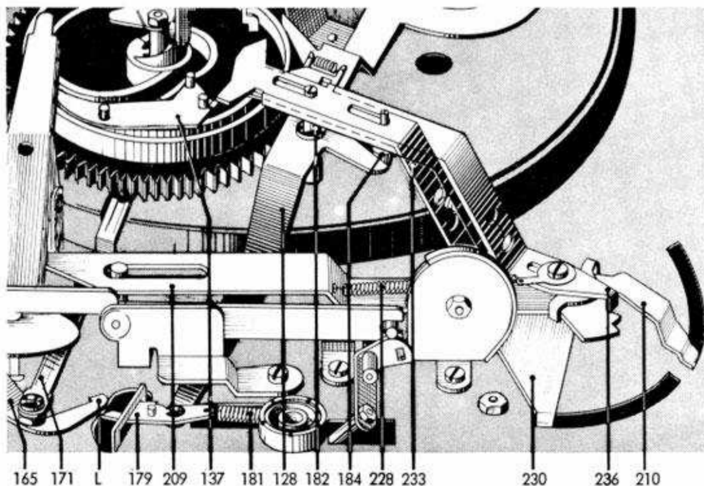
Fig. 13 Start position
