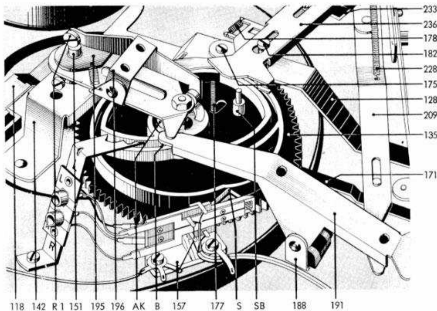
Fig. 15 Record drop
