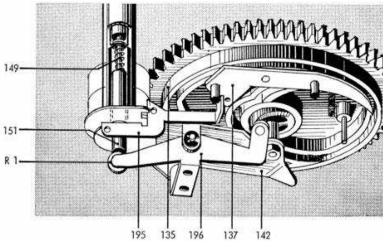
Fig. 18 First stage of change or shut-off action
