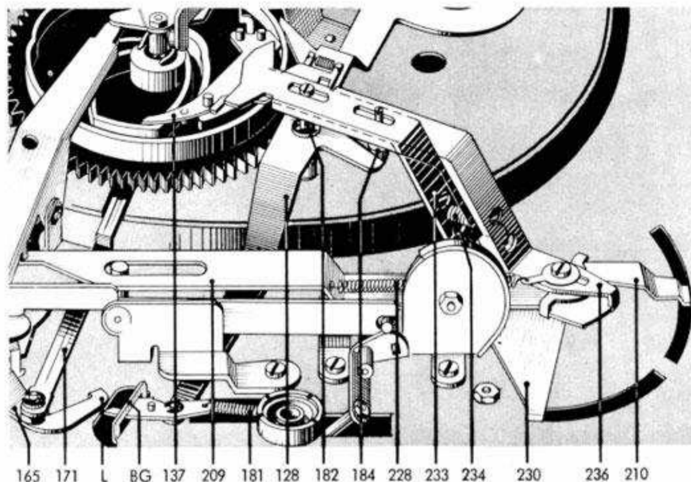
Fig. 14 Stop action
