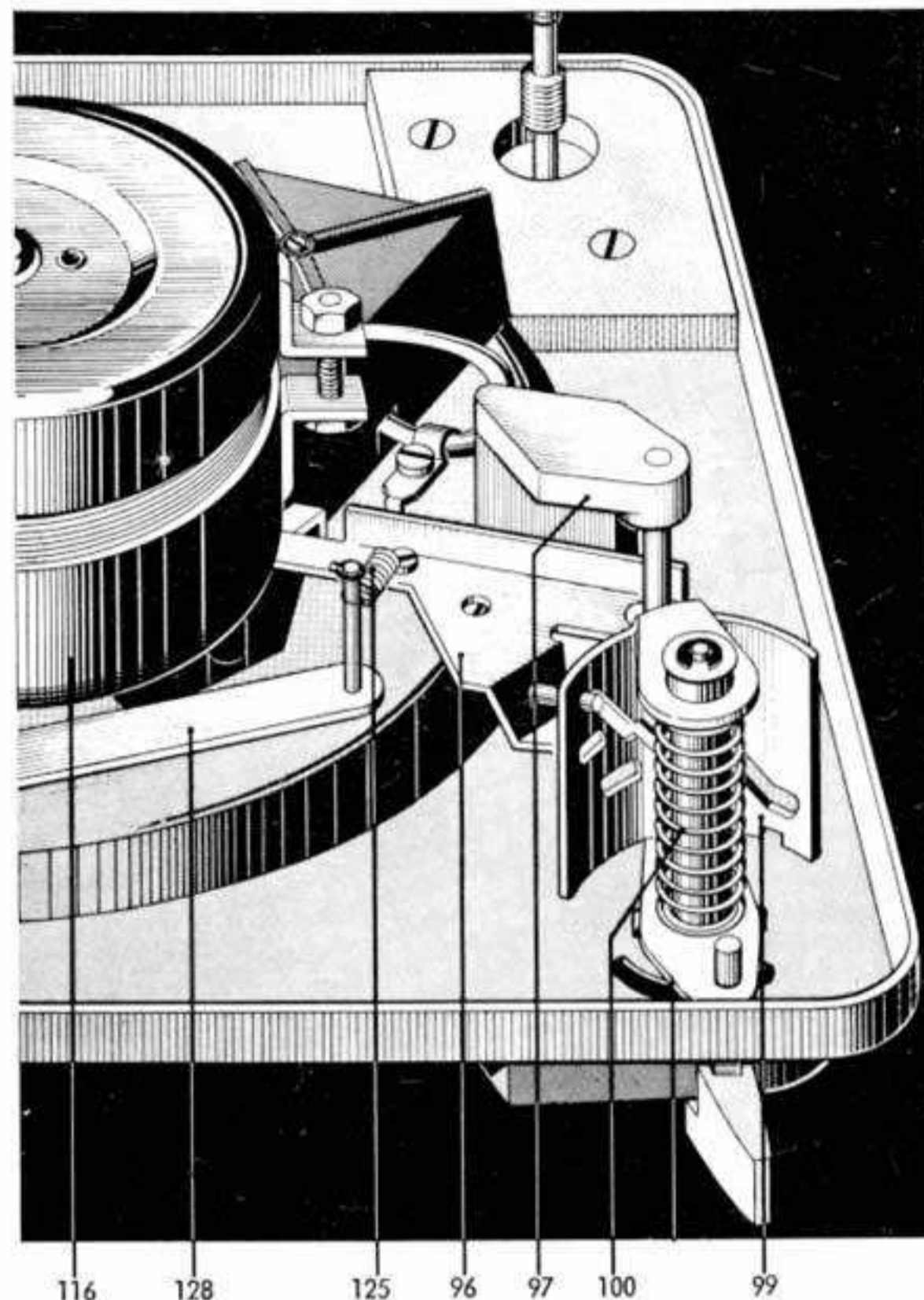
Fig. 4 Turntable speeds and drive wheel shift mechanism
